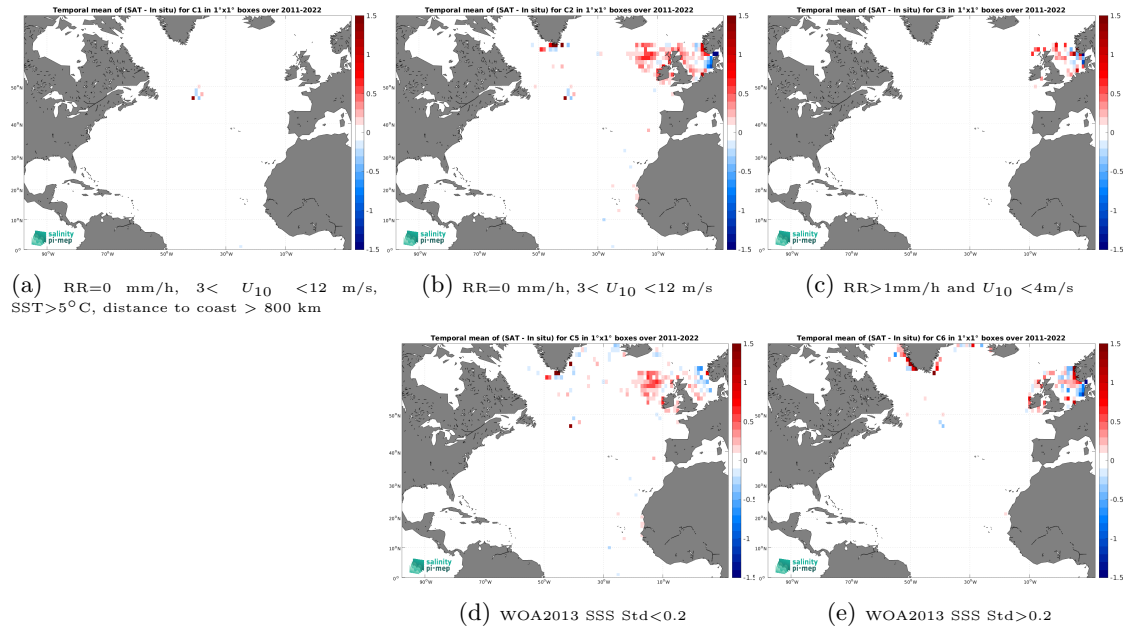
Figure 12: Temporal mean gridded over spatial boxes of size 1^\circ \times 1^\circ of \Delta\text{SSS} (SMAP SSS L4 OI v2 - Monthly (IPRC) - ICES) for 5 different subdatasets corresponding to:RR=0 mm/h, 3 < U_{10} < 12 m/s, SST >5^\circ\text{C} , distance to coast > 800 km (a), RR=0 mm/h, 3 < U_{10} < 12 m/s (b), RR >1 mm/h and U_{10} < 4 m/s (c), WOA2013 SSS Std <0.2 (d), WOA2013 SSS Std >0.2 (e).
