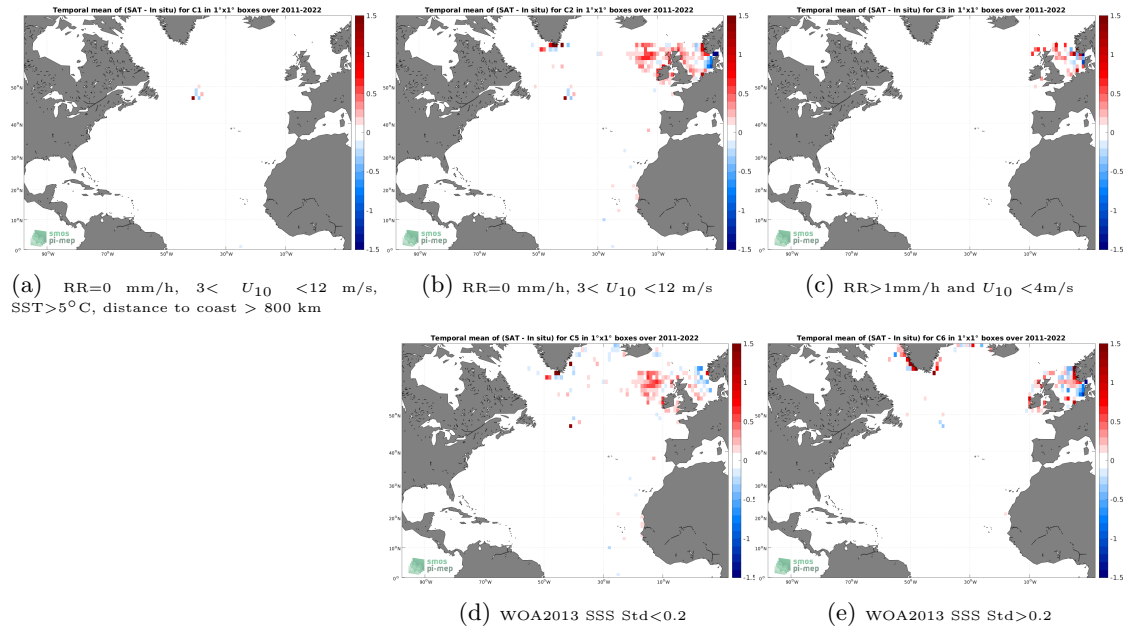
Figure 12: Temporal mean gridded over spatial boxes of size 1^\circ \times 1^\circ of \Delta SSS (SMAP SSS L4 OI v2 - Monthly (IPRC) - ICES) for 5 different subdatasets corresponding to:RR=0 mm/h, 3 < U_{10} < 12 m/s, SST >5^\circ\text{C} , distance to coast > 800 km (a), RR=0 mm/h, 3 < U_{10} < 12 m/s (b), RR >1 mm/h and U_{10} < 4 m/s (c), WOA2013 SSS Std <0.2 (d), WOA2013 SSS Std >0.2 (e).
