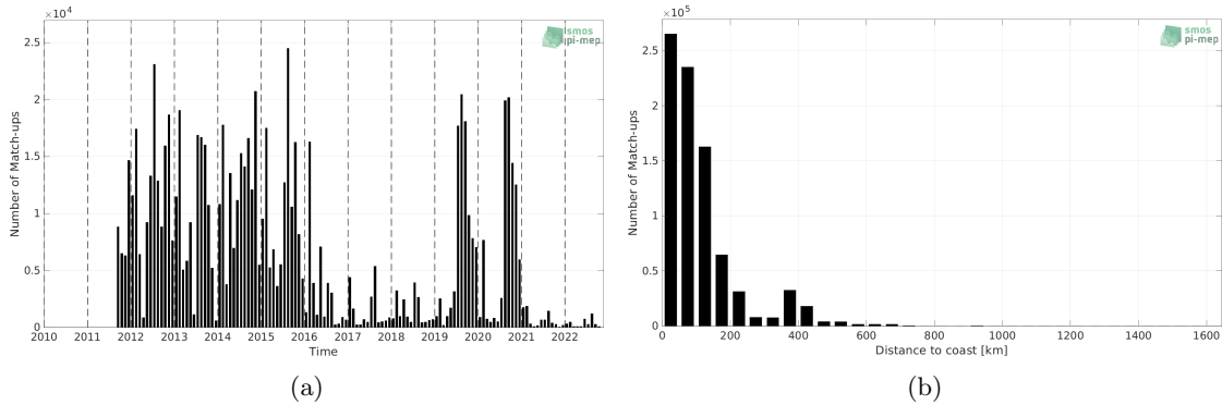
Figure 1: Number of match-ups between ICES and SMAP SSS L4 OI v2 - Monthly (IPRC) SSS as a function of time (a) and as function of the distance to coast (b) over the North Atlantic Ocean Pi-MEP region and for the full satellite product period.
