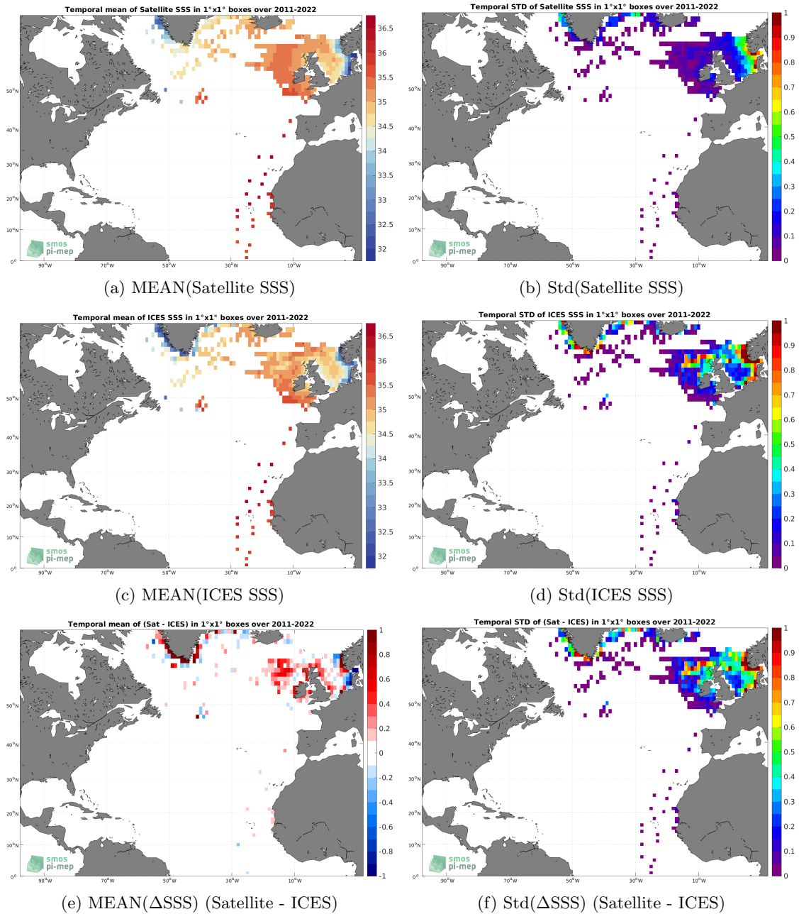
Figure 6: Temporal mean (left) and Std (right) of SSS from SMAP SSS L4 OI v2 - Monthly (IPRC) (top), ICES (middle), and of \Delta SSS (Satellite - ICES). Only match-up pairs are used to generate these maps.
