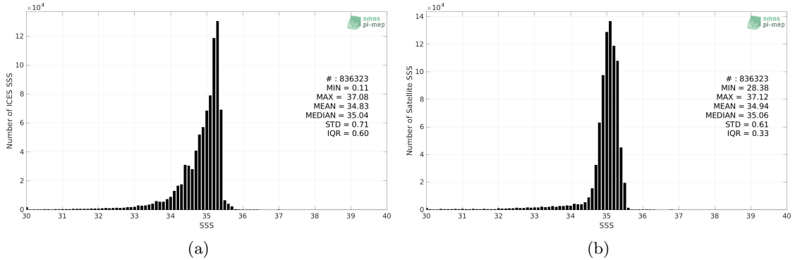
Figure 2: Histograms of SSS from ICES (a) and SMAP SSS L4 OI v2 - Monthly (IPRC) (b) considering all match-up pairs per bins of 0.1 over the North Atlantic Ocean Pi-MEP region and for the full satellite product period.
