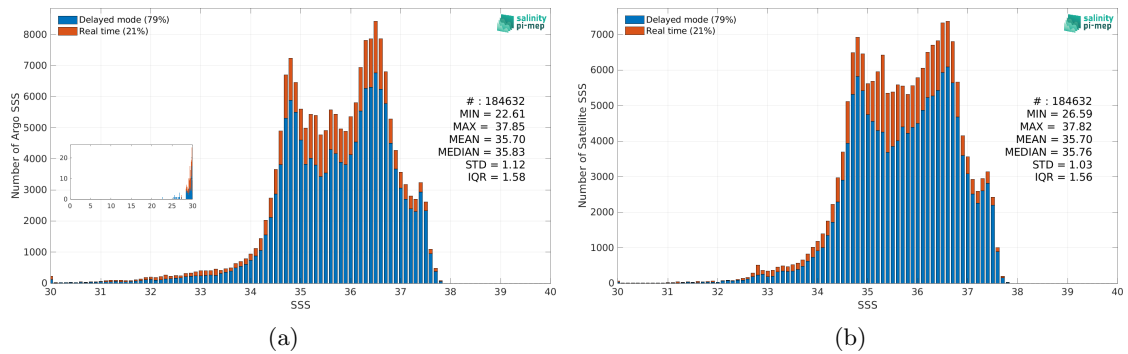
Figure 2: Histograms of SSS from Argo (a) and SMAP SSS L4 OI v2 - Monthly (IPRC) (b) considering all match-up pairs per bins of 0.1 over the North Atlantic Ocean Pi-MEP region and for the full satellite product period.
