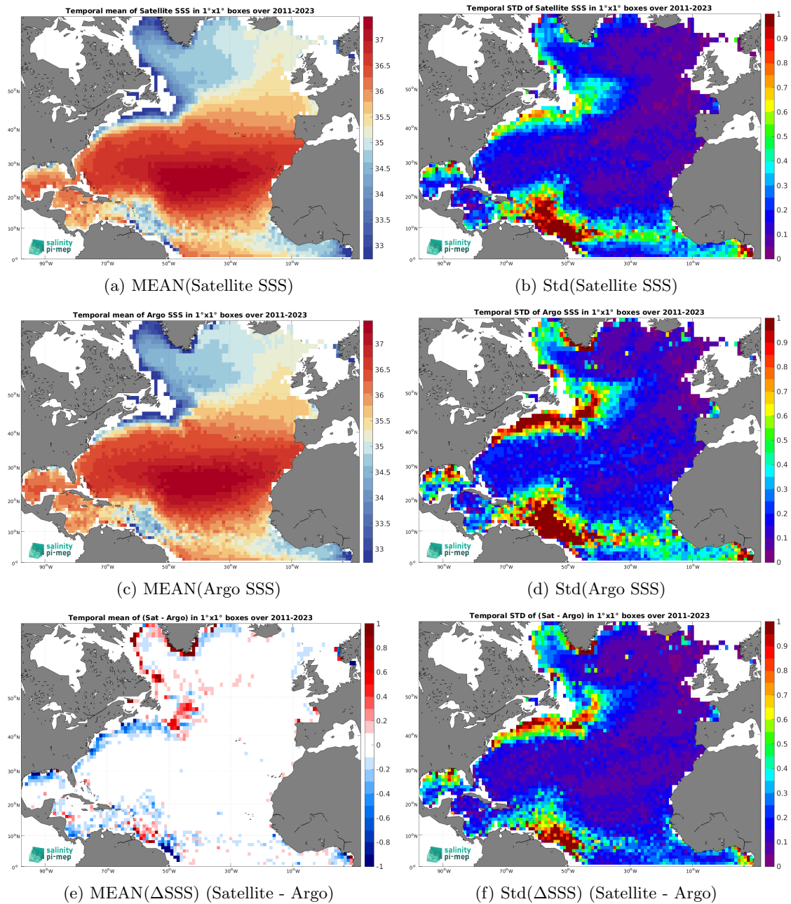
Figure 6: Temporal mean (left) and Std (right) of SSS from SMAP SSS L4 OI v2 - Monthly (IPRC) (top), Argo (middle), and of \Delta SSS (Satellite - Argo). Only match-up pairs are used to generate these maps.
