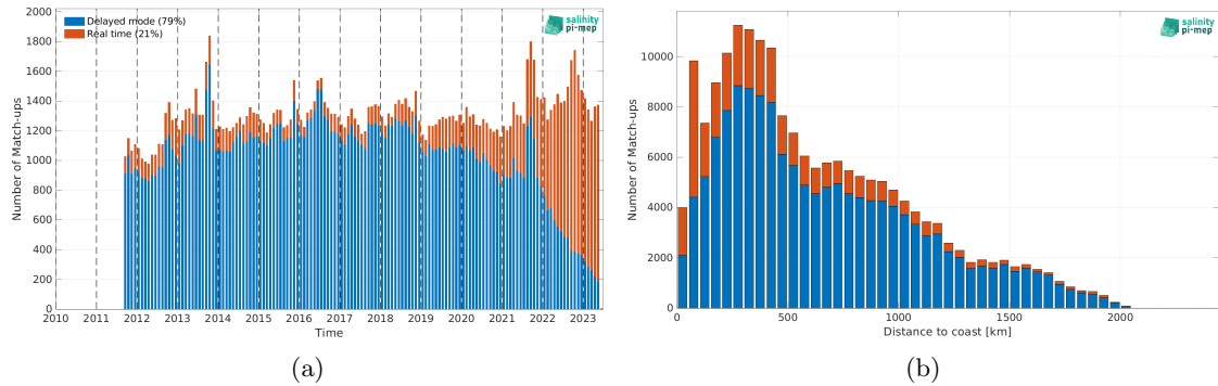
Figure 1: Number of match-ups between Argo and SMAP SSS L4 OI v2 - Monthly (IPRC) SSS as a function of time (a) and as function of the distance to coast (b) over the North Atlantic Ocean Pi-MEP region and for the full satellite product period.
