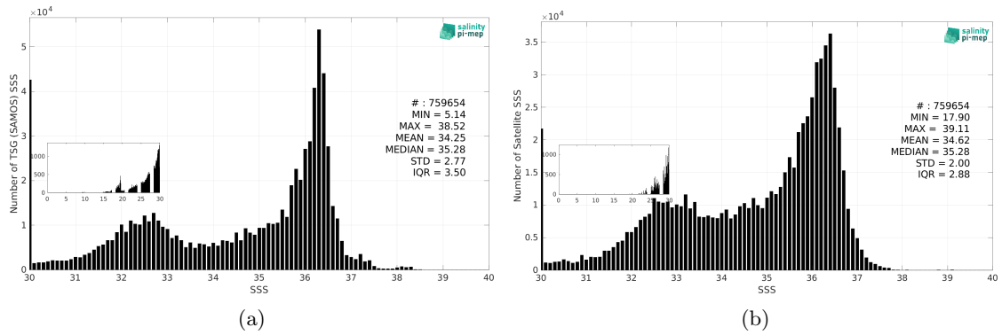
Figure 3: Histograms of SSS from TSG (SAMOS) (a) and SMAP SSS L3 v6 - 8-Day running (RSS) (b) considering all match-up pairs per bins of 0.1 over the North Atlantic Ocean Pi-MEP region and for the full satellite product period.
