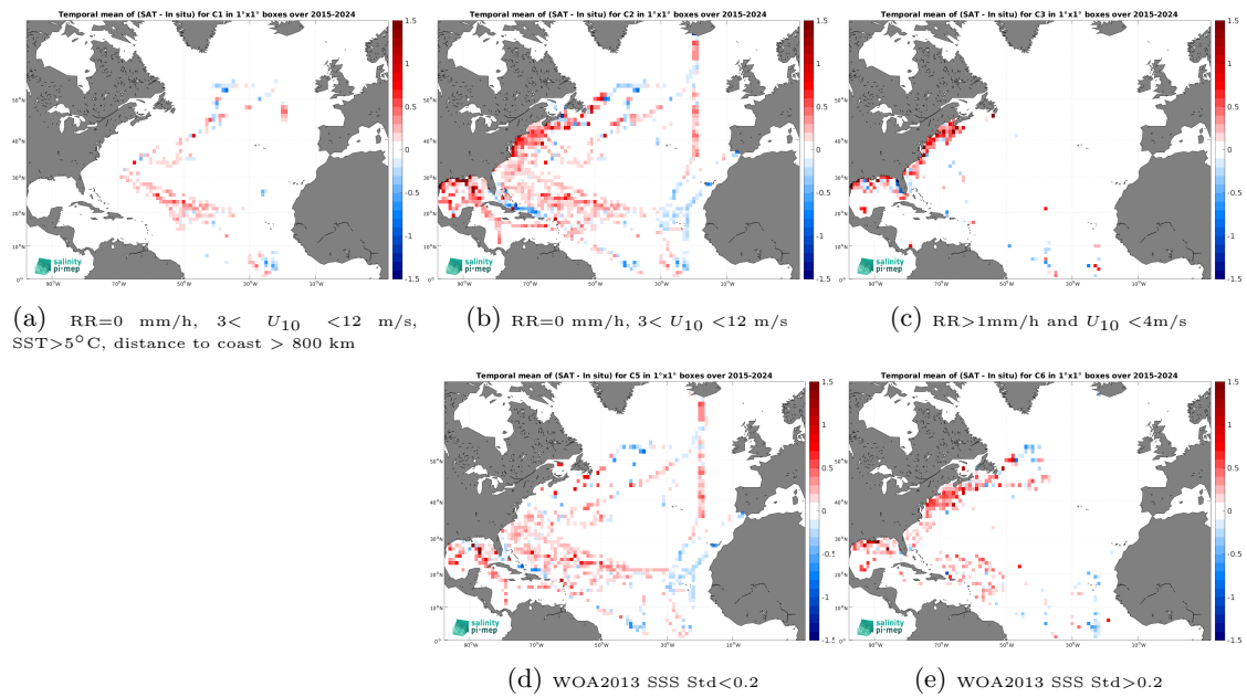
Figure 14: Temporal mean gridded over spatial boxes of size 1^\circ \times 1^\circ of \Delta\text{SSS} (SMAP SSS L3 v6 - 8-Day running (RSS) - TSG (SAMOS)) for 5 different subdatasets corresponding to:RR=0 mm/h, 3 < U_{10} < 12 m/s, SST > 5^\circ\text{C} , distance to coast > 800 km (a), RR=0 mm/h, 3 < U_{10} < 12 m/s (b), RR > 1 mm/h and U_{10} < 4 m/s (c), WOA2013 SSS Std < 0.2 (d), WOA2013 SSS Std > 0.2 (e).
