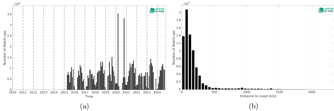
Figure 2: Number of match-ups between TSG (SAMOS) and SMAP SSS L3 v6 - 8-Day running (RSS) SSS as a function of time (a) and as function of the distance to coast (b) over the North Atlantic Ocean Pi-MEP region and for the full satellite product period.
