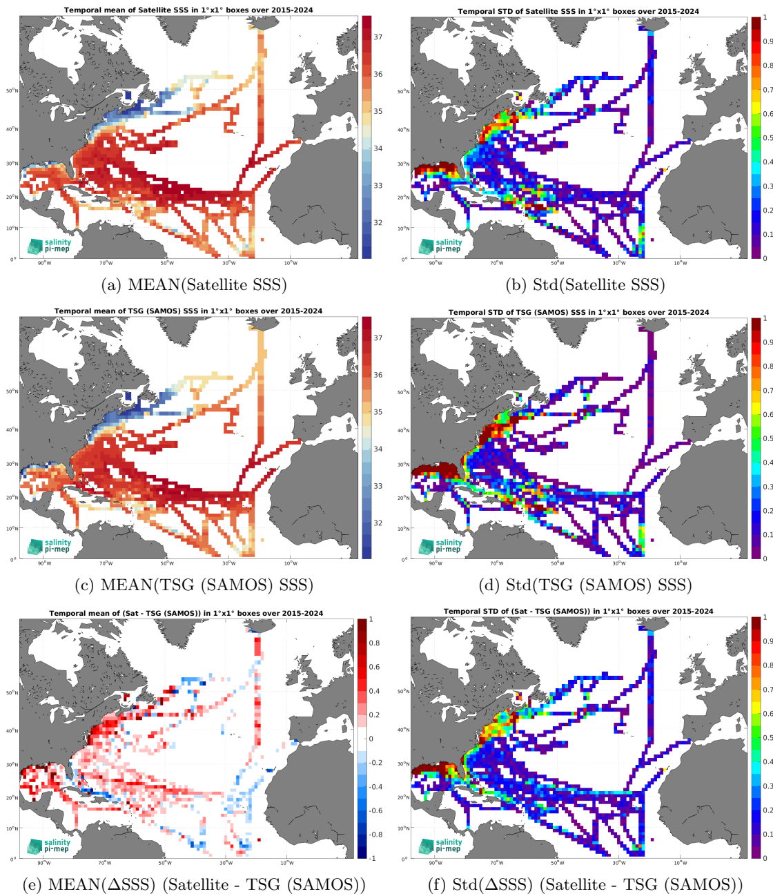
Figure 7: Temporal mean (left) and Std (right) of SSS from SMAP SSS L3 v6 - 8-Day running (RSS) (top), TSG (SAMOS) (middle), and of \Delta SSS (Satellite - TSG (SAMOS)). Only match-up pairs are used to generate these maps.
