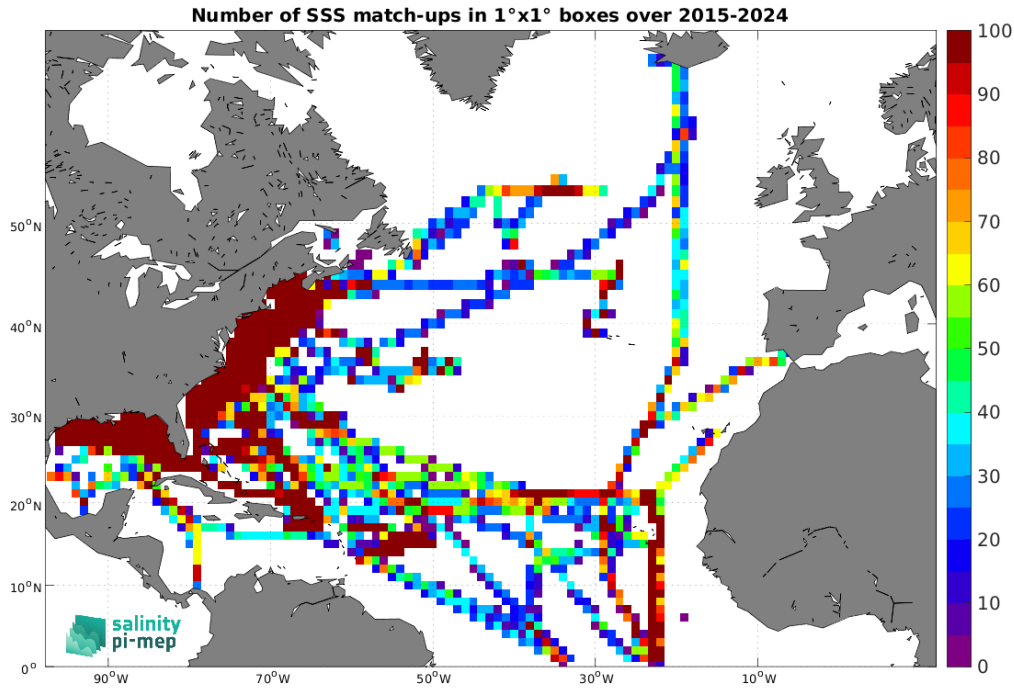
Figure 5: Number of SSS match-ups between TSG (SAMOS) SSS and the SMAP SSS L3 v6 - 8-Day running (RSS) SSS product for the North Atlantic Ocean Pi-MEP region over 1^\circ \times 1^\circ boxes and for the full satellite product period.
