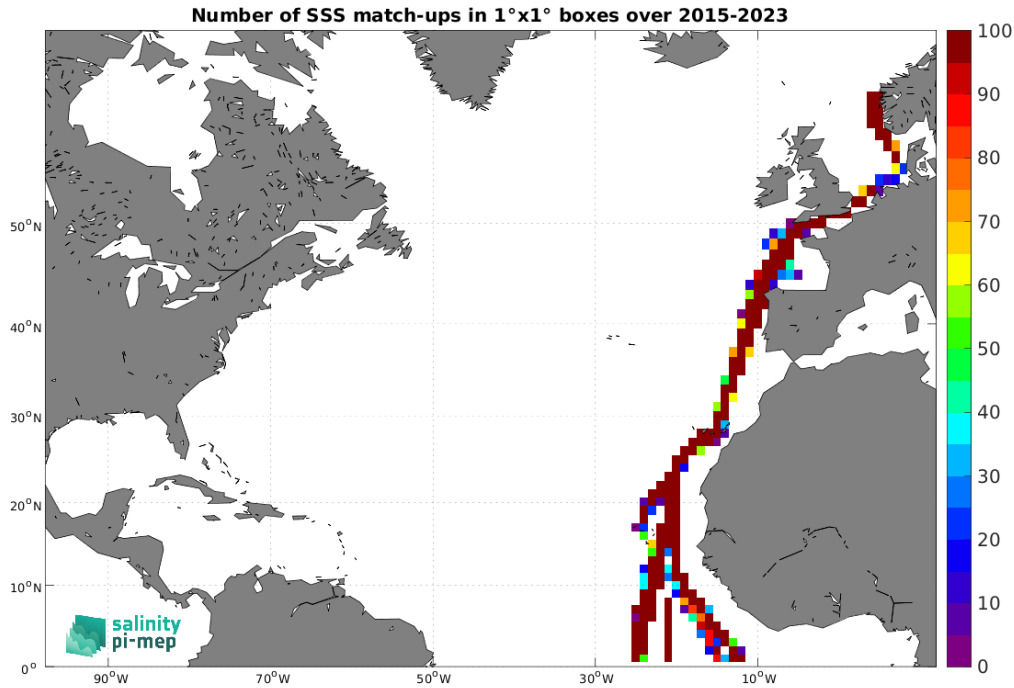
Figure 5: Number of SSS match-ups between TSG (Polarstern) SSS and the SMAP SSS L3 v6 - 8-Day running (RSS) SSS product for the North Atlantic Ocean Pi-MEP region over 1^\circ \times 1^\circ boxes and for the full satellite product period.
