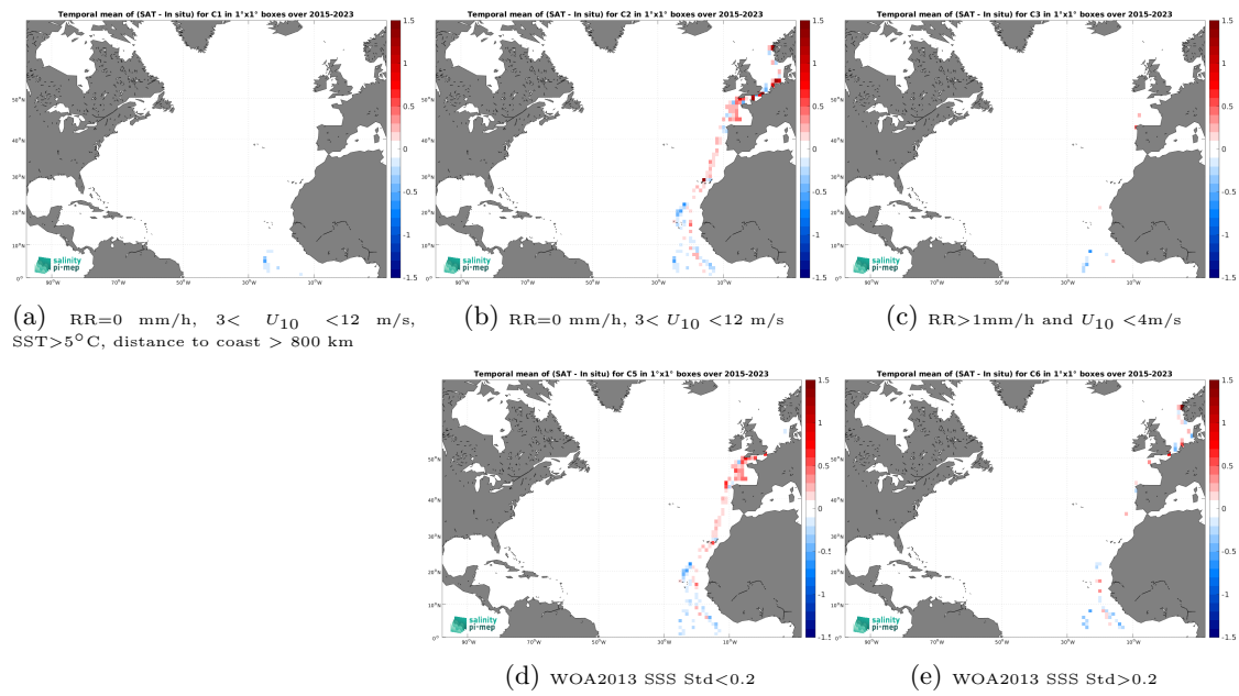
Figure 14: Temporal mean gridded over spatial boxes of size 1^\circ \times 1^\circ of \Delta\text{SSS} (SMAP SSS L3 v6 - 8-Day running (RSS) - TSG (Polarstern)) for 5 different subdatasets corresponding to:RR=0 mm/h, 3 < U_{10} < 12 m/s, SST >5^\circ\text{C} , distance to coast > 800 km (a), RR=0 mm/h, 3 < U_{10} < 12 m/s (b), RR >1 mm/h and U_{10} < 4 m/s (c), WOA2013 SSS Std <0.2 (d), WOA2013 SSS Std >0.2 (e).
