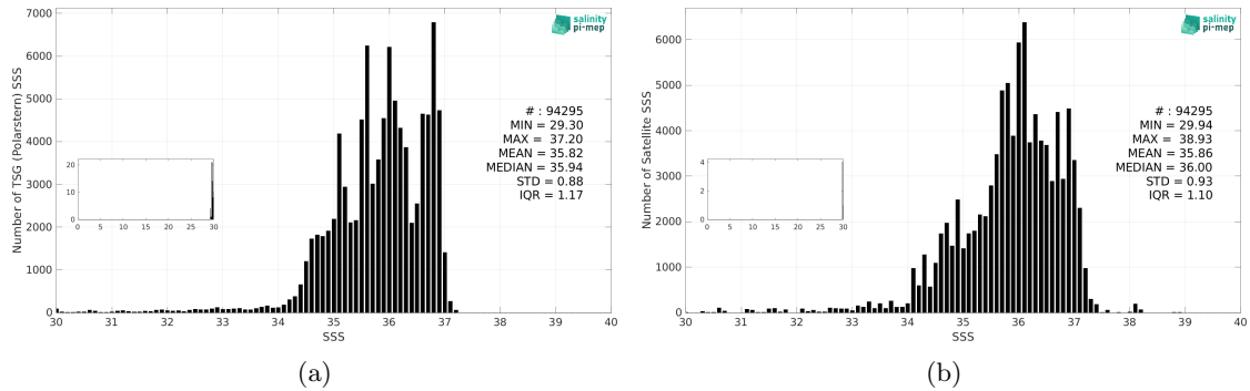
Figure 3: Histograms of SSS from TSG (Polarstern) (a) and SMAP SSS L3 v6 - 8-Day running (RSS) (b) considering all match-up pairs per bins of 0.1 over the North Atlantic Ocean Pi-MEP region and for the full satellite product period.
