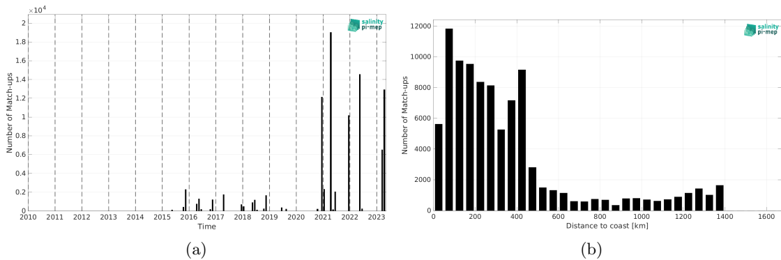
Figure 2: Number of match-ups between TSG (Polarstern) and SMAP SSS L3 v6 - 8-Day running (RSS) SSS as a function of time (a) and as function of the distance to coast (b) over the North Atlantic Ocean Pi-MEP region and for the full satellite product period.
