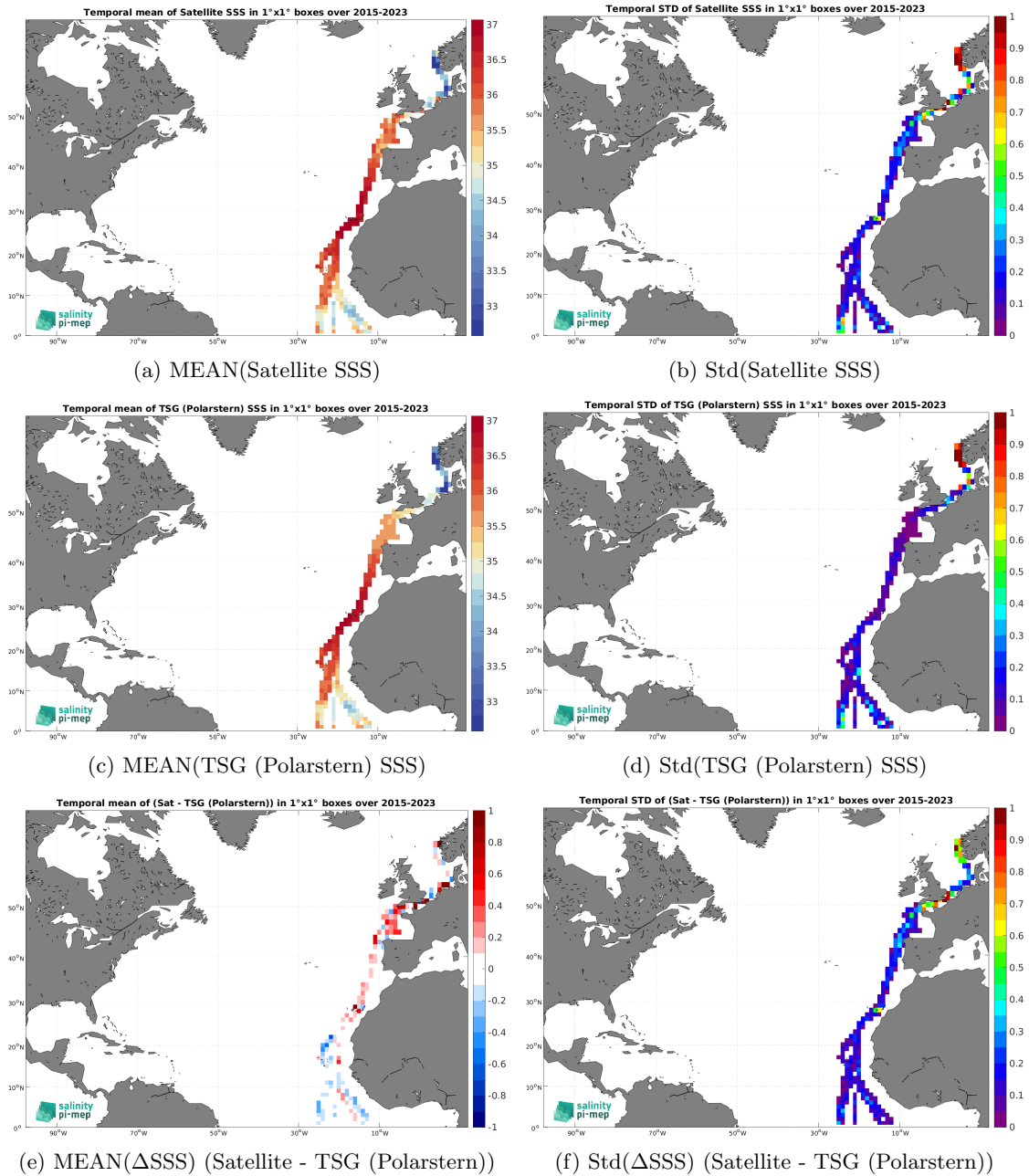
Figure 7: Temporal mean (left) and Std (right) of SSS from SMAP SSS L3 v6 - 8-Day running (RSS) (top), TSG (Polarstern) (middle), and of \Delta SSS (Satellite - TSG (Polarstern)). Only match-up pairs are used to generate these maps.
