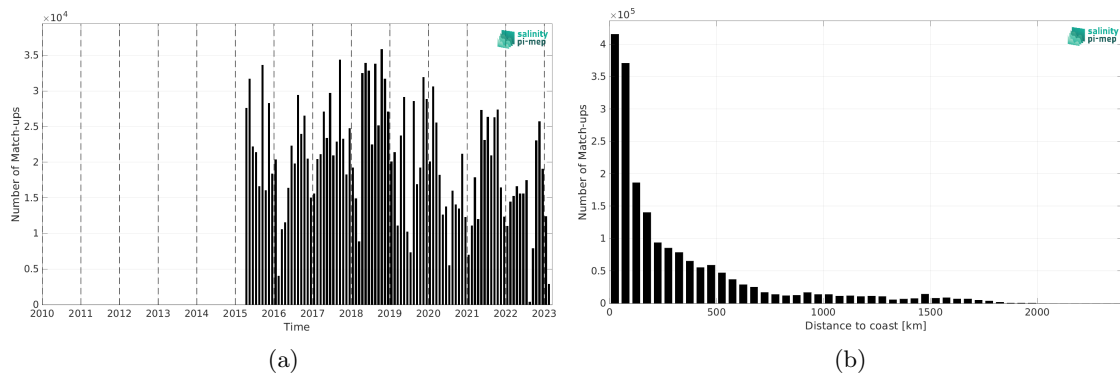
Figure 2: Number of match-ups between TSG (LEGOS-DM) and SMAP SSS L3 v6 - 8-Day running (RSS) SSS as a function of time (a) and as function of the distance to coast (b) over the North Atlantic Ocean Pi-MEP region and for the full satellite product period.
