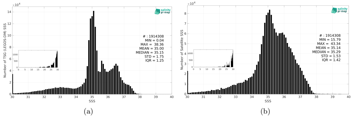
Figure 3: Histograms of SSS from TSG (LEGOS-DM) (a) and SMAP SSS L3 v6 - 8-Day running (RSS) (b) considering all match-up pairs per bins of 0.1 over the North Atlantic Ocean Pi-MEP region and for the full satellite product period.
