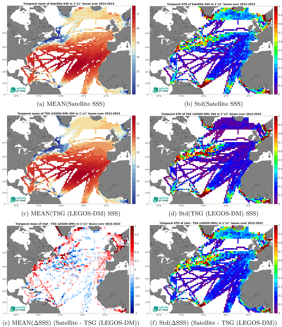
Figure 7: Temporal mean (left) and Std (right) of SSS from SMAP SSS L3 v6 - 8-Day running (RSS) (top), TSG (LEGOS-DM) (middle), and of \Delta SSS (Satellite - TSG (LEGOS-DM)). Only match-up pairs are used to generate these maps.
