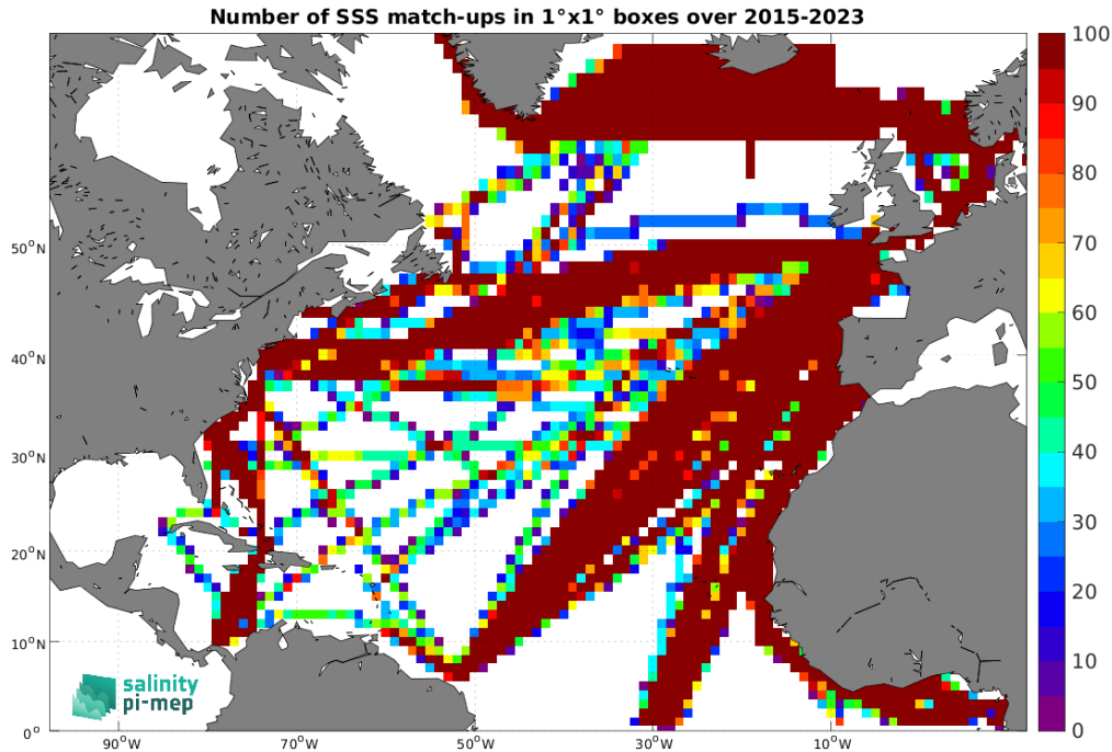
Figure 5: Number of SSS match-ups between TSG (LEGOS-DM) SSS and the SMAP SSS L3 v6 - 8-Day running (RSS) SSS product for the North Atlantic Ocean Pi-MEP region over 1^\circ \times 1^\circ boxes and for the full satellite product period.
