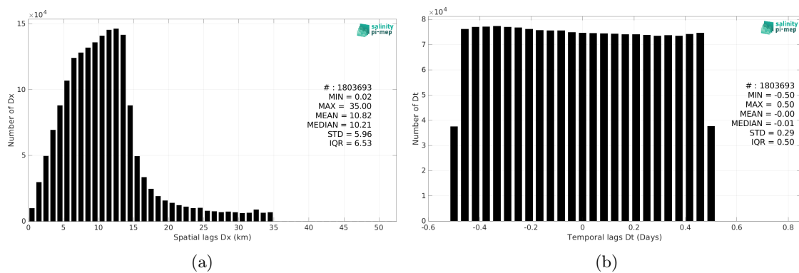
Figure 6: Histograms of the spatial (a) and temporal (b) lags between the location/time of the TSG (LEGOS-DM) measurement and the date of the corresponding SMAP SSS L3 v6 - 8-Day running (RSS) SSS pixel.
