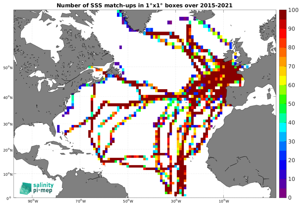
Figure 5: Number of SSS match-ups between TSG (GOSUD-Sailing-ship) SSS and the SMAP SSS L3 v6 - 8-Day running (RSS) SSS product for the North Atlantic Ocean Pi-MEP region over 1^\circ \times 1^\circ boxes and for the full satellite product period.
