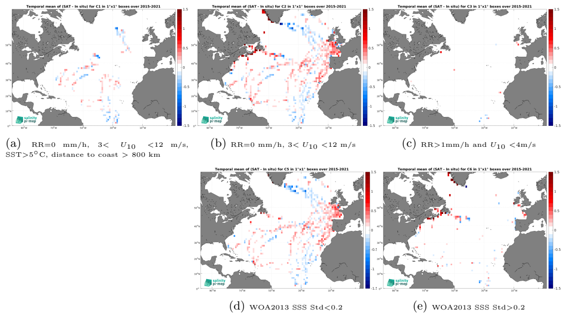
Figure 14: Temporal mean gridded over spatial boxes of size 1^\circ \times 1^\circ of \Delta\text{SSS} (SMAP SSS L3 v6 - 8-Day running (RSS) - TSG (GOSUD-Sailing-ship)) for 5 different subdatasets corresponding to:RR=0 mm/h, 3 < U_{10} < 12 m/s, SST >5^\circ\text{C} , distance to coast > 800 km (a), RR=0 mm/h, 3 < U_{10} < 12 m/s (b), RR >1 mm/h and U_{10} < 4 m/s (c), WOA2013 SSS Std <0.2 (d), WOA2013 SSS Std >0.2 (e).
