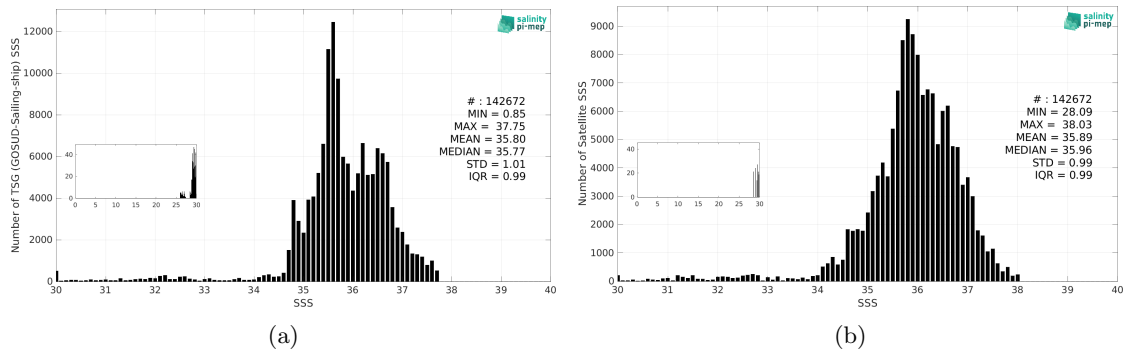
Figure 3: Histograms of SSS from TSG (GOSUD-Sailing-ship) (a) and SMAP SSS L3 v6 - 8-Day running (RSS) (b) considering all match-up pairs per bins of 0.1 over the North Atlantic Ocean Pi-MEP region and for the full satellite product period.
