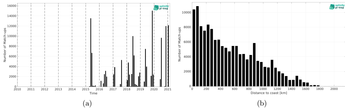
Figure 2: Number of match-ups between TSG (GOSUD-Sailing-ship) and SMAP SSS L3 v6 - 8-Day running (RSS) SSS as a function of time (a) and as function of the distance to coast (b) over the North Atlantic Ocean Pi-MEP region and for the full satellite product period.
