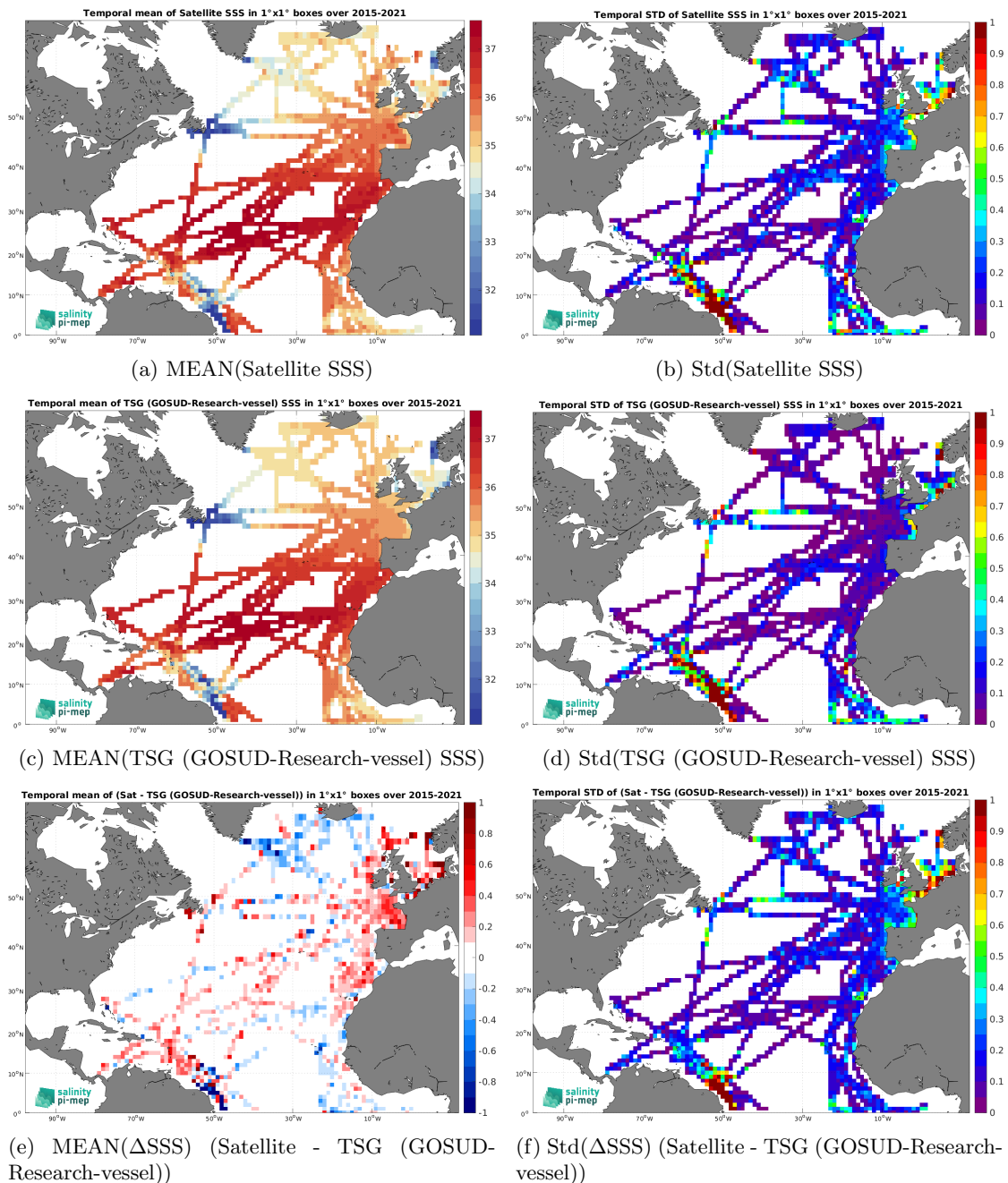
Figure 7: Temporal mean (left) and Std (right) of SSS from SMAP SSS L3 v6 - 8-Day running (RSS) (top), TSG (GOSUD-Research-vessel) (middle), and of \Delta SSS (Satellite - TSG (GOSUD-Research-vessel)). Only match-up pairs are used to generate these maps.
