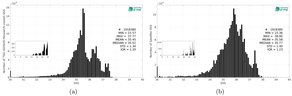
Figure 3: Histograms of SSS from TSG (GOSUD-Research-vessel) (a) and SMAP SSS L3 v6 - 8-Day running (RSS) (b) considering all match-up pairs per bins of 0.1 over the North Atlantic Ocean Pi-MEP region and for the full satellite product period.
