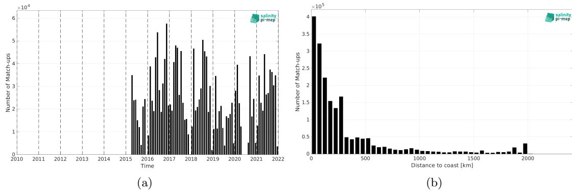
Figure 2: Number of match-ups between TSG (GOSUD-Research-vessel) and SMAP SSS L3 v6 - 8-Day running (RSS) SSS as a function of time (a) and as function of the distance to coast (b) over the North Atlantic Ocean Pi-MEP region and for the full satellite product period.
