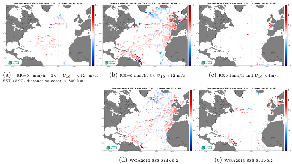
Figure 14: Temporal mean gridded over spatial boxes of size 1^\circ \times 1^\circ of \Delta\text{SSS} (SMAP SSS L3 v6 - 8-Day running (RSS) - TSG (GOSUD-Research-vessel)) for 5 different subdatasets corresponding to:RR=0 mm/h, 3 < U_{10} < 12 m/s, SST >5^\circ\text{C} , distance to coast > 800 km (a), RR=0 mm/h, 3 < U_{10} < 12 m/s (b), RR >1 mm/h and U_{10} < 4 m/s (c), WOA2013 SSS Std <0.2 (d), WOA2013 SSS Std >0.2 (e).
