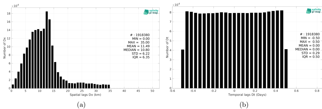
Figure 6: Histograms of the spatial (a) and temporal (b) lags between the location/time of the TSG (GOSUD-Research-vessel) measurement and the date of the corresponding SMAP SSS L3 v6 - 8-Day running (RSS) SSS pixel.
