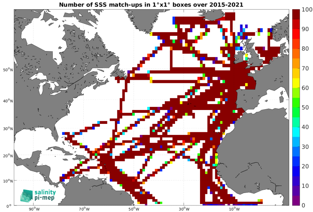
Figure 5: Number of SSS match-ups between TSG (GOSUD-Research-vessel) SSS and the SMAP SSS L3 v6 - 8-Day running (RSS) SSS product for the North Atlantic Ocean Pi-MEP region over 1^\circ \times 1^\circ boxes and for the full satellite product period.
