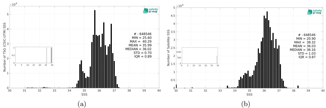
Figure 3: Histograms of SSS from TSG (CSIC-UTM) (a) and SMAP SSS L3 v6 - 8-Day running (RSS) (b) considering all match-up pairs per bins of 0.1 over the North Atlantic Ocean Pi-MEP region and for the full satellite product period.
