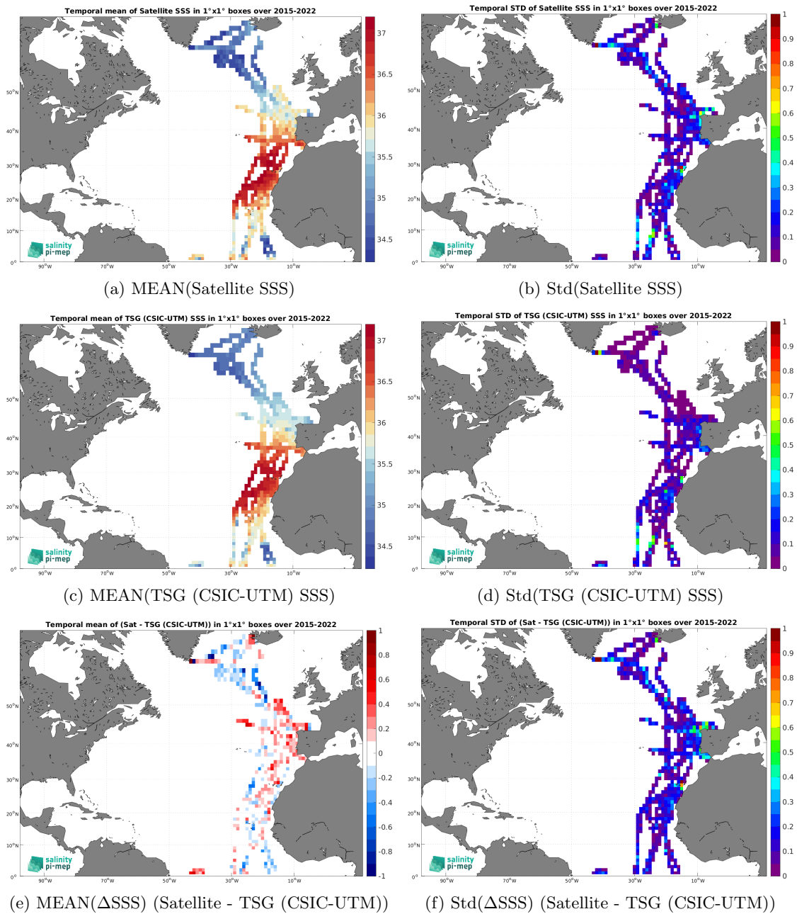
Figure 7: Temporal mean (left) and Std (right) of SSS from SMAP SSS L3 v6 - 8-Day running (RSS) (top), TSG (CSIC-UTM) (middle), and of \Delta SSS (Satellite - TSG (CSIC-UTM)). Only match-up pairs are used to generate these maps.
