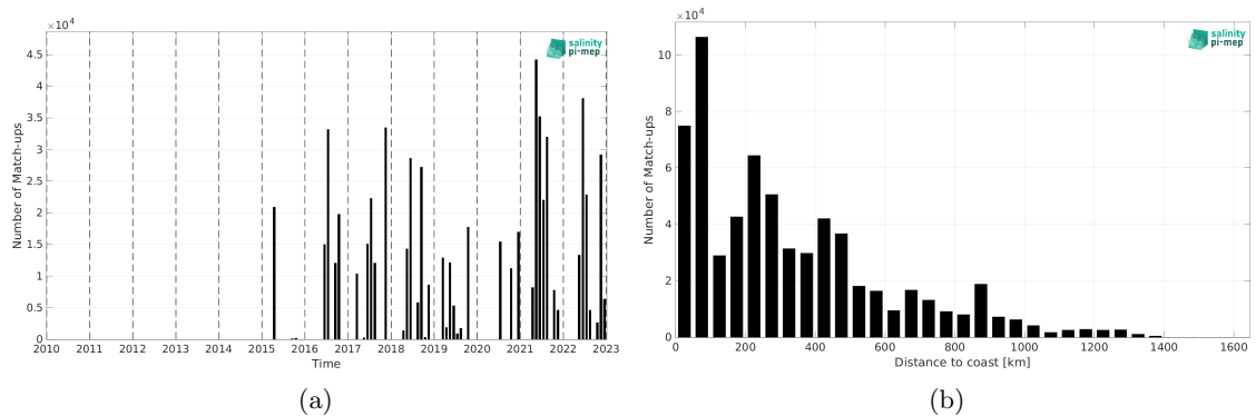
Figure 2: Number of match-ups between TSG (CSIC-UTM) and SMAP SSS L3 v6 - 8-Day running (RSS) SSS as a function of time (a) and as function of the distance to coast (b) over the North Atlantic Ocean Pi-MEP region and for the full satellite product period.
