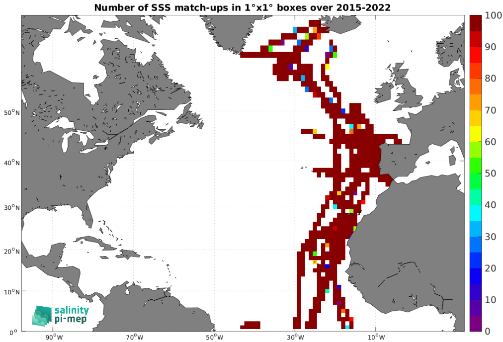
Figure 5: Number of SSS match-ups between TSG (CSIC-UTM) SSS and the SMAP SSS L3 v6 - 8-Day running (RSS) SSS product for the North Atlantic Ocean Pi-MEP region over 1^\circ \times 1^\circ boxes and for the full satellite product period.
