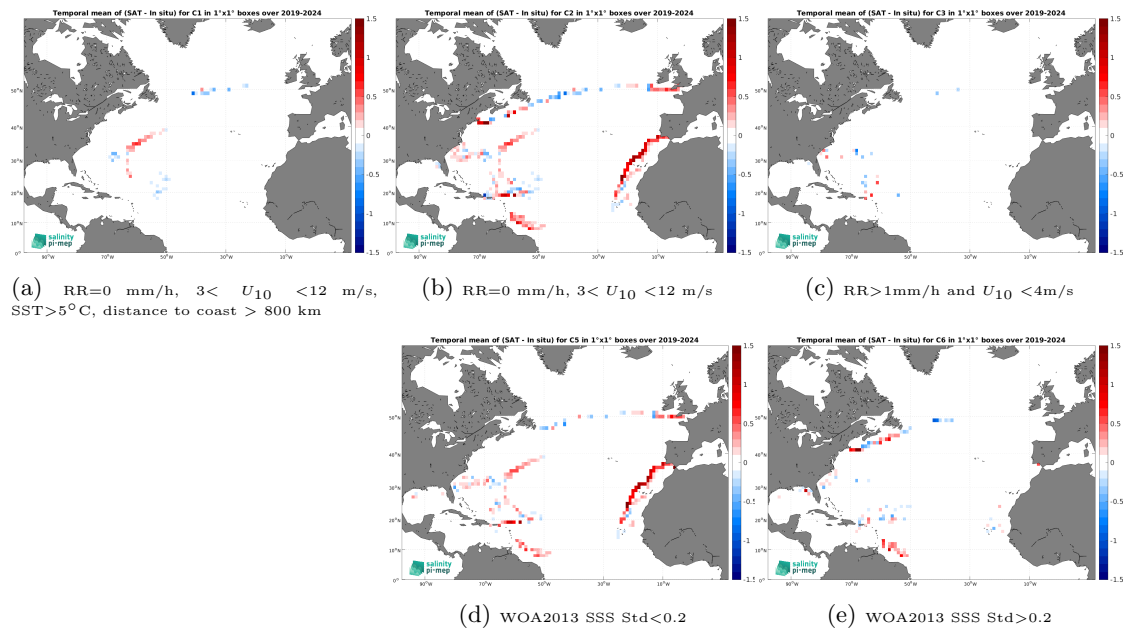
Figure 14: Temporal mean gridded over spatial boxes of size 1^\circ \times 1^\circ of \Delta\text{SSS} (SMAP SSS L3 v6 - 8-Day running (RSS) - Saildrone) for 5 different subdatasets corresponding to:RR=0 mm/h, 3 < U_{10} < 12 m/s, SST>5°C, distance to coast > 800 km (a), RR=0 mm/h, 3 < U_{10} < 12 m/s (b), RR>1mm/h and U_{10} < 4 m/s (c), WOA2013 SSS Std<0.2 (d), WOA2013 SSS Std>0.2 (e).
