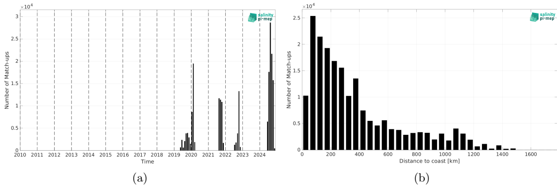
Figure 2: Number of match-ups between Sairdrone and SMAP SSS L3 v6 - 8-Day running (RSS) SSS as a function of time (a) and as function of the distance to coast (b) over the North Atlantic Ocean Pi-MEP region and for the full satellite product period.
