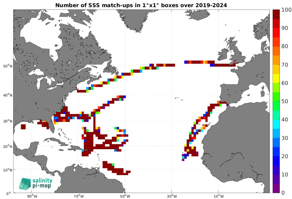
Figure 5: Number of SSS match-ups between Saildrone SSS and the SMAP SSS L3 v6 - 8-Day running (RSS) SSS product for the North Atlantic Ocean Pi-MEP region over 1^\circ \times 1^\circ boxes and for the full satellite product period.
