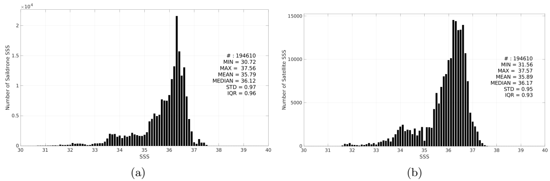
Figure 3: Histograms of SSS from Saildrone (a) and SMAP SSS L3 v6 - 8-Day running (RSS) (b) considering all match-up pairs per bins of 0.1 over the North Atlantic Ocean Pi-MEP region and for the full satellite product period.
