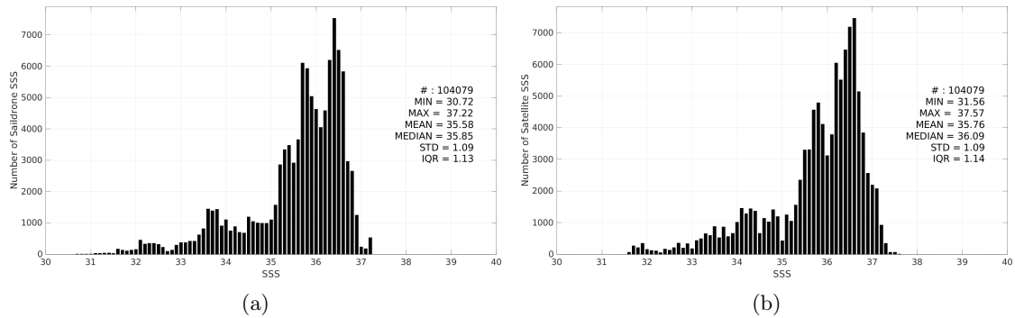
Figure 3: Histograms of SSS from Saildrone (a) and SMAP SSS L3 v6 - 8-Day running (RSS) (b) considering all match-up pairs per bins of 0.1 over the North Atlantic Ocean Pi-MEP region and for the full satellite product period.
