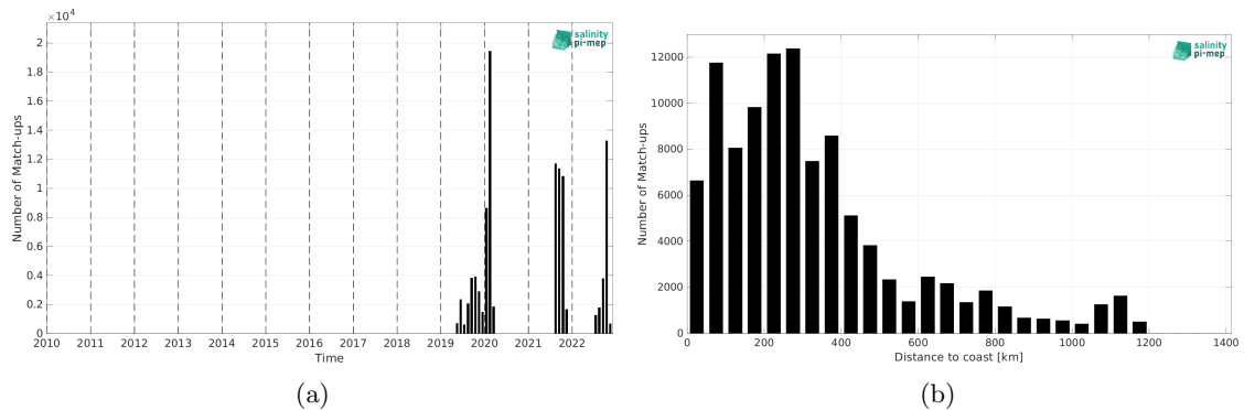
Figure 2: Number of match-ups between Saildrone and SMAP SSS L3 v6 - 8-Day running (RSS) SSS as a function of time (a) and as function of the distance to coast (b) over the North Atlantic Ocean Pi-MEP region and for the full satellite product period.
