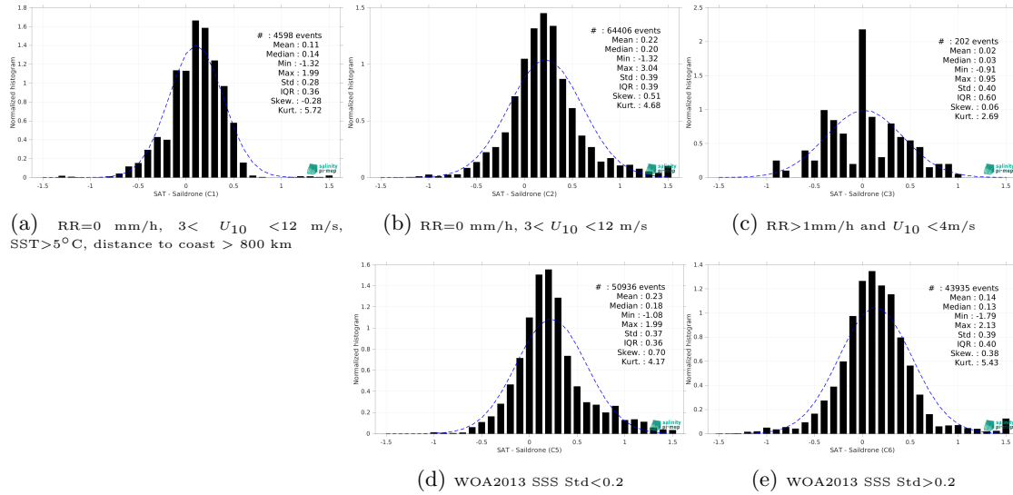
Figure 15: Normalized histogram of \Delta SSS (SMAP SSS L3 v6 - 8-Day running (RSS) - Sairdronne) for 5 different subdatasets corresponding to: RR=0 mm/h, 3 < U_{10} < 12 m/s, SST > 5°C, distance to coast > 800 km (a), RR=0 mm/h, 3 < U_{10} < 12 m/s (b), RR > 1mm/h and U_{10} < 4 m/s (c), WOA2013 SSS Std < 0.2 (d), WOA2013 SSS Std > 0.2 (e).
