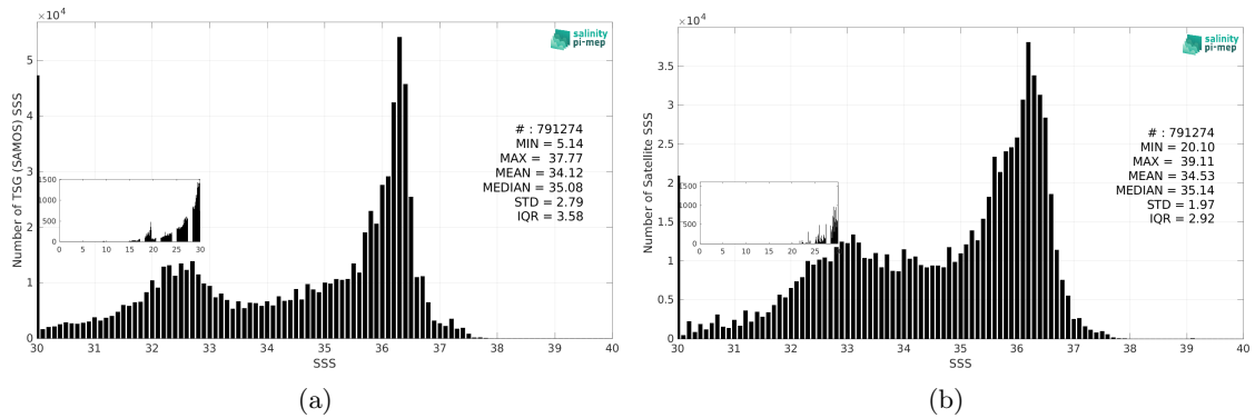
Figure 3: Histograms of SSS from TSG (SAMOS) (a) and SMAP SSS L3 v6 - Monthly (RSS) (b) considering all match-up pairs per bins of 0.1 over the North Atlantic Ocean Pi-MEP region and for the full satellite product period.
