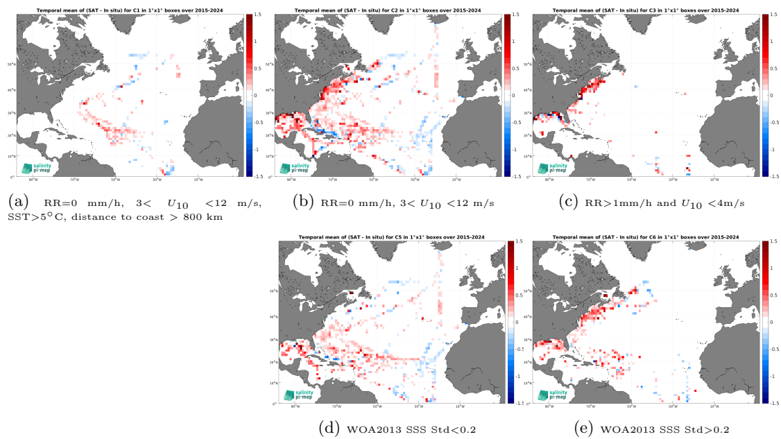
Figure 14: Temporal mean gridded over spatial boxes of size 1^\circ \times 1^\circ of \Delta\text{SSS} (SMAP SSS L3 v6 - Monthly (RSS) - TSG (SAMOS)) for 5 different subdatasets corresponding to:RR=0 mm/h, 3 < U_{10} < 12 m/s, SST >5^\circ\text{C} , distance to coast > 800 km (a), RR=0 mm/h, 3 < U_{10} < 12 m/s (b), RR >1 mm/h and U_{10} < 4 m/s (c), WOA2013 SSS Std <0.2 (d), WOA2013 SSS Std >0.2 (e).
