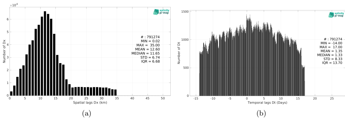
Figure 6: Histograms of the spatial (a) and temporal (b) lags between the location/time of the TSG (SAMOS) measurement and the date of the corresponding SMAP SSS L3 v6 - Monthly (RSS) SSS pixel.
