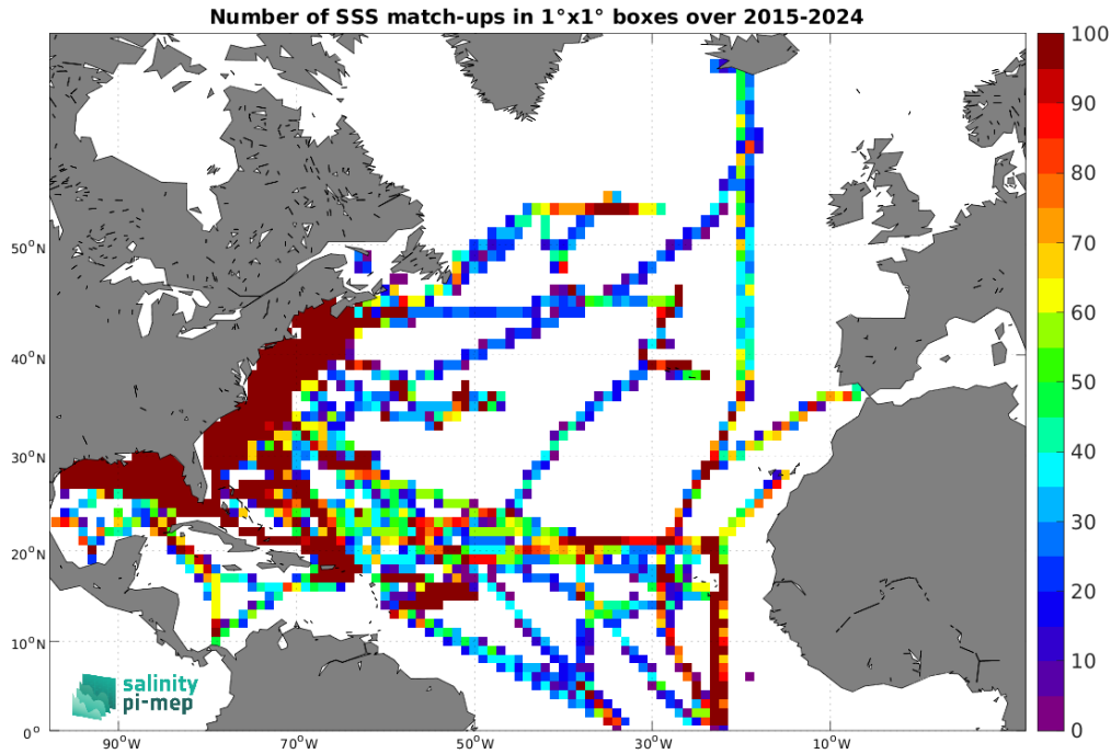
Figure 5: Number of SSS match-ups between TSG (SAMOS) SSS and the SMAP SSS L3 v6 - Monthly (RSS) SSS product for the North Atlantic Ocean Pi-MEP region over 1^\circ \times 1^\circ boxes and for the full satellite product period.
