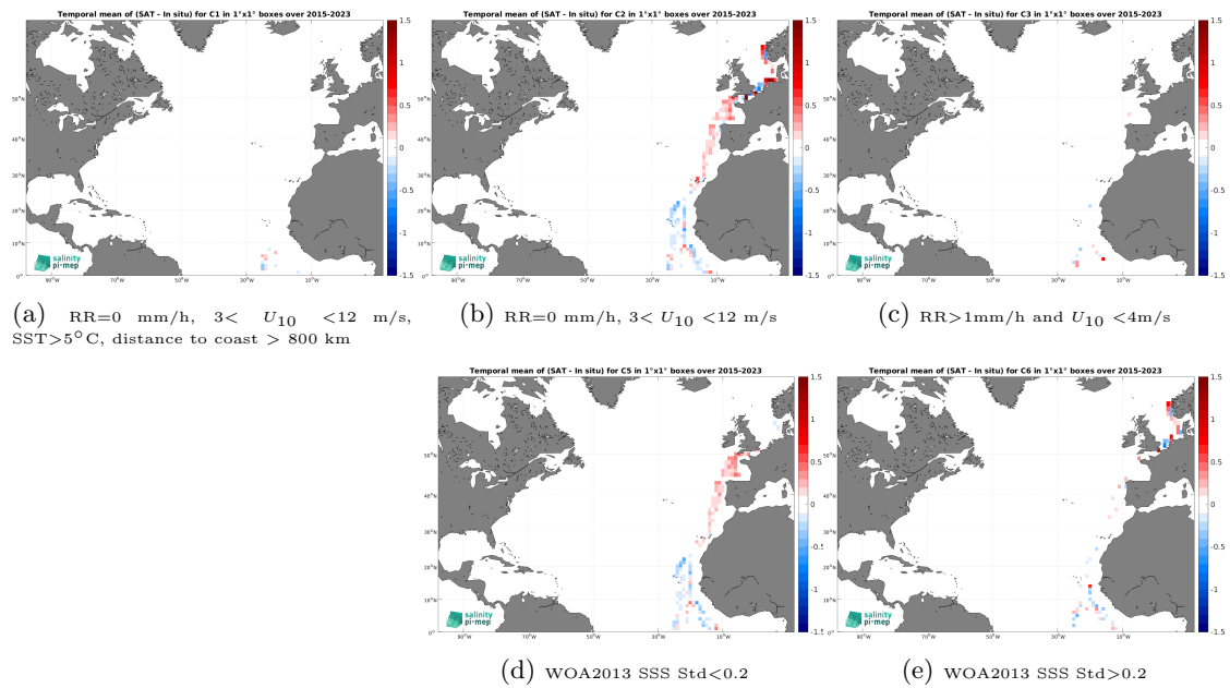
Figure 14: Temporal mean gridded over spatial boxes of size 1^\circ \times 1^\circ of \Delta\text{SSS} (SMAP SSS L3 v6 - Monthly (RSS) - TSG (Polarstern)) for 5 different subdatasets corresponding to: RR=0 mm/h, 3 < U_{10} < 12 m/s, SST > 5°C, distance to coast > 800 km (a), RR=0 mm/h, 3 < U_{10} < 12 m/s (b), RR > 1mm/h and U_{10} < 4 m/s (c), WOA2013 SSS Std < 0.2 (d), WOA2013 SSS Std > 0.2 (e).
