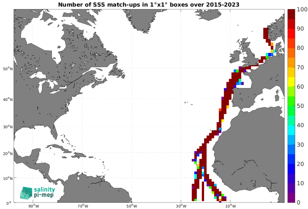
Figure 5: Number of SSS match-ups between TSG (Polarstern) SSS and the SMAP SSS L3 v6 - Monthly (RSS) SSS product for the North Atlantic Ocean Pi-MEP region over 1^\circ \times 1^\circ boxes and for the full satellite product period.
