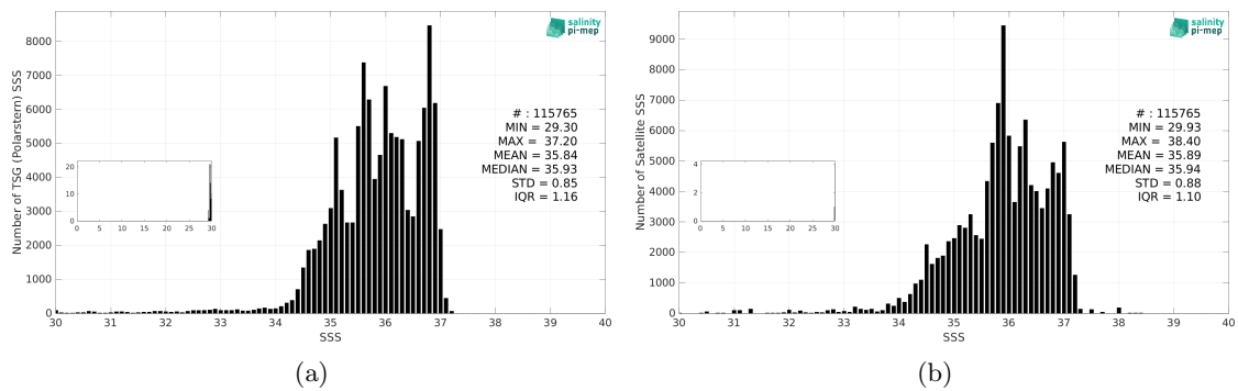
Figure 3: Histograms of SSS from TSG (Polarstern) (a) and SMAP SSS L3 v6 - Monthly (RSS) (b) considering all match-up pairs per bins of 0.1 over the North Atlantic Ocean Pi-MEP region and for the full satellite product period.
