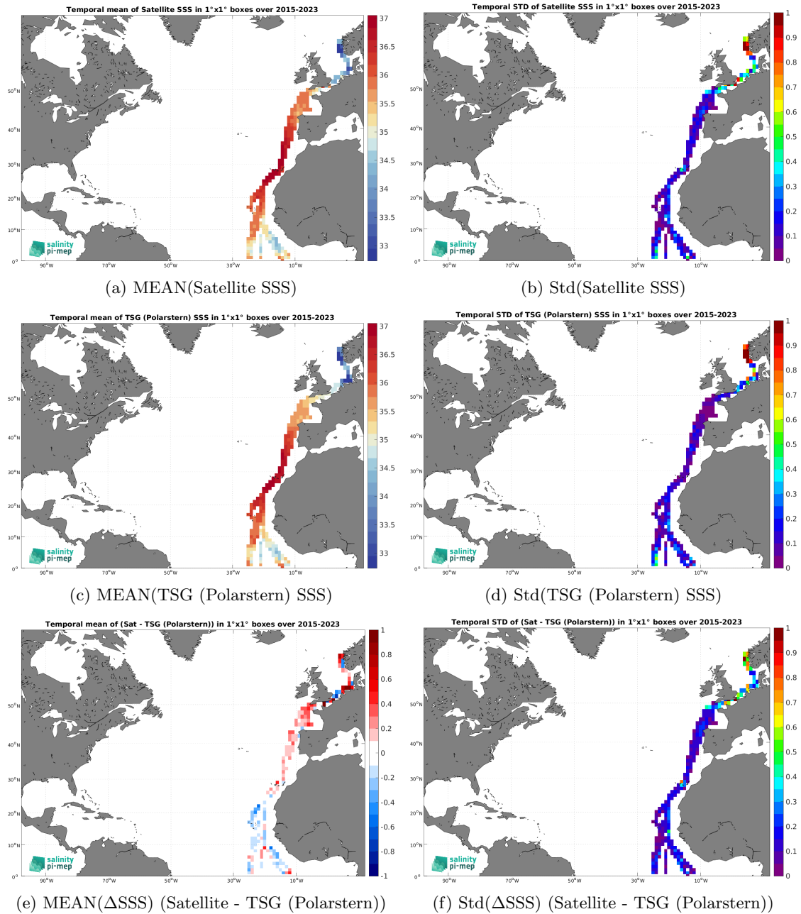
Figure 7: Temporal mean (left) and Std (right) of SSS from SMAP SSS L3 v6 - Monthly (RSS) (top), TSG (Polarstern) (middle), and of \Delta SSS (Satellite - TSG (Polarstern)). Only match-up pairs are used to generate these maps.
