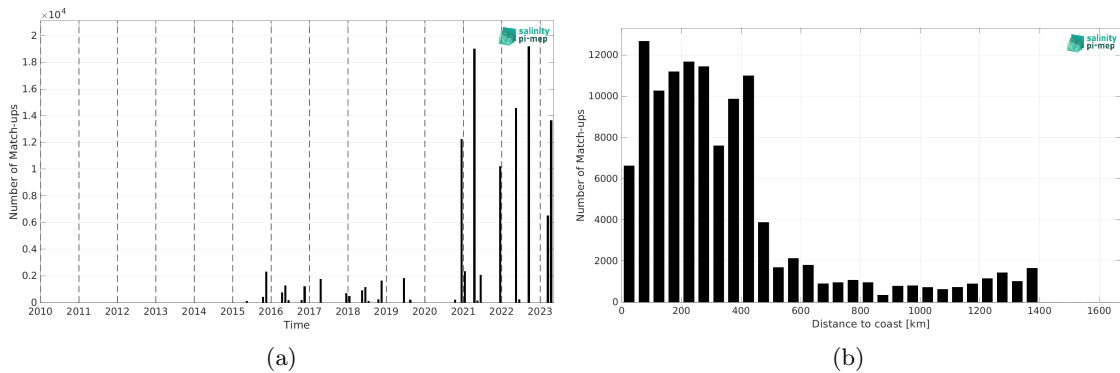
Figure 2: Number of match-ups between TSG (Polarstern) and SMAP SSS L3 v6 - Monthly (RSS) SSS as a function of time (a) and as function of the distance to coast (b) over the North Atlantic Ocean Pi-MEP region and for the full satellite product period.
