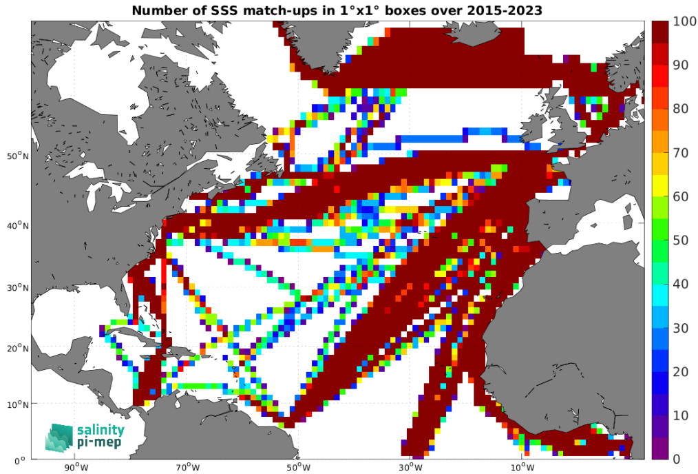
Figure 5: Number of SSS match-ups between TSG (LEGOS-DM) SSS and the SMAP SSS L3 v6 - Monthly (RSS) SSS product for the North Atlantic Ocean Pi-MEP region over 1°x1° boxes and for the full satellite product period.
