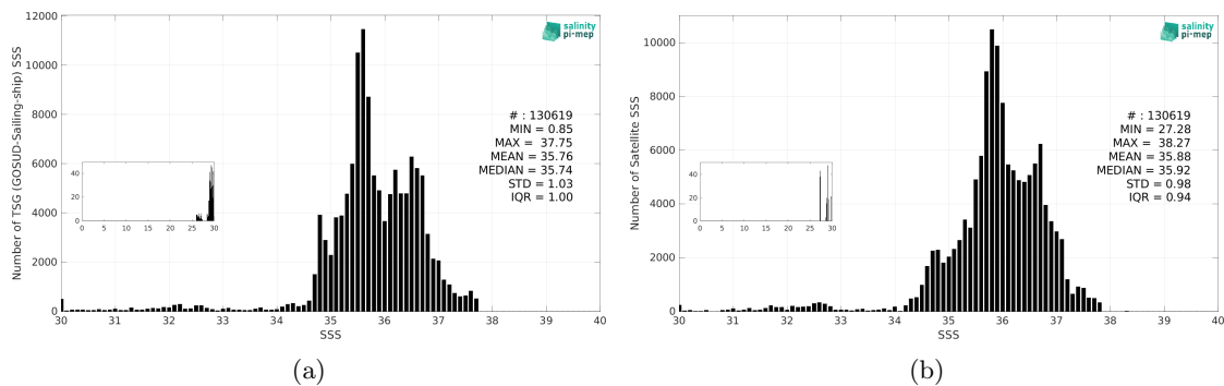
Figure 3: Histograms of SSS from TSG (GOSUD-Sailing-ship) (a) and SMAP SSS L3 v6 - Monthly (RSS) (b) considering all match-up pairs per bins of 0.1 over the North Atlantic Ocean Pi-MEP region and for the full satellite product period.
