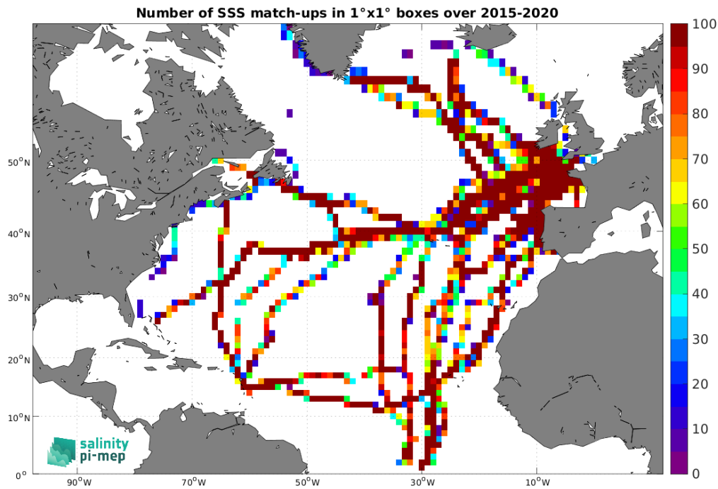
Figure 5: Number of SSS match-ups between TSG (GOSUD-Sailing-ship) SSS and the SMAP SSS L3 v6 - Monthly (RSS) SSS product for the North Atlantic Ocean Pi-MEP region over 1^\circ \times 1^\circ boxes and for the full satellite product period.
