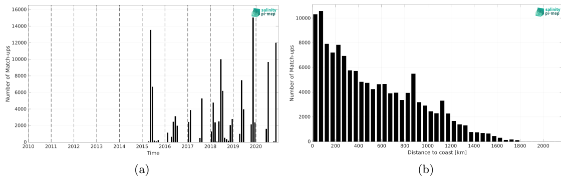
Figure 2: Number of match-ups between TSG (GOSUD-Sailing-ship) and SMAP SSS L3 v6 - Monthly (RSS) SSS as a function of time (a) and as function of the distance to coast (b) over the North Atlantic Ocean Pi-MEP region and for the full satellite product period.
