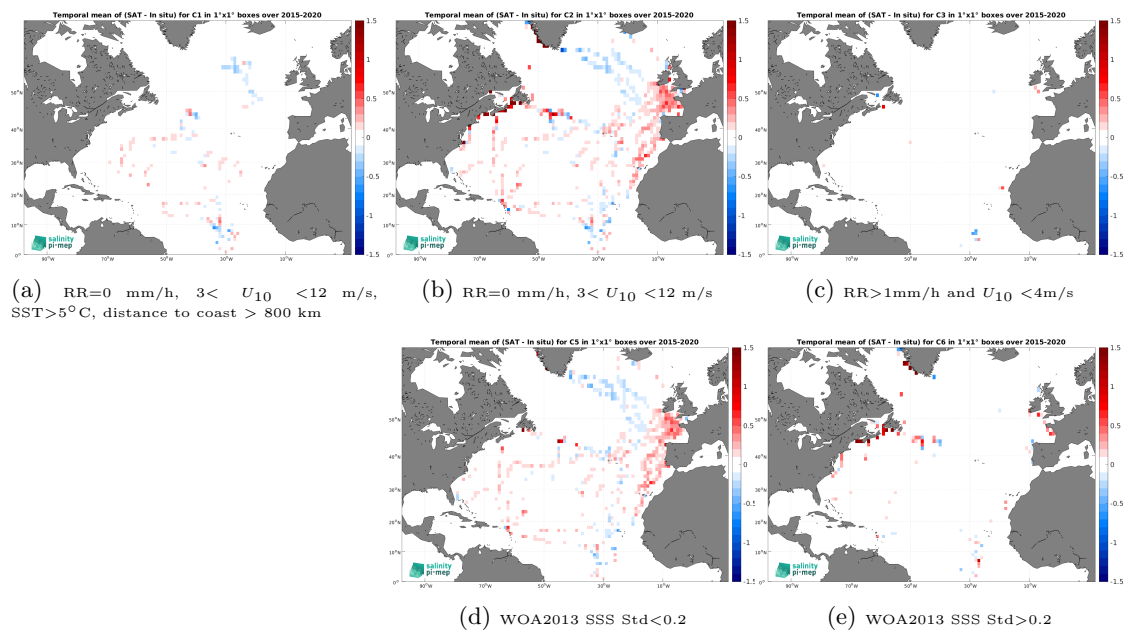
Figure 14: Temporal mean gridded over spatial boxes of size 1^\circ \times 1^\circ of \Delta\text{SSS} (SMAP SSS L3 v6 - Monthly (RSS) - TSG (GOSUD-Sailing-ship)) for 5 different subdatasets corresponding to:RR=0 mm/h, 3 < U_{10} < 12 m/s, SST >5^\circ\text{C} , distance to coast > 800 km (a), RR=0 mm/h, 3 < U_{10} < 12 m/s (b), RR >1 mm/h and U_{10} < 4 m/s (c), WOA2013 SSS Std <0.2 (d), WOA2013 SSS Std >0.2 (e).
