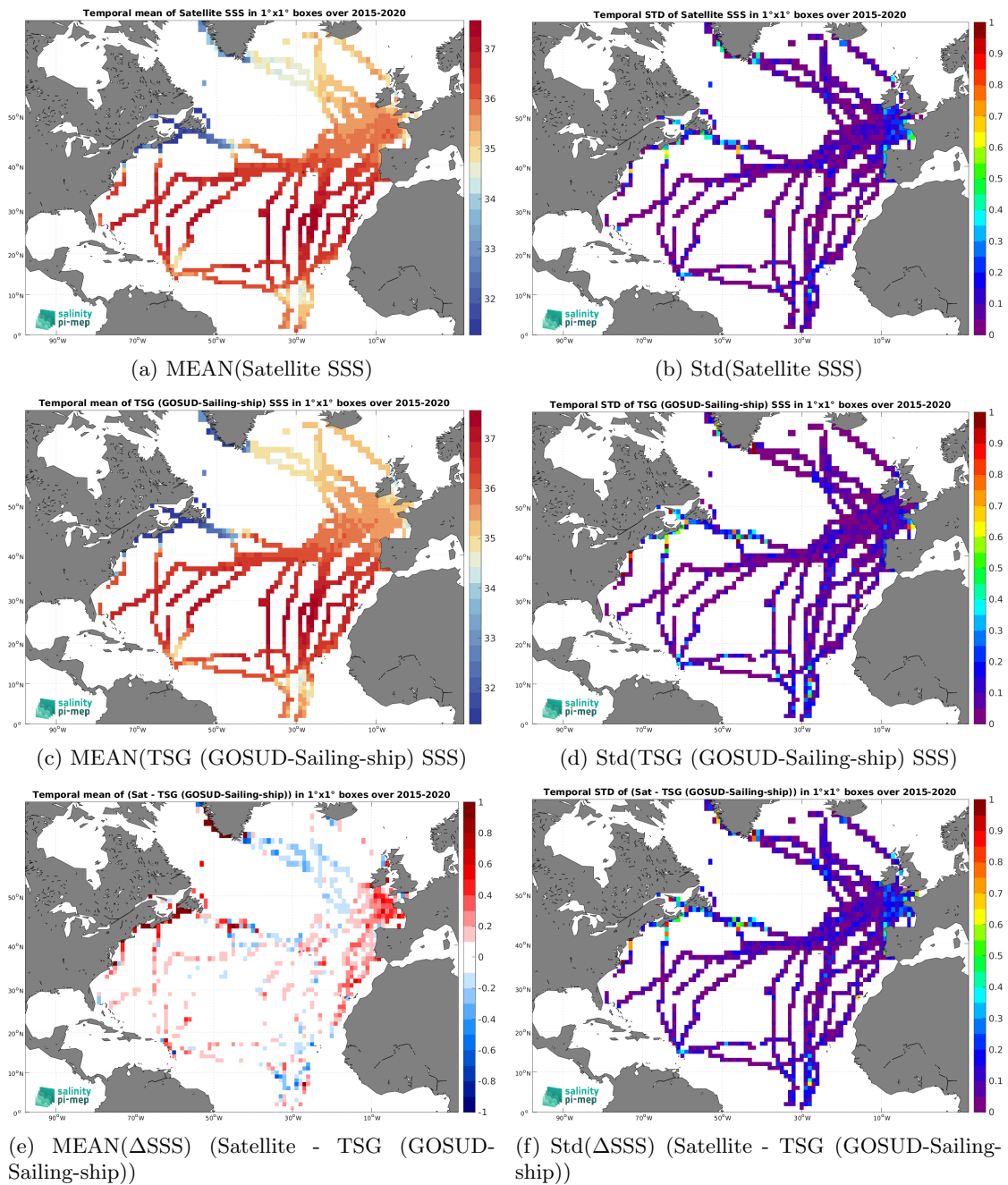
Figure 7: Temporal mean (left) and Std (right) of SSS from SMAP SSS L3 v6 - Monthly (RSS) (top), TSG (GOSUD-Sailing-ship) (middle), and of \Delta SSS (Satellite - TSG (GOSUD-Sailing-ship)). Only match-up pairs are used to generate these maps.
