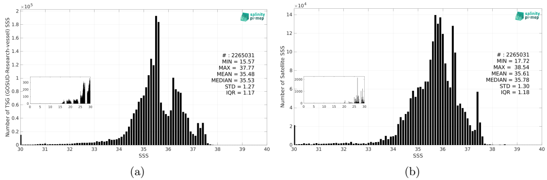
Figure 3: Histograms of SSS from TSG (GOSUD-Research-vessel) (a) and SMAP SSS L3 v6 - Monthly (RSS) (b) considering all match-up pairs per bins of 0.1 over the North Atlantic Ocean Pi-MEP region and for the full satellite product period.
