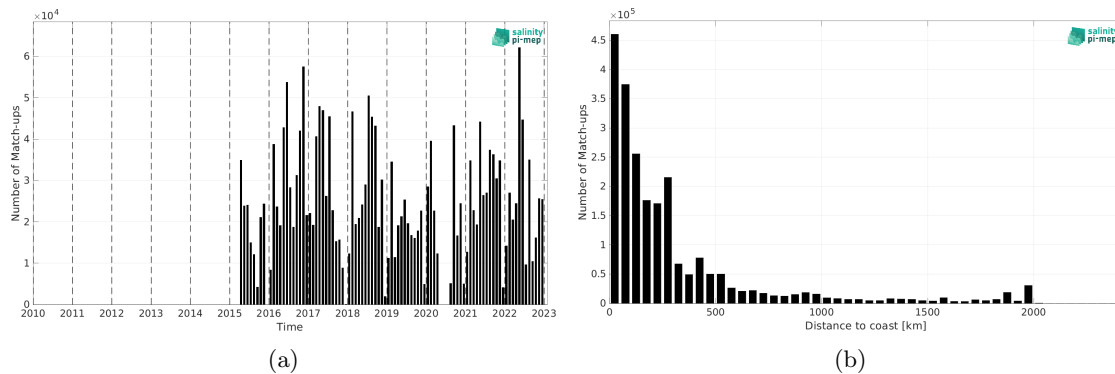
Figure 2: Number of match-ups between TSG (GOSUD-Research-vessel) and SMAP SSS L3 v6 - Monthly (RSS) SSS as a function of time (a) and as function of the distance to coast (b) over the North Atlantic Ocean Pi-MEP region and for the full satellite product period.
