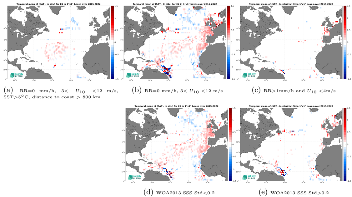
Figure 14: Temporal mean gridded over spatial boxes of size 1^\circ \times 1^\circ of \Delta\text{SSS} (SMAP SSS L3 v6 - Monthly (RSS) - TSG (GOSUD-Research-vessel)) for 5 different subdatasets corresponding to:RR=0 mm/h, 3 < U_{10} < 12 m/s, SST >5^\circ\text{C} , distance to coast > 800 km (a), RR=0 mm/h, 3 < U_{10} < 12 m/s (b), RR >1 mm/h and U_{10} < 4 m/s (c), WOA2013 SSS Std <0.2 (d), WOA2013 SSS Std >0.2 (e).
