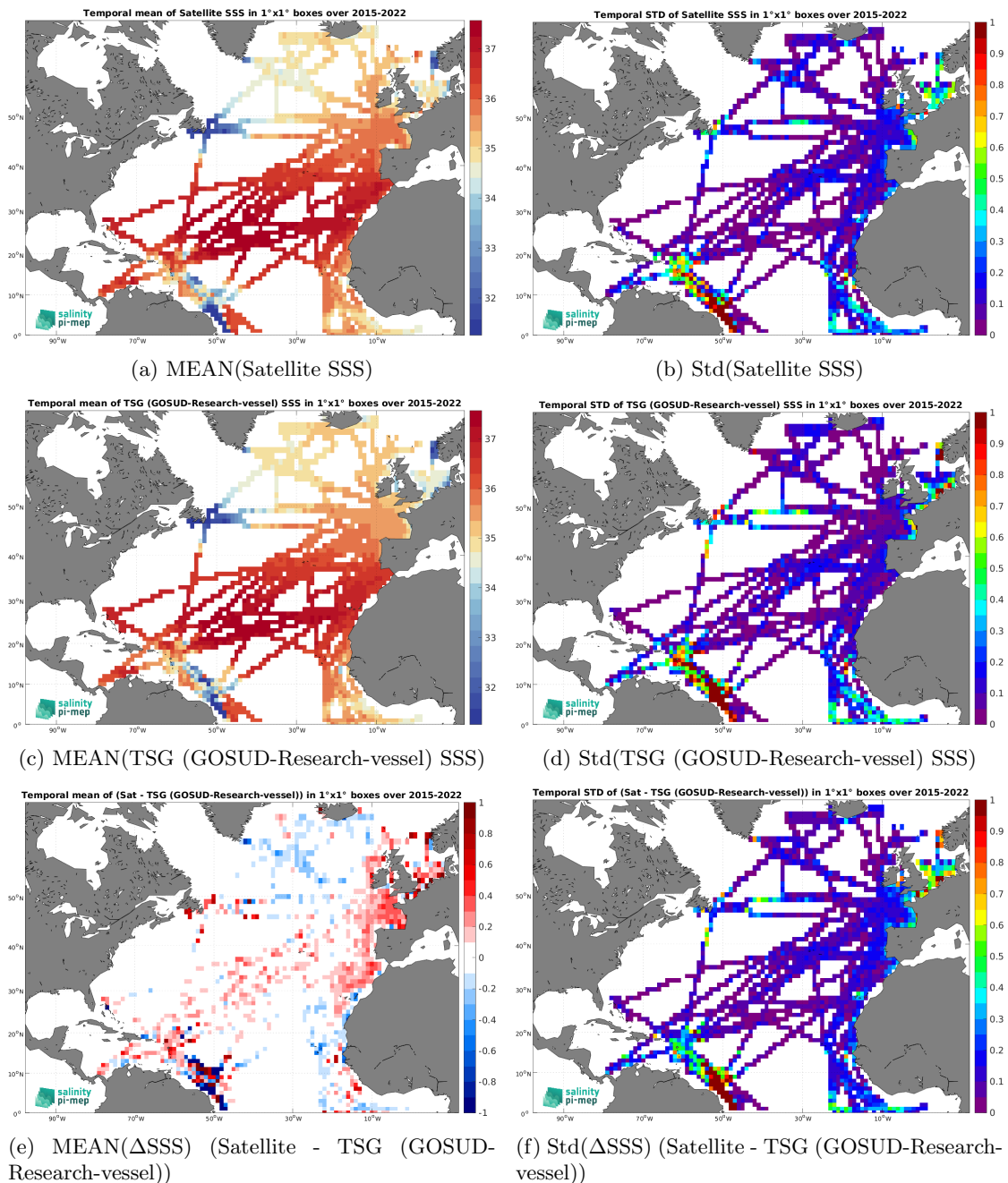
Figure 7: Temporal mean (left) and Std (right) of SSS from SMAP SSS L3 v6 - Monthly (RSS) (top), TSG (GOSUD-Research-vessel) (middle), and of \Delta SSS (Satellite - TSG (GOSUD-Research-vessel)). Only match-up pairs are used to generate these maps.
