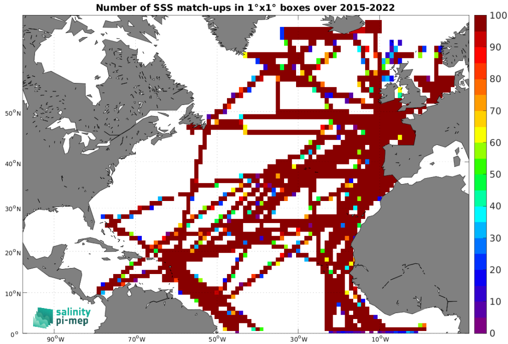
Figure 5: Number of SSS match-ups between TSG (GOSUD-Research-vessel) SSS and the SMAP SSS L3 v6 - Monthly (RSS) SSS product for the North Atlantic Ocean Pi-MEP region over 1^\circ \times 1^\circ boxes and for the full satellite product period.
