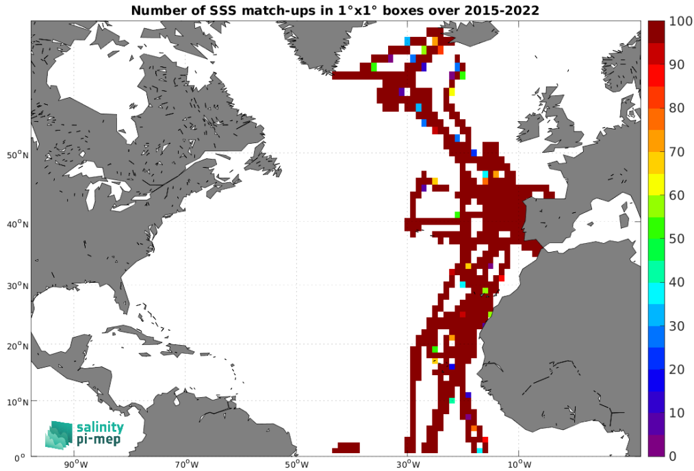
Figure 5: Number of SSS match-ups between TSG (CSIC-UTM) SSS and the SMAP SSS L3 v6 - Monthly (RSS) SSS product for the North Atlantic Ocean Pi-MEP region over 1^\circ \times 1^\circ boxes and for the full satellite product period.
