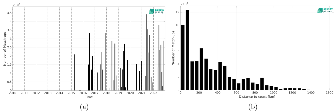
Figure 2: Number of match-ups between TSG (CSIC-UTM) and SMAP SSS L3 v6 - Monthly (RSS) SSS as a function of time (a) and as function of the distance to coast (b) over the North Atlantic Ocean Pi-MEP region and for the full satellite product period.
