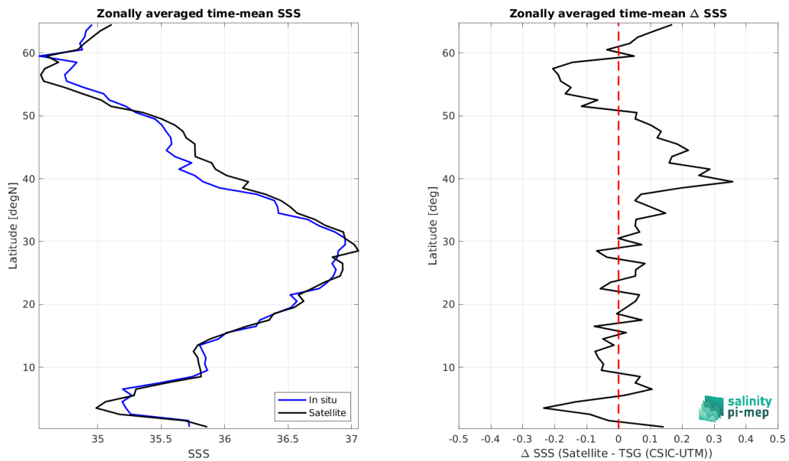
Figure 9: Left panel: Zonal mean SSS from SMAP SSS L3 v6 - Monthly (RSS) satellite product (black) and from TSG (CSIC-UTM) (blue). Right panel: Zonal mean of \Delta SSS (Satellite - TSG (CSIC-UTM)) for all the collected Pi-MEP match-up pairs estimated over the full satellite product period.
