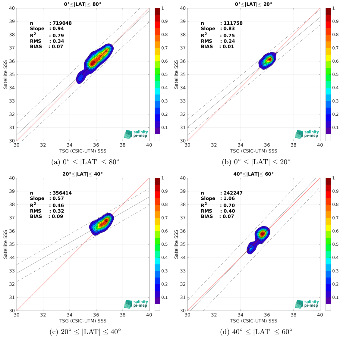
Figure 10: Contour maps of the concentration of SMAP SSS L3 v6 - Monthly (RSS) SSS (y-axis) versus TSG (CSIC-UTM) SSS (x-axis) at match-up pairs for different latitude bands. For each plot, the red line shows x=y . The black thin and dashed lines indicate a linear fit through the data cloud and the \pm 95\% confidence levels, respectively. The number match-up pairs n , the slope and R^2 coefficient of the linear fit, the root mean square (RMS) and the mean bias between satellite and in situ data are indicated for each latitude band in each plots.
