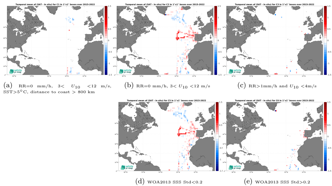
Figure 14: Temporal mean gridded over spatial boxes of size 1^\circ \times 1^\circ of \Delta\text{SSS} (SMAP SSS L3 v6 - Monthly (RSS) - TSG (CSIC-UTM)) for 5 different subdatasets corresponding to:RR=0 mm/h, 3 < U_{10} < 12 m/s, SST >5^\circ\text{C} , distance to coast > 800 km (a), RR=0 mm/h, 3 < U_{10} < 12 m/s (b), RR >1 mm/h and U_{10} < 4 m/s (c), WOA2013 SSS Std <0.2 (d), WOA2013 SSS Std >0.2 (e).
