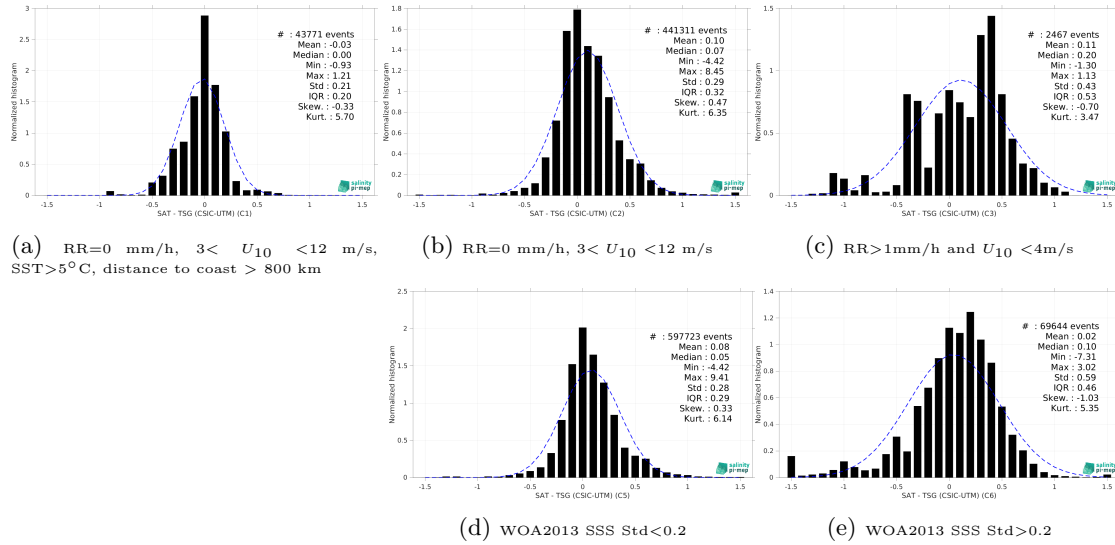
Figure 15: Normalized histogram of \Delta SSS (SMAP SSS L3 v6 - Monthly (RSS) - TSG (CSIC-UTM)) for 5 different subdatasets corresponding to: RR=0 mm/h, 3 < U_{10} < 12 m/s, SST > 5°C, distance to coast > 800 km (a), RR=0 mm/h, 3 < U_{10} < 12 m/s (b), RR > 1mm/h and U_{10} < 4 m/s (c), WOA2013 SSS Std < 0.2 (d), WOA2013 SSS Std > 0.2 (e).
