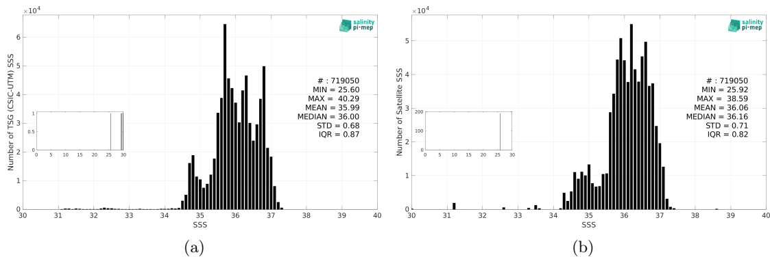
Figure 3: Histograms of SSS from TSG (CSIC-UTM) (a) and SMAP SSS L3 v6 - Monthly (RSS) (b) considering all match-up pairs per bins of 0.1 over the North Atlantic Ocean Pi-MEP region and for the full satellite product period.
