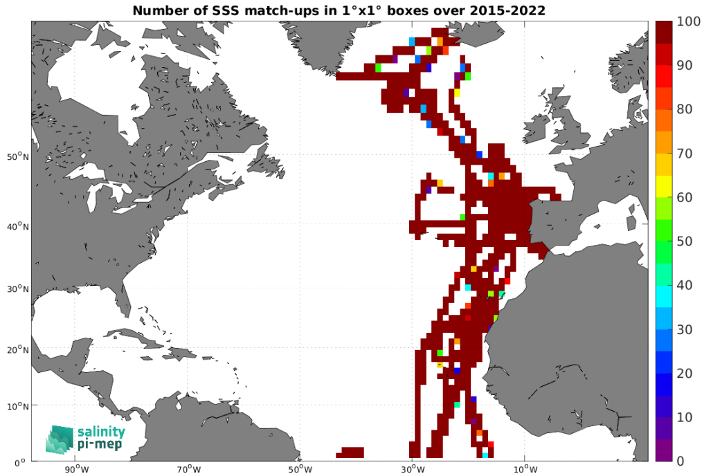
Figure 5: Number of SSS match-ups between TSG (CSIC-UTM) SSS and the SMAP SSS L3 v6 - Monthly (RSS) SSS product for the North Atlantic Ocean Pi-MEP region over 1°x1° boxes and for the full satellite product period.
