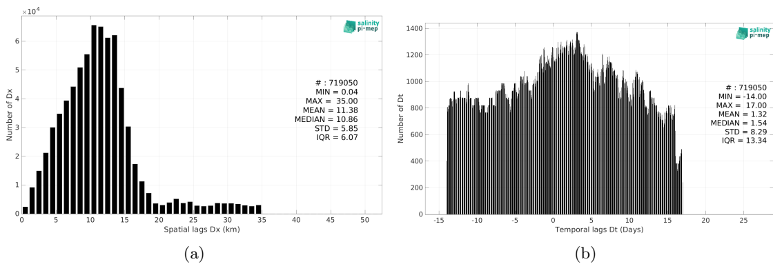
Figure 6: Histograms of the spatial (a) and temporal (b) lags between the location/time of the TSG (CSIC-UTM) measurement and the date of the corresponding SMAP SSS L3 v6 - Monthly (RSS) SSS pixel.
