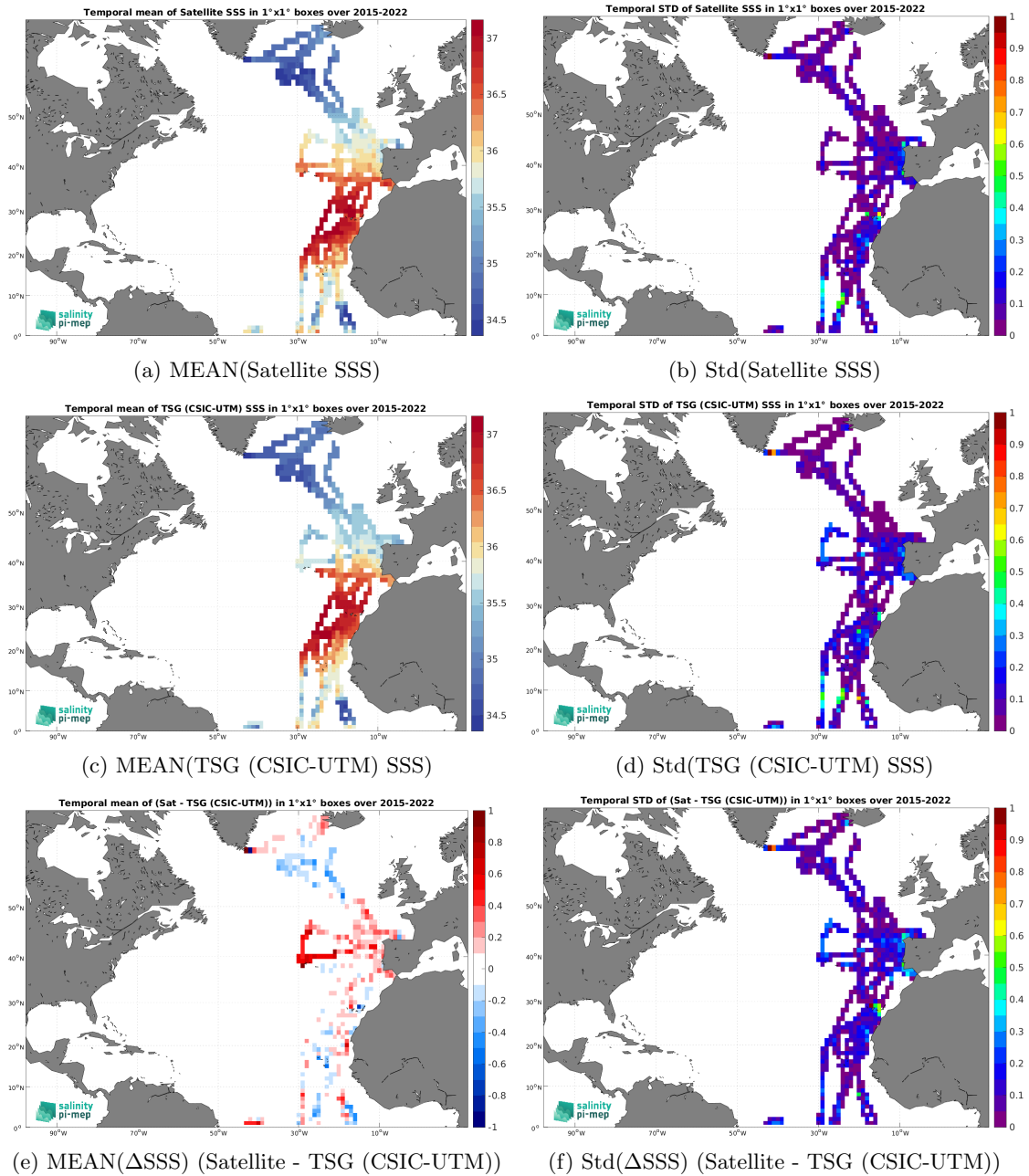
Figure 7: Temporal mean (left) and Std (right) of SSS from SMAP SSS L3 v6 - Monthly (RSS) (top), TSG (CSIC-UTM) (middle), and of \Delta SSS (Satellite - TSG (CSIC-UTM)). Only match-up pairs are used to generate these maps.
