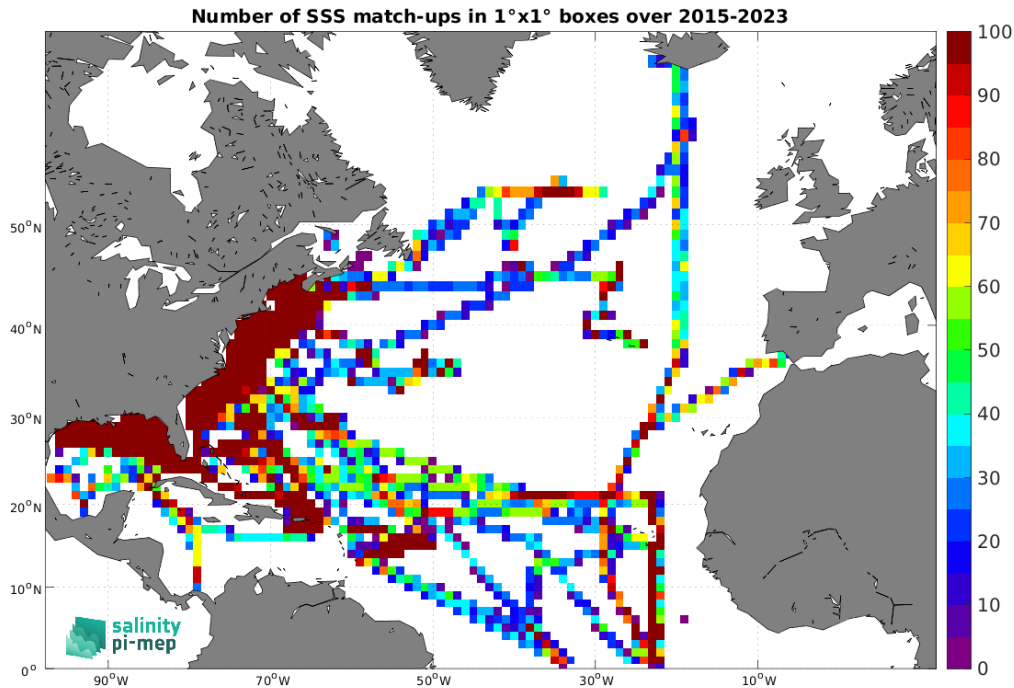
Figure 5: Number of SSS match-ups between TSG (SAMOS) SSS and the SMAP SSS L3 v5.3 - 8-Day running (RSS) SSS product for the North Atlantic Ocean Pi-MEP region over 1^\circ \times 1^\circ boxes and for the full satellite product period.
