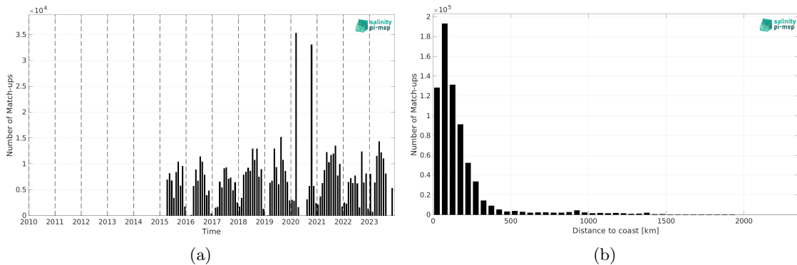
Figure 2: Number of match-ups between TSG (SAMOS) and SMAP SSS L3 v5.3 - 8-Day running (RSS) SSS as a function of time (a) and as function of the distance to coast (b) over the North Atlantic Ocean Pi-MEP region and for the full satellite product period.
