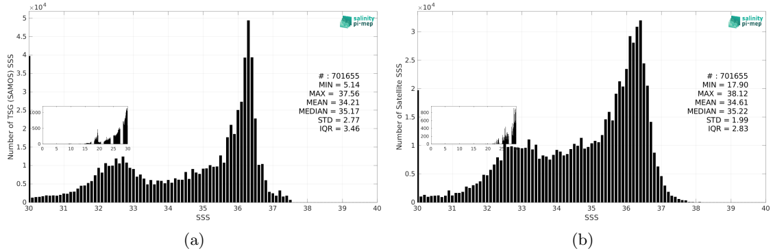
Figure 3: Histograms of SSS from TSG (SAMOS) (a) and SMAP SSS L3 v5.3 - 8-Day running (RSS) (b) considering all match-up pairs per bins of 0.1 over the North Atlantic Ocean Pi-MEP region and for the full satellite product period.
