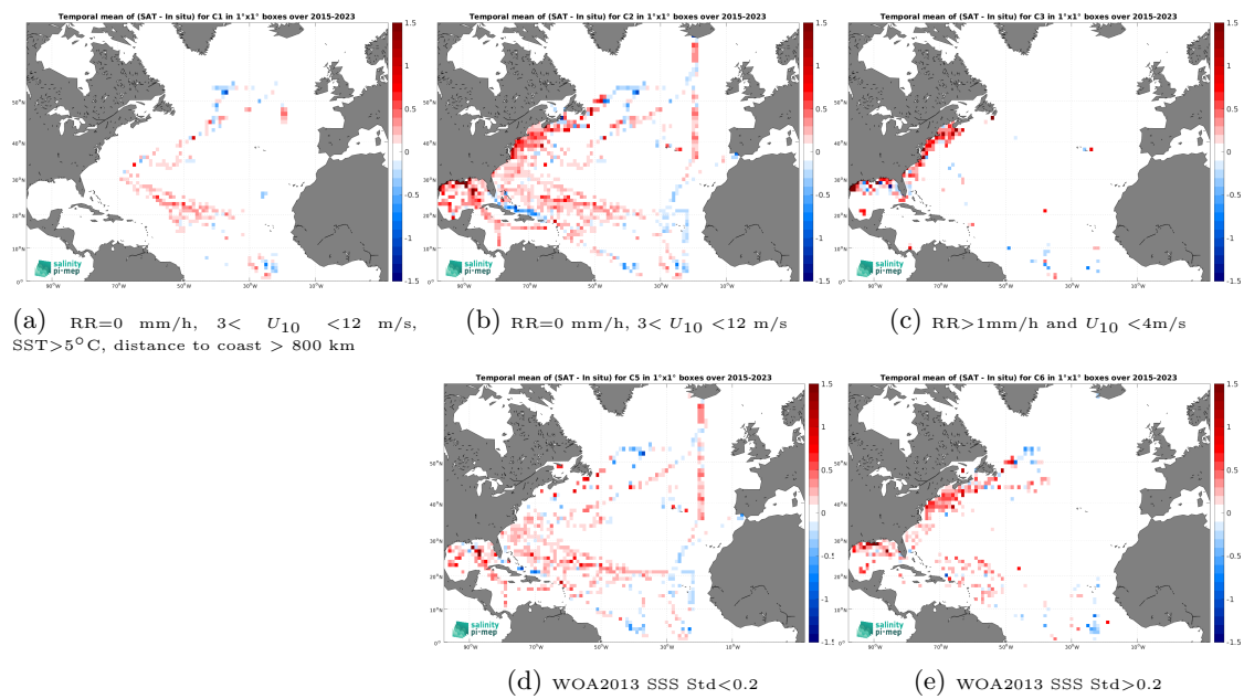
Figure 14: Temporal mean gridded over spatial boxes of size 1^\circ \times 1^\circ of \Delta\text{SSS} (SMAP SSS L3 v5.3 - 8-Day running (RSS) - TSG (SAMOS)) for 5 different subdatasets corresponding to:RR=0 mm/h, 3 < U_{10} < 12 m/s, SST >5^\circ\text{C} , distance to coast > 800 km (a), RR=0 mm/h, 3 < U_{10} < 12 m/s (b), RR >1 mm/h and U_{10} < 4 m/s (c), WOA2013 SSS Std <0.2 (d), WOA2013 SSS Std >0.2 (e).
