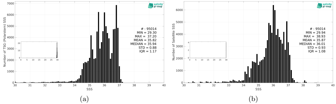
Figure 3: Histograms of SSS from TSG (Polarstern) (a) and SMAP SSS L3 v5.3 - 8-Day running (RSS) (b) considering all match-up pairs per bins of 0.1 over the North Atlantic Ocean Pi-MEP region and for the full satellite product period.
