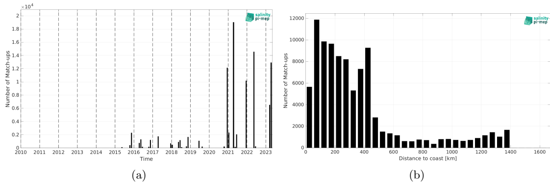
Figure 2: Number of match-ups between TSG (Polarstern) and SMAP SSS L3 v5.3 - 8-Day running (RSS) SSS as a function of time (a) and as function of the distance to coast (b) over the North Atlantic Ocean Pi-MEP region and for the full satellite product period.
