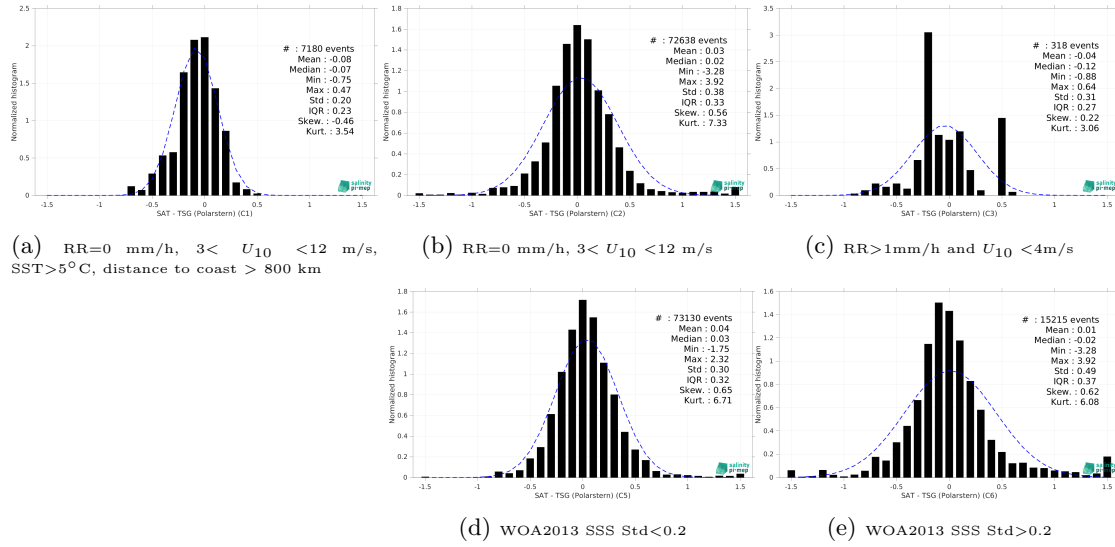
Figure 15: Normalized histogram of \Delta SSS (SMAP SSS L3 v5.3 - 8-Day running (RSS) - TSG (Polarstern)) for 5 different subdatasets corresponding to: RR=0 mm/h, 3 < U_{10} < 12 m/s, SST > 5°C, distance to coast > 800 km (a), RR=0 mm/h, 3 < U_{10} < 12 m/s (b), RR > 1mm/h and U_{10} < 4 m/s (c), WOA2013 SSS Std < 0.2 (d), WOA2013 SSS Std > 0.2 (e).
