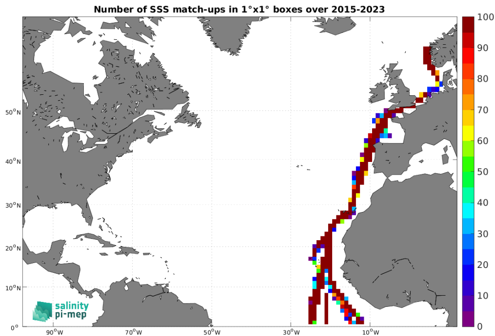
Figure 5: Number of SSS match-ups between TSG (Polarstern) SSS and the SMAP SSS L3 v5.3 - 8-Day running (RSS) SSS product for the North Atlantic Ocean Pi-MEP region over 1^\circ \times 1^\circ boxes and for the full satellite product period.
