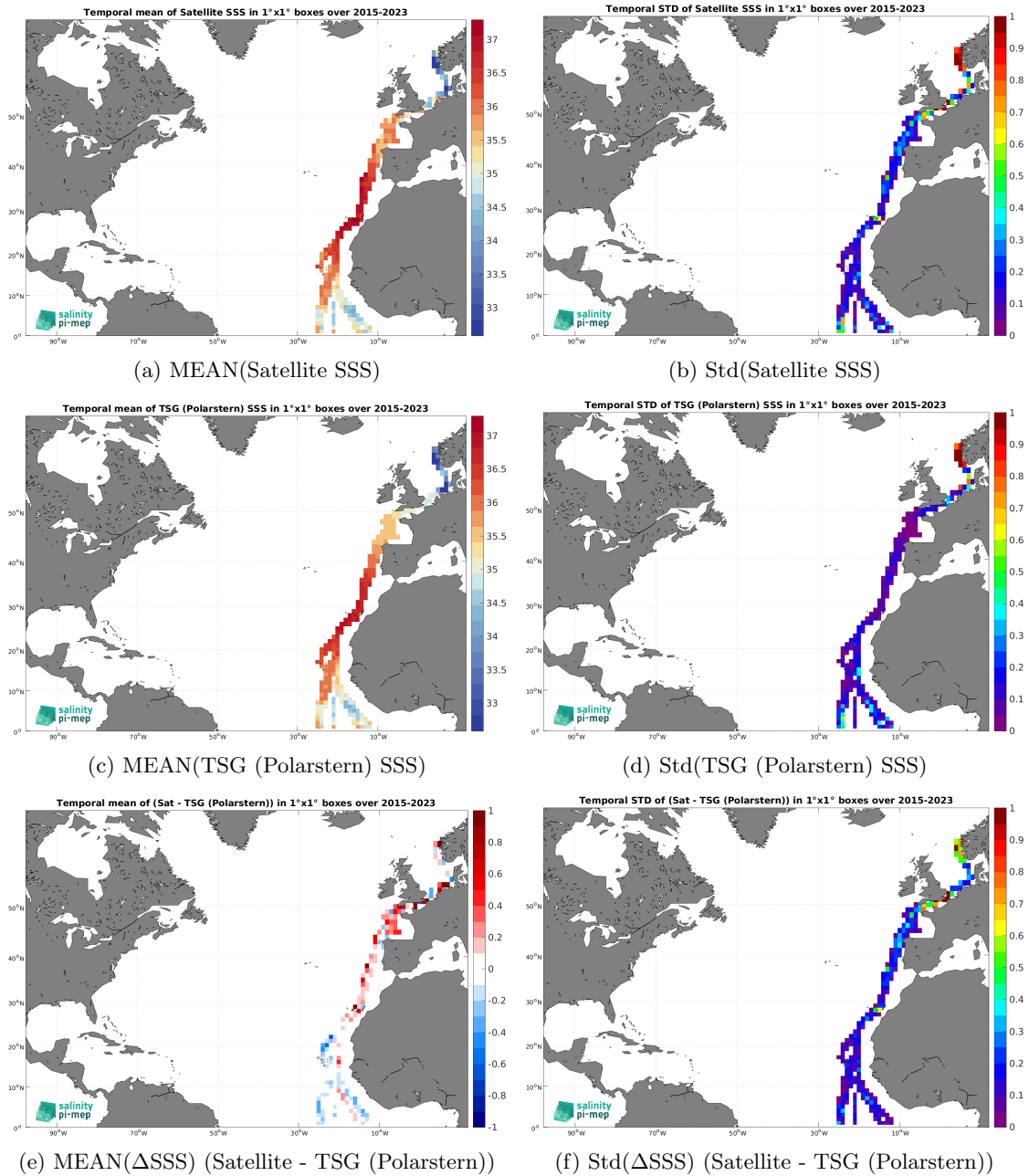
Figure 7: Temporal mean (left) and Std (right) of SSS from SMAP SSS L3 v5.3 - 8-Day running (RSS) (top), TSG (Polarstern) (middle), and of \Delta SSS (Satellite - TSG (Polarstern)). Only match-up pairs are used to generate these maps.
