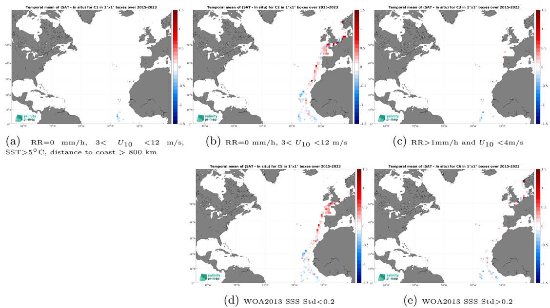
Figure 14: Temporal mean gridded over spatial boxes of size 1^\circ \times 1^\circ of \Delta\text{SSS} (SMAP SSS L3 v5.3 - 8-Day running (RSS) - TSG (Polarstern)) for 5 different subdatasets corresponding to:RR=0 mm/h, 3 < U_{10} < 12 m/s, SST >5^\circ\text{C} , distance to coast > 800 km (a), RR=0 mm/h, 3 < U_{10} < 12 m/s (b), RR >1 mm/h and U_{10} < 4 m/s (c), WOA2013 SSS Std <0.2 (d), WOA2013 SSS Std >0.2 (e).
