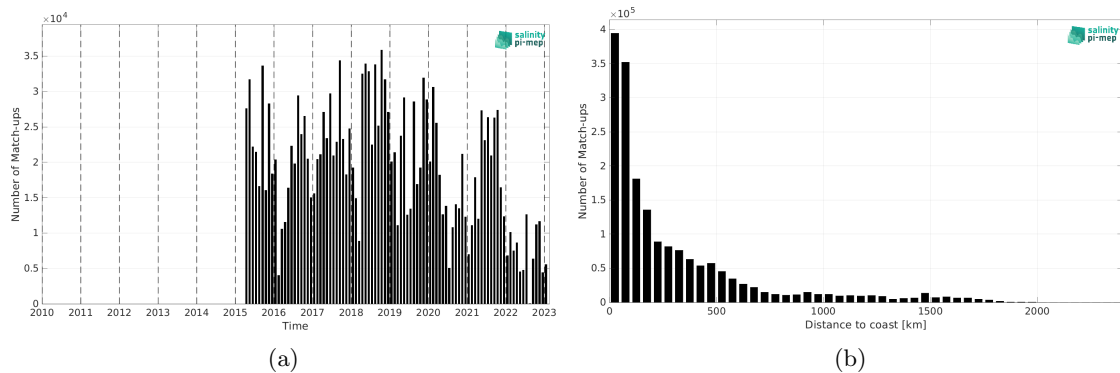
Figure 2: Number of match-ups between TSG (LEGOS-DM) and SMAP SSS L3 v5.3 - 8-Day running (RSS) SSS as a function of time (a) and as function of the distance to coast (b) over the North Atlantic Ocean Pi-MEP region and for the full satellite product period.
