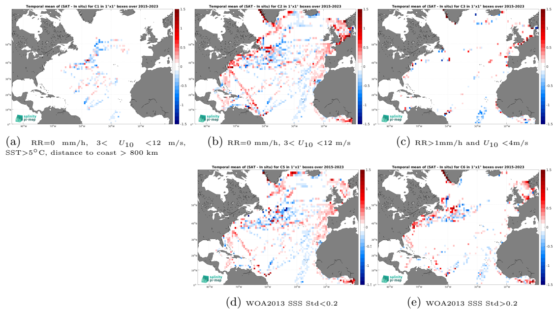
Figure 14: Temporal mean gridded over spatial boxes of size 1^\circ \times 1^\circ of \Delta\text{SSS} (SMAP SSS L3 v5.3 - 8-Day running (RSS) - TSG (LEGOS-DM)) for 5 different subdatasets corresponding to:RR=0 mm/h, 3 < U_{10} < 12 m/s, SST >5^\circ\text{C} , distance to coast > 800 km (a), RR=0 mm/h, 3 < U_{10} < 12 m/s (b), RR >1 mm/h and U_{10} < 4 m/s (c), WOA2013 SSS Std <0.2 (d), WOA2013 SSS Std >0.2 (e).
