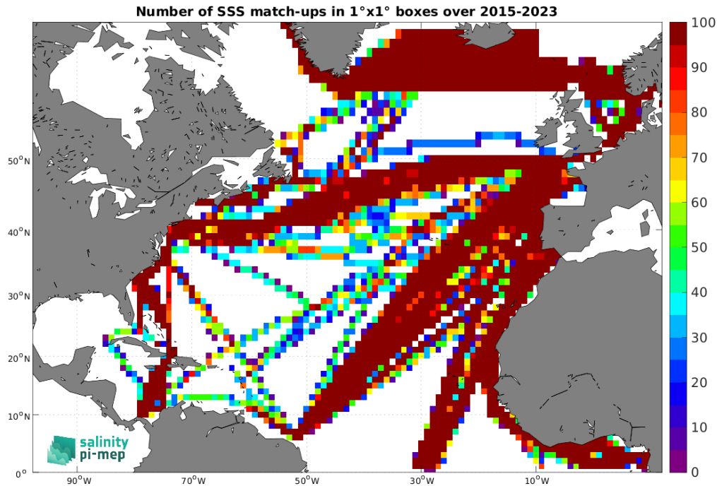
Figure 5: Number of SSS match-ups between TSG (LEGOS-DM) SSS and the SMAP SSS L3 v5.3 - 8-Day running (RSS) SSS product for the North Atlantic Ocean Pi-MEP region over 1^\circ \times 1^\circ boxes and for the full satellite product period.
