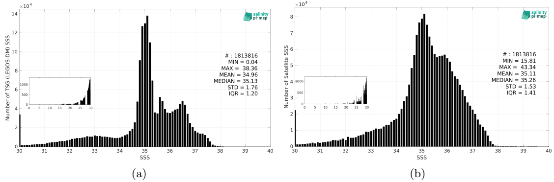
Figure 3: Histograms of SSS from TSG (LEGOS-DM) (a) and SMAP SSS L3 v5.3 - 8-Day running (RSS) (b) considering all match-up pairs per bins of 0.1 over the North Atlantic Ocean Pi-MEP region and for the full satellite product period.
