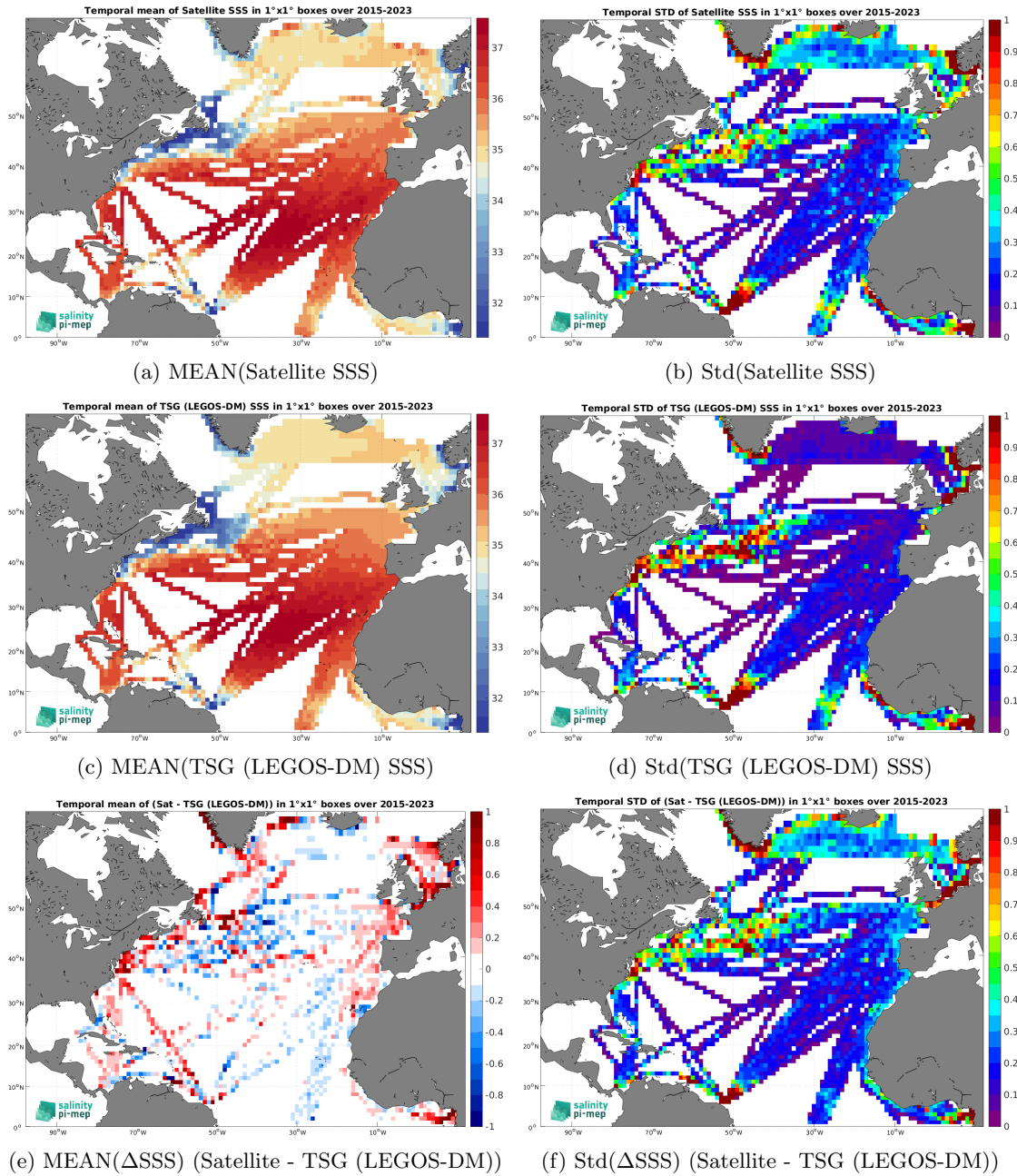
Figure 7: Temporal mean (left) and Std (right) of SSS from SMAP SSS L3 v5.3 - 8-Day running (RSS) (top), TSG (LEGOS-DM) (middle), and of \Delta SSS (Satellite - TSG (LEGOS-DM)). Only match-up pairs are used to generate these maps.
