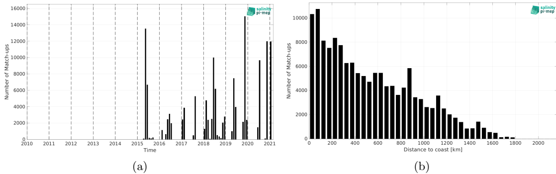
Figure 2: Number of match-ups between TSG (GOSUD-Sailing-ship) and SMAP SSS L3 v5.3 - 8-Day running (RSS) SSS as a function of time (a) and as function of the distance to coast (b) over the North Atlantic Ocean Pi-MEP region and for the full satellite product period.
