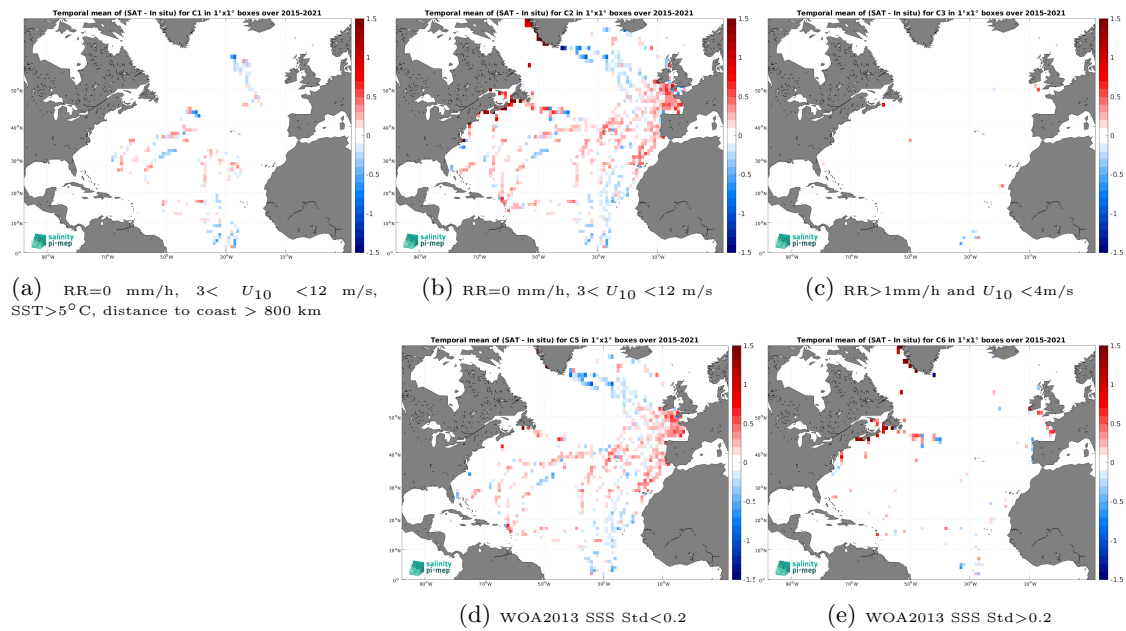
Figure 14: Temporal mean gridded over spatial boxes of size 1^\circ \times 1^\circ of \Delta\text{SSS} (SMAP SSS L3 v5.3 - 8-Day running (RSS) - TSG (GOSUD-Sailing-ship)) for 5 different subdatasets corresponding to:RR=0 mm/h, 3 < U_{10} < 12 m/s, SST>5°C, distance to coast > 800 km (a), RR=0 mm/h, 3 < U_{10} < 12 m/s (b), RR>1mm/h and U_{10} < 4 m/s (c), WOA2013 SSS Std<0.2 (d), WOA2013 SSS Std>0.2 (e).
