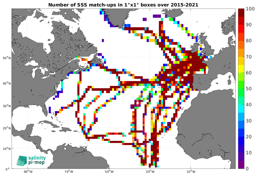
Figure 5: Number of SSS match-ups between TSG (GOSUD-Sailing-ship) SSS and the SMAP SSS L3 v5.3 - 8-Day running (RSS) SSS product for the North Atlantic Ocean Pi-MEP region over 1^\circ \times 1^\circ boxes and for the full satellite product period.
