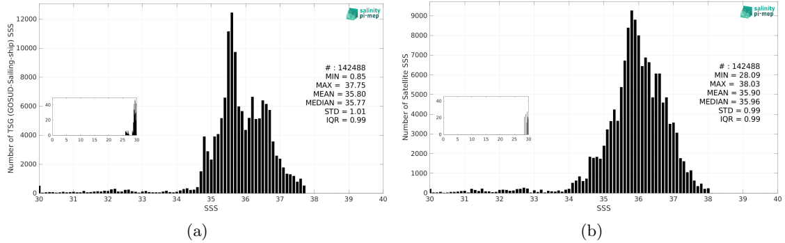
Figure 3: Histograms of SSS from TSG (GOSUD-Sailing-ship) (a) and SMAP SSS L3 v5.3 - 8-Day running (RSS) (b) considering all match-up pairs per bins of 0.1 over the North Atlantic Ocean Pi-MEP region and for the full satellite product period.
