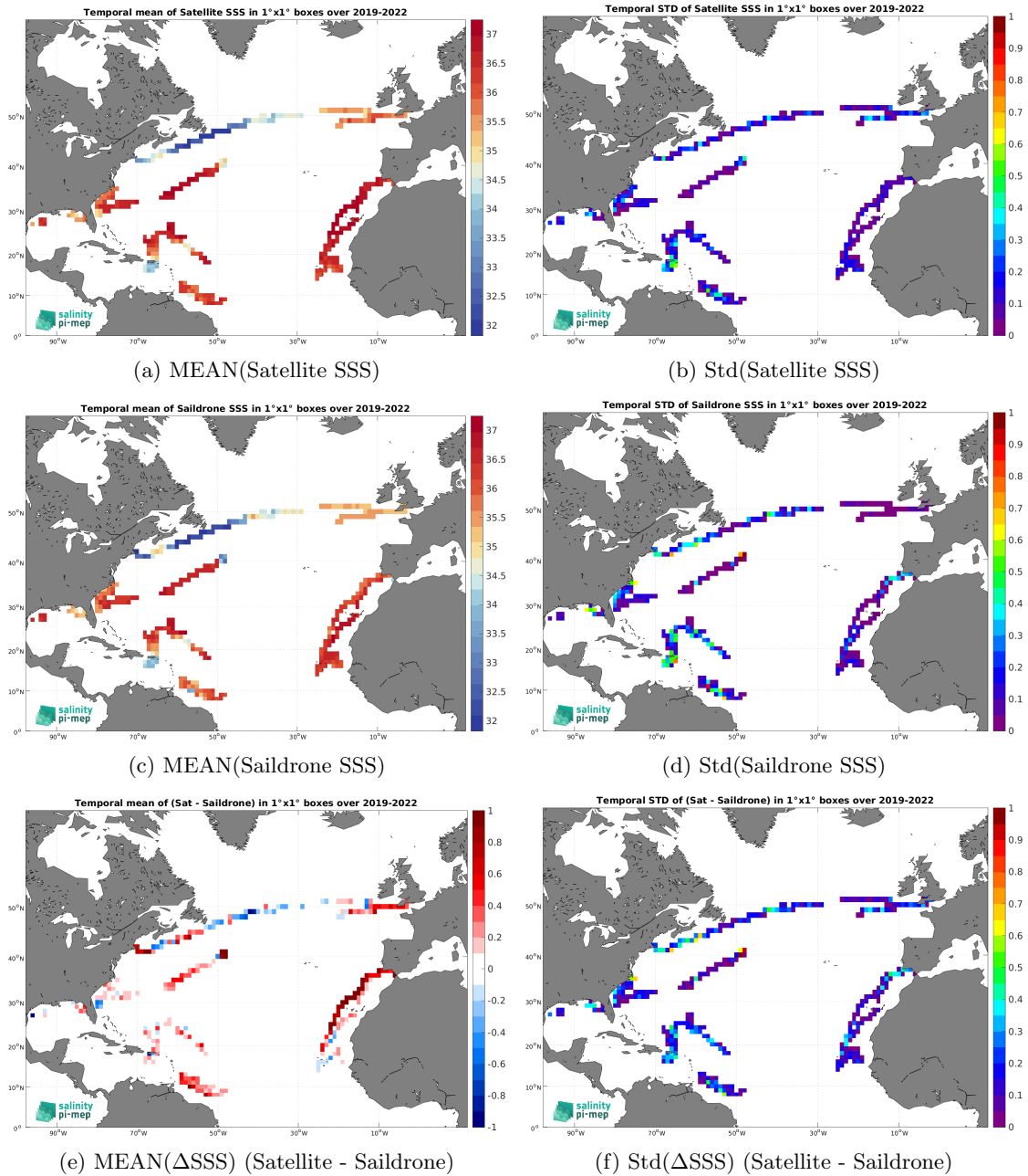
Figure 7: Temporal mean (left) and Std (right) of SSS from SMAP SSS L3 v5.3 - 8-Day running (RSS) (top), Saildrone (middle), and of \Delta SSS (Satellite - Saildrone). Only match-up pairs are used to generate these maps.
