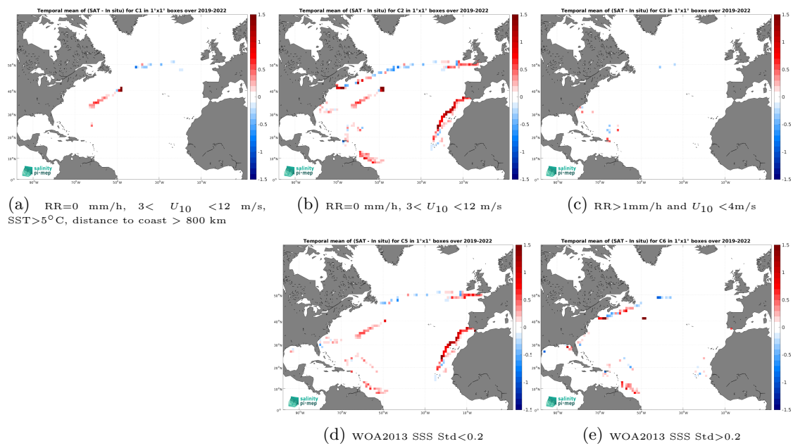
Figure 14: Temporal mean gridded over spatial boxes of size 1^\circ \times 1^\circ of \Delta\text{SSS} (SMAP SSS L3 v5.3 - 8-Day running (RSS) - Saifdrone) for 5 different subdatasets corresponding to:RR=0 mm/h, 3 < U_{10} < 12 m/s, SST >5^\circ\text{C} , distance to coast > 800 km (a), RR=0 mm/h, 3 < U_{10} < 12 m/s (b), RR >1 mm/h and U_{10} < 4 m/s (c), WOA2013 SSS Std <0.2 (d), WOA2013 SSS Std >0.2 (e).
