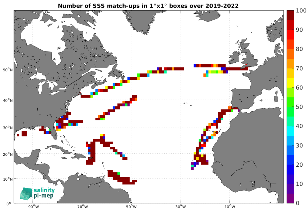
Figure 5: Number of SSS match-ups between Saildrone SSS and the SMAP SSS L3 v5.3 - 8-Day running (RSS) SSS product for the North Atlantic Ocean Pi-MEP region over 1^\circ \times 1^\circ boxes and for the full satellite product period.
