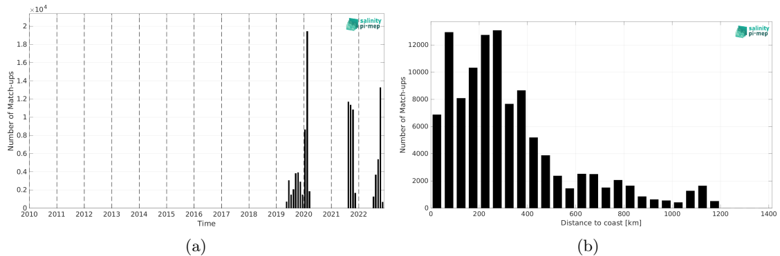
Figure 2: Number of match-ups between Saildrone and SMAP SSS L3 v5.3 - 8-Day running (RSS) SSS as a function of time (a) and as function of the distance to coast (b) over the North Atlantic Ocean Pi-MEP region and for the full satellite product period.
