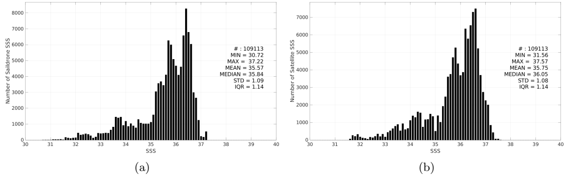
Figure 3: Histograms of SSS from Saildrone (a) and SMAP SSS L3 v5.3 - 8-Day running (RSS) (b) considering all match-up pairs per bins of 0.1 over the North Atlantic Ocean Pi-MEP region and for the full satellite product period.
