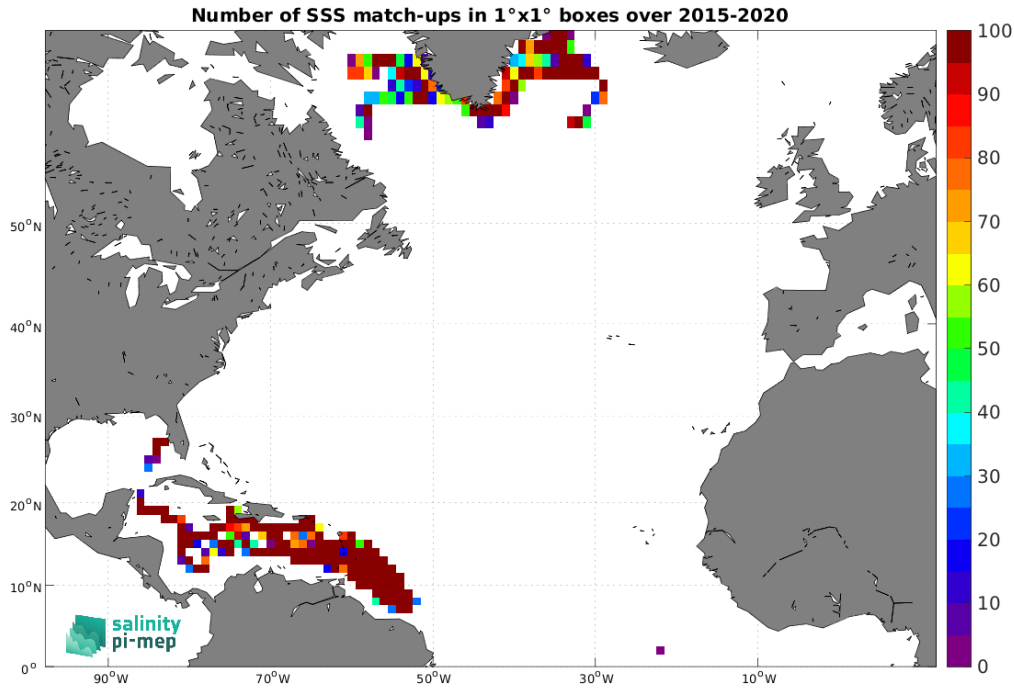
Figure 4: Number of SSS match-ups between Surface drifters SSS and the SMAP SSS L3 v5.3 - 8-Day running (RSS) SSS product for the North Atlantic Ocean Pi-MEP region over 1^\circ \times 1^\circ boxes and for the full satellite product period.
