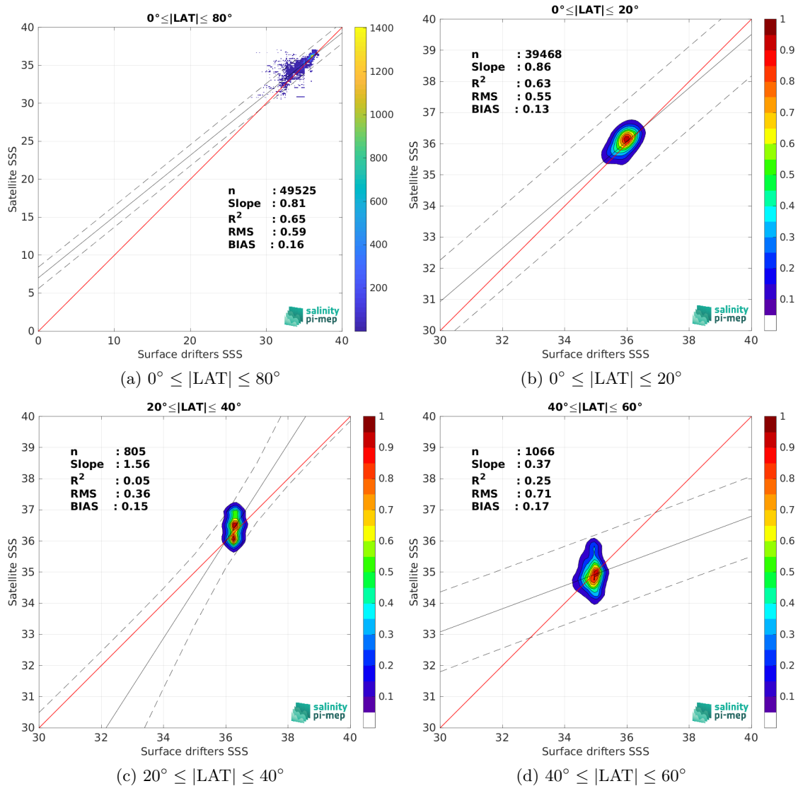
Figure 9: Contour maps of the concentration of SMAP SSS L3 v5.3 - 8-Day running (RSS) SSS (y-axis) versus Surface drifters SSS (x-axis) at match-up pairs for different latitude bands. For each plot, the red line shows x=y . The black thin and dashed lines indicate a linear fit through the data cloud and the \pm 95\% confidence levels, respectively. The number match-up pairs n , the slope and R^2 coefficient of the linear fit, the root mean square (RMS) and the mean bias between satellite and in situ data are indicated for each latitude band in each plots.
