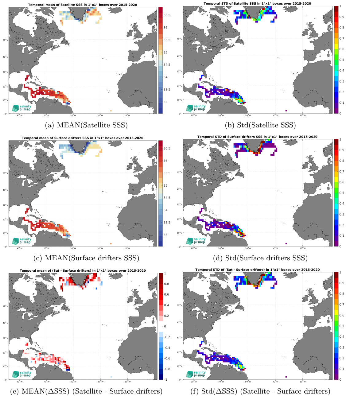
Figure 6: Temporal mean (left) and Std (right) of SSS from SMAP SSS L3 v5.3 - 8-Day running (RSS) (top), Surface drifters (middle), and of \Delta SSS (Satellite - Surface drifters). Only match-up pairs are used to generate these maps.
