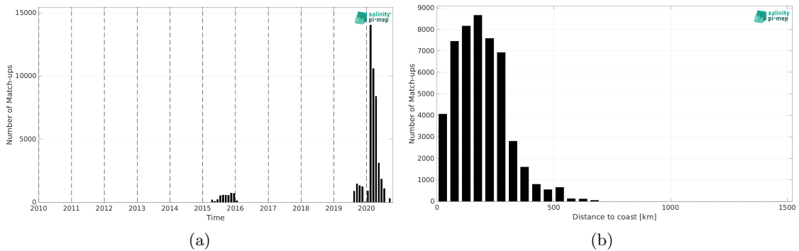
Figure 2: Number of match-ups between Surface drifters and SMAP SSS L3 v5.3 - 8-Day running (RSS) SSS as a function of time (a) and as function of the distance to coast (b) over the North Atlantic Ocean Pi-MEP region and for the full satellite product period.
