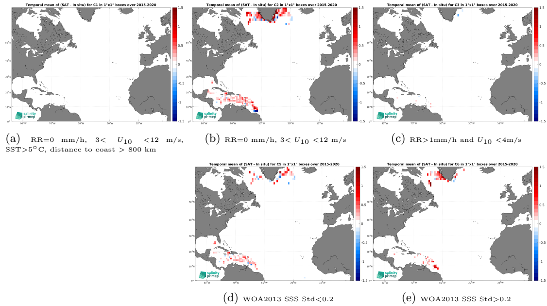
Figure 13: Temporal mean gridded over spatial boxes of size 1^\circ \times 1^\circ of \Delta\text{SSS} (SMAP SSS L3 v5.3 - 8-Day running (RSS) - Surface drifters) for 5 different subdatasets corresponding to:RR=0 mm/h, 3 < U_{10} < 12 m/s, SST > 5^\circ\text{C} , distance to coast > 800 km (a), RR=0 mm/h, 3 < U_{10} < 12 m/s (b), RR > 1 mm/h and U_{10} < 4 m/s (c), WOA2013 SSS Std < 0.2 (d), WOA2013 SSS Std > 0.2 (e).
