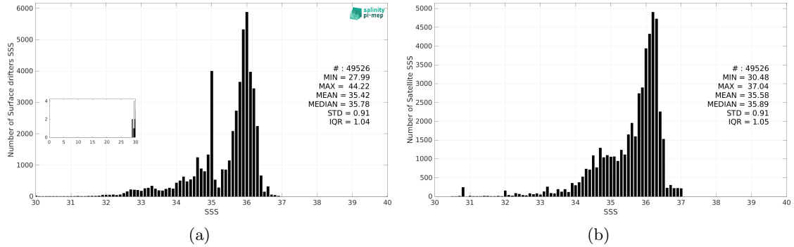
Figure 3: Histograms of SSS from Surface drifters (a) and SMAP SSS L3 v5.3 - 8-Day running (RSS) (b) considering all match-up pairs per bins of 0.1 over the North Atlantic Ocean Pi-MEP region and for the full satellite product period.
