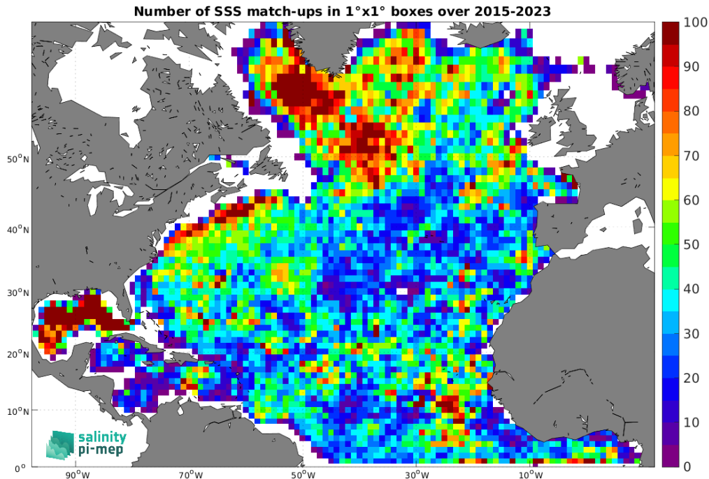
Figure 5: Number of SSS match-ups between Argo SSS and the SMAP SSS L3 v5.3 - 8-Day running (RSS) SSS product for the North Atlantic Ocean Pi-MEP region over 1^\circ \times 1^\circ boxes and for the full satellite product period.
