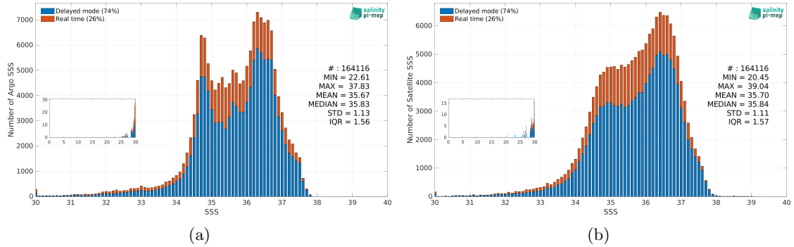
Figure 3: Histograms of SSS from Argo (a) and SMAP SSS L3 v5.3 - 8-Day running (RSS) (b) considering all match-up pairs per bins of 0.1 over the North Atlantic Ocean Pi-MEP region and for the full satellite product period.
