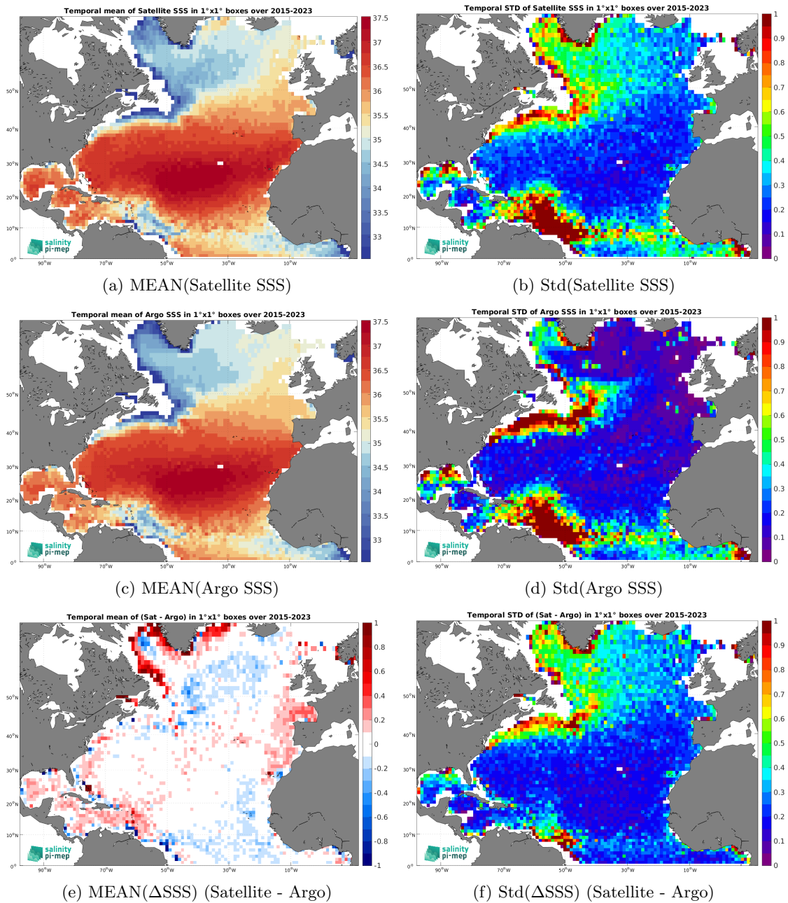
Figure 7: Temporal mean (left) and Std (right) of SSS from SMAP SSS L3 v5.3 - 8-Day running (RSS) (top), Argo (middle), and of \Delta SSS (Satellite - Argo). Only match-up pairs are used to generate these maps.
