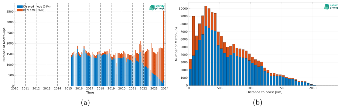
Figure 2: Number of match-ups between Argo and SMAP SSS L3 v5.3 - 8-Day running (RSS) SSS as a function of time (a) and as function of the distance to coast (b) over the North Atlantic Ocean Pi-MEP region and for the full satellite product period.
