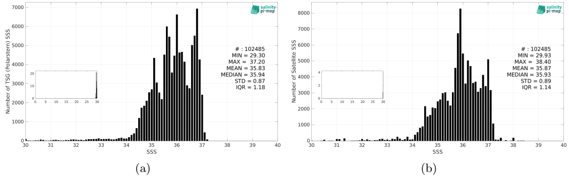
Figure 3: Histograms of SSS from TSG (Polarstern) (a) and SMAP SSS L3 v5.3 - Monthly (RSS) (b) considering all match-up pairs per bins of 0.1 over the North Atlantic Ocean Pi-MEP region and for the full satellite product period.
