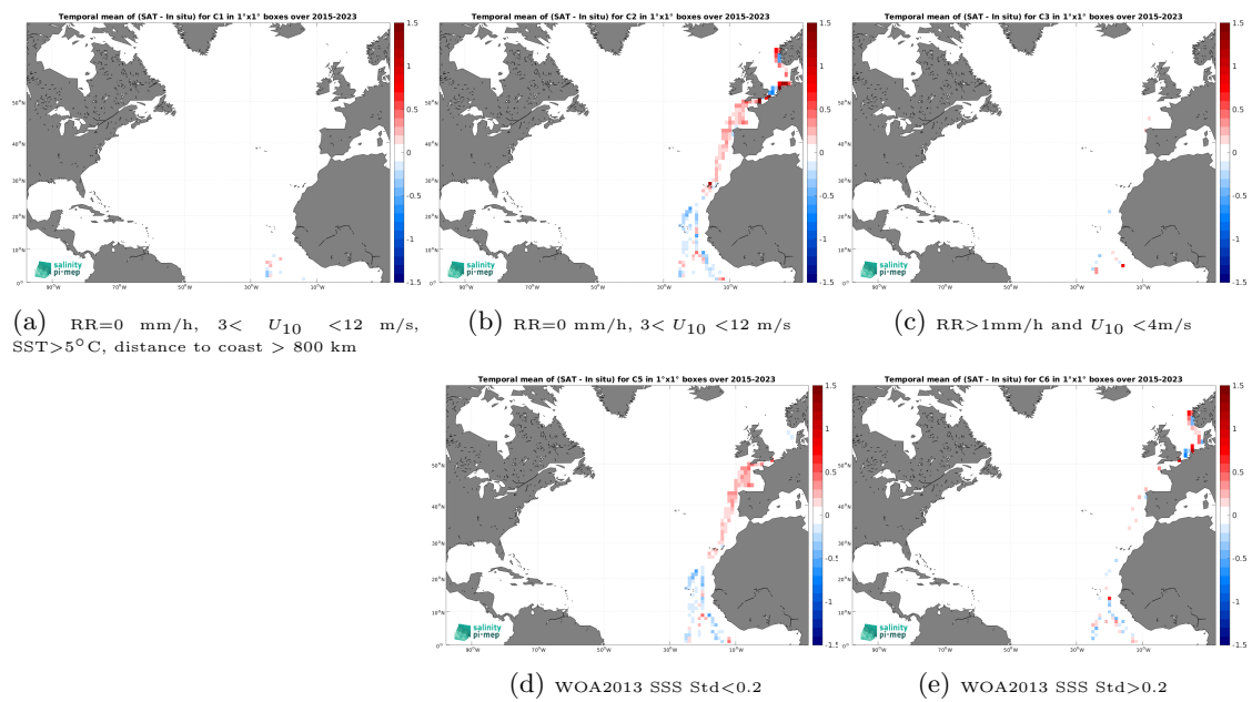
Figure 14: Temporal mean gridded over spatial boxes of size 1^\circ \times 1^\circ of \Delta\text{SSS} (SMAP SSS L3 v5.3 - Monthly (RSS) - TSG (Polarstern)) for 5 different subdatasets corresponding to:RR=0 mm/h, 3 < U_{10} < 12 m/s, SST > 5^\circ\text{C} , distance to coast > 800 km (a), RR=0 mm/h, 3 < U_{10} < 12 m/s (b), RR > 1 mm/h and U_{10} < 4 m/s (c), WOA2013 SSS Std < 0.2 (d), WOA2013 SSS Std > 0.2 (e).
