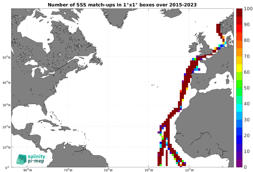
Figure 5: Number of SSS match-ups between TSG (Polarstern) SSS and the SMAP SSS L3 v5.3 - Monthly (RSS) SSS product for the North Atlantic Ocean Pi-MEP region over 1^\circ \times 1^\circ boxes and for the full satellite product period.
