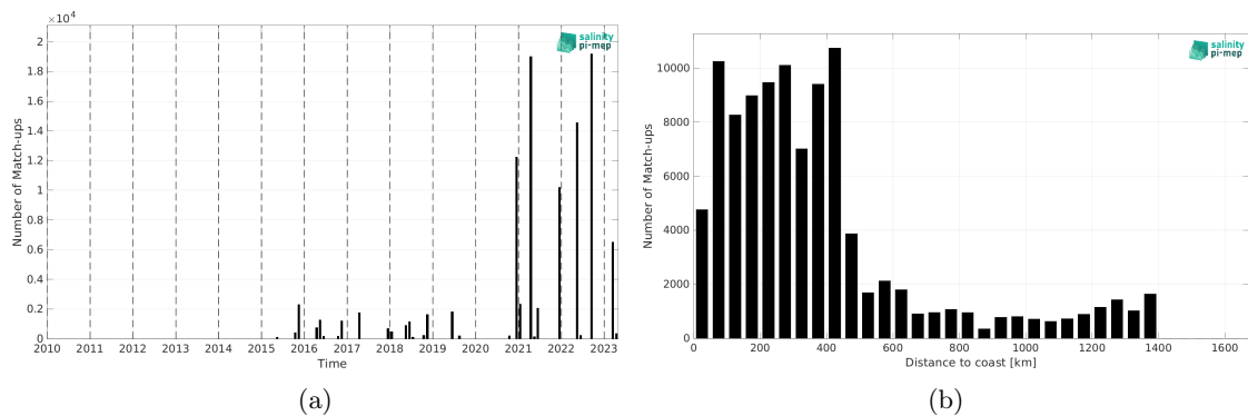
Figure 2: Number of match-ups between TSG (Polarstern) and SMAP SSS L3 v5.3 - Monthly (RSS) SSS as a function of time (a) and as function of the distance to coast (b) over the North Atlantic Ocean Pi-MEP region and for the full satellite product period.
