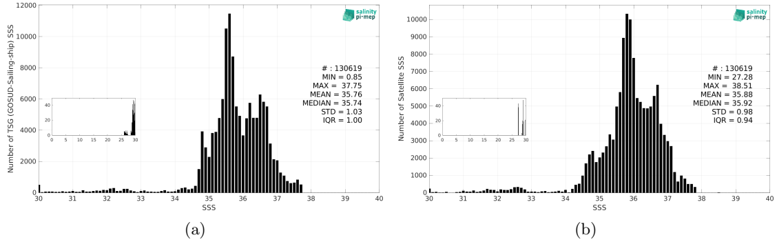
Figure 3: Histograms of SSS from TSG (GOSUD-Sailing-ship) (a) and SMAP SSS L3 v5.3 - Monthly (RSS) (b) considering all match-up pairs per bins of 0.1 over the North Atlantic Ocean Pi-MEP region and for the full satellite product period.
