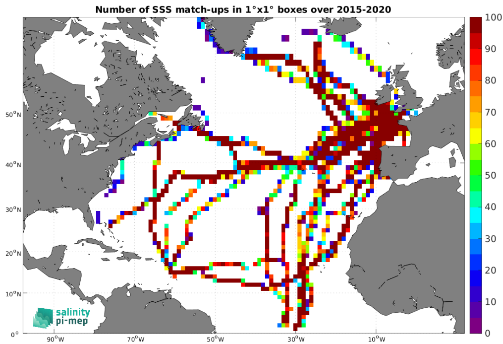
Figure 5: Number of SSS match-ups between TSG (GOSUD-Sailing-ship) SSS and the SMAP SSS L3 v5.3 - Monthly (RSS) SSS product for the North Atlantic Ocean Pi-MEP region over 1^\circ \times 1^\circ boxes and for the full satellite product period.
