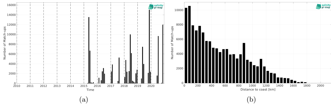
Figure 2: Number of match-ups between TSG (GOSUD-Sailing-ship) and SMAP SSS L3 v5.3 - Monthly (RSS) SSS as a function of time (a) and as function of the distance to coast (b) over the North Atlantic Ocean Pi-MEP region and for the full satellite product period.
