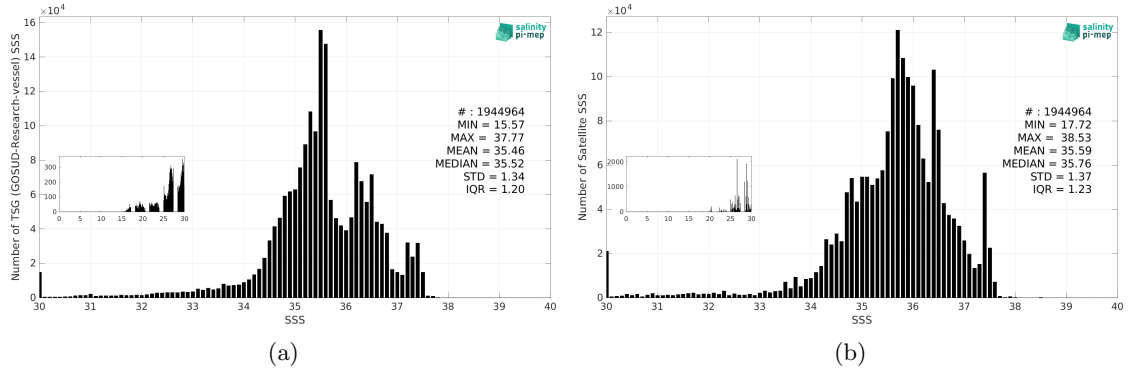
Figure 3: Histograms of SSS from TSG (GOSUD-Research-vessel) (a) and SMAP SSS L3 v5.3 - Monthly (RSS) (b) considering all match-up pairs per bins of 0.1 over the North Atlantic Ocean Pi-MEP region and for the full satellite product period.
