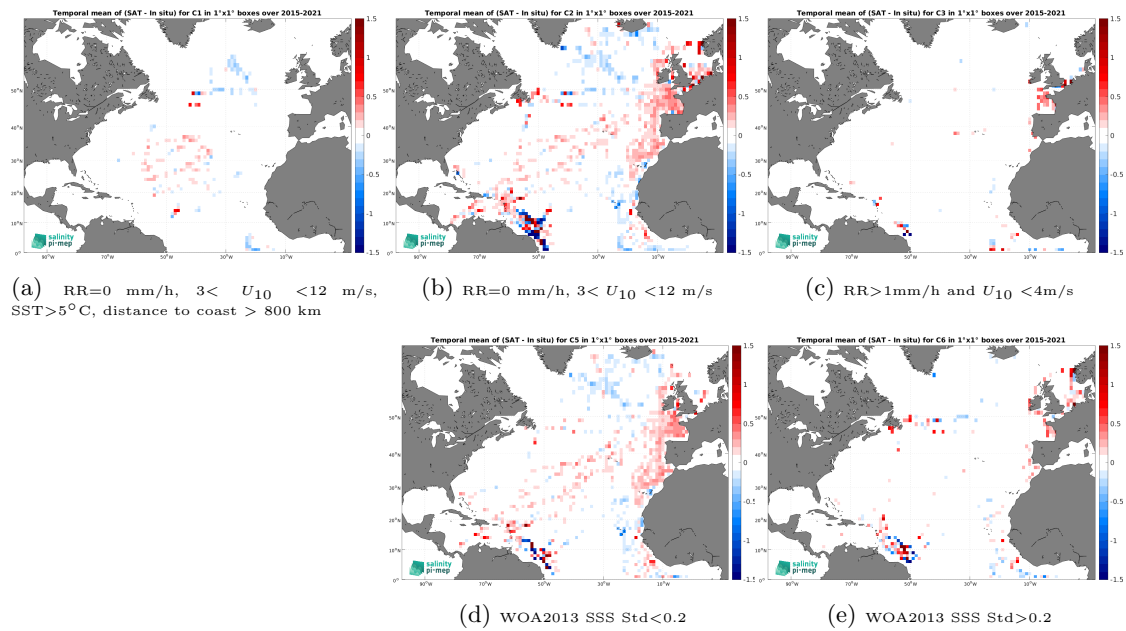
Figure 14: Temporal mean gridded over spatial boxes of size 1^\circ \times 1^\circ of \Delta\text{SSS} (SMAP SSS L3 v5.3 - Monthly (RSS) - TSG (GOSUD-Research-vessel)) for 5 different subdatasets corresponding to:RR=0 mm/h, 3 < U_{10} < 12 m/s, SST > 5°C, distance to coast > 800 km (a), RR=0 mm/h, 3 < U_{10} < 12 m/s (b), RR > 1mm/h and U_{10} < 4 m/s (c), WOA2013 SSS Std < 0.2 (d), WOA2013 SSS Std > 0.2 (e).
