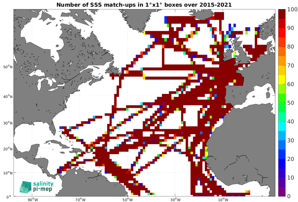
Figure 5: Number of SSS match-ups between TSG (GOSUD-Research-vessel) SSS and the SMAP SSS L3 v5.3 - Monthly (RSS) SSS product for the North Atlantic Ocean Pi-MEP region over 1^\circ \times 1^\circ boxes and for the full satellite product period.
