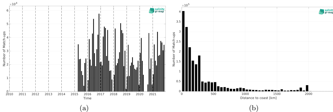
Figure 2: Number of match-ups between TSG (GOSUD-Research-vessel) and SMAP SSS L3 v5.3 - Monthly (RSS) SSS as a function of time (a) and as function of the distance to coast (b) over the North Atlantic Ocean Pi-MEP region and for the full satellite product period.
