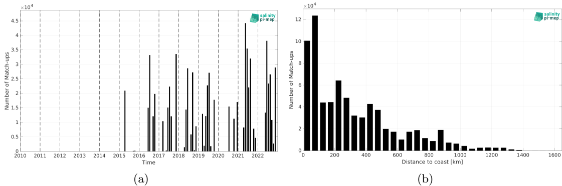
Figure 2: Number of match-ups between TSG (CSIC-UTM) and SMAP SSS L3 v5.3 - Monthly (RSS) SSS as a function of time (a) and as function of the distance to coast (b) over the North Atlantic Ocean Pi-MEP region and for the full satellite product period.
