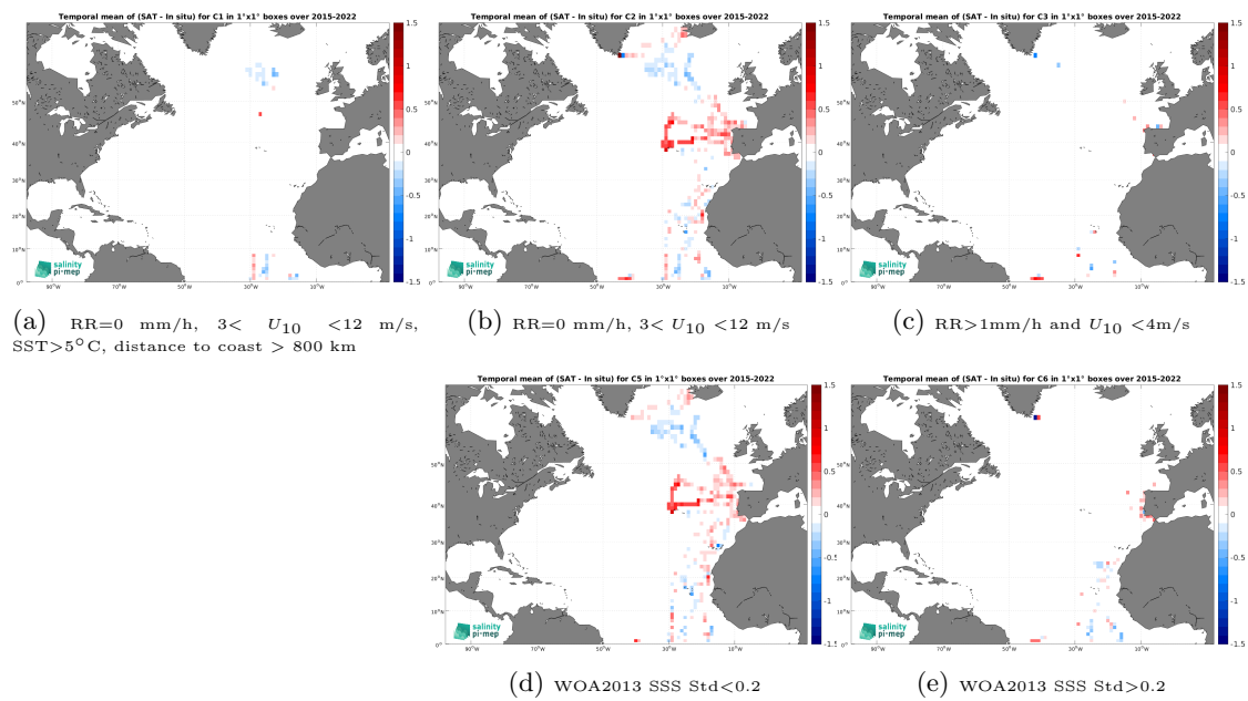
Figure 14: Temporal mean gridded over spatial boxes of size 1^\circ \times 1^\circ of \Delta\text{SSS} (SMAP SSS L3 v5.3 - Monthly (RSS) - TSG (CSIC-UTM)) for 5 different subdatasets corresponding to:RR=0 mm/h, 3 < U_{10} < 12 m/s, SST > 5°C, distance to coast > 800 km (a), RR=0 mm/h, 3 < U_{10} < 12 m/s (b), RR > 1mm/h and U_{10} < 4 m/s (c), WOA2013 SSS Std < 0.2 (d), WOA2013 SSS Std > 0.2 (e).
