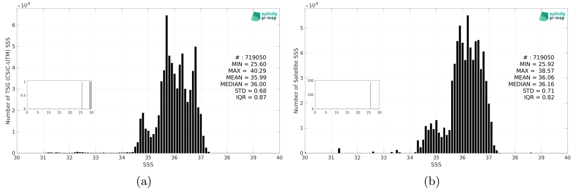
Figure 3: Histograms of SSS from TSG (CSIC-UTM) (a) and SMAP SSS L3 v5.3 - Monthly (RSS) (b) considering all match-up pairs per bins of 0.1 over the North Atlantic Ocean Pi-MEP region and for the full satellite product period.
