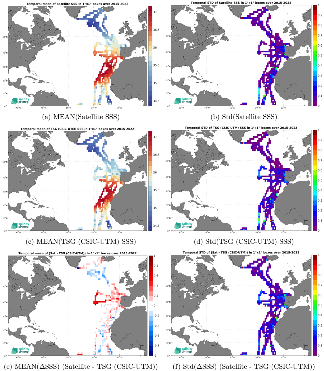
Figure 7: Temporal mean (left) and Std (right) of SSS from SMAP SSS L3 v5.3 - Monthly (RSS) (top), TSG (CSIC-UTM) (middle), and of \Delta SSS (Satellite - TSG (CSIC-UTM)). Only match-up pairs are used to generate these maps.
