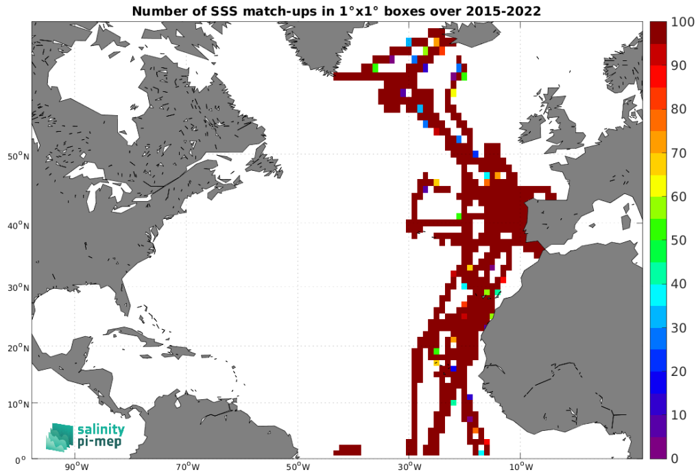
Figure 5: Number of SSS match-ups between TSG (CSIC-UTM) SSS and the SMAP SSS L3 v5.3 - Monthly (RSS) SSS product for the North Atlantic Ocean Pi-MEP region over 1^\circ \times 1^\circ boxes and for the full satellite product period.
