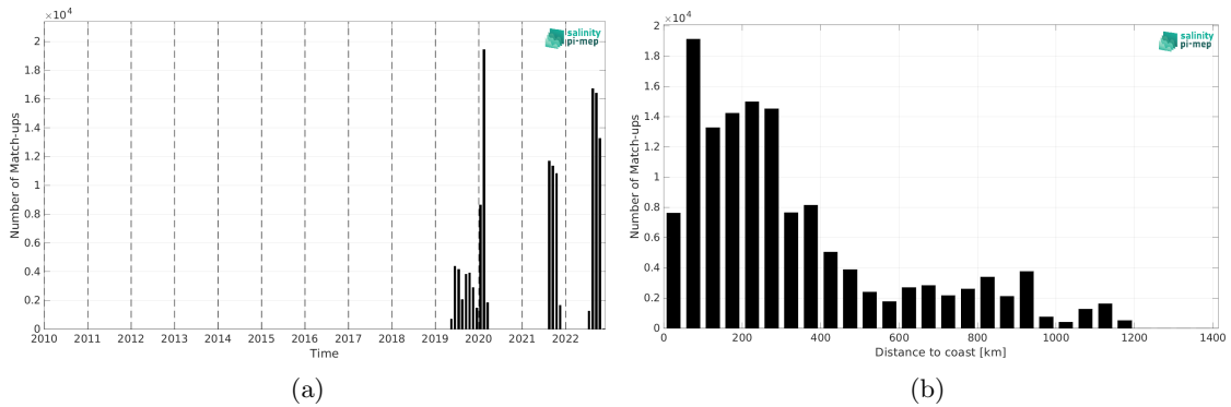
Figure 2: Number of match-ups between Saildrone and SMAP SSS L3 v5.3 - Monthly (RSS) SSS as a function of time (a) and as function of the distance to coast (b) over the North Atlantic Ocean Pi-MEP region and for the full satellite product period.
