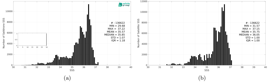
Figure 3: Histograms of SSS from Saildrone (a) and SMAP SSS L3 v5.3 - Monthly (RSS) (b) considering all match-up pairs per bins of 0.1 over the North Atlantic Ocean Pi-MEP region and for the full satellite product period.
