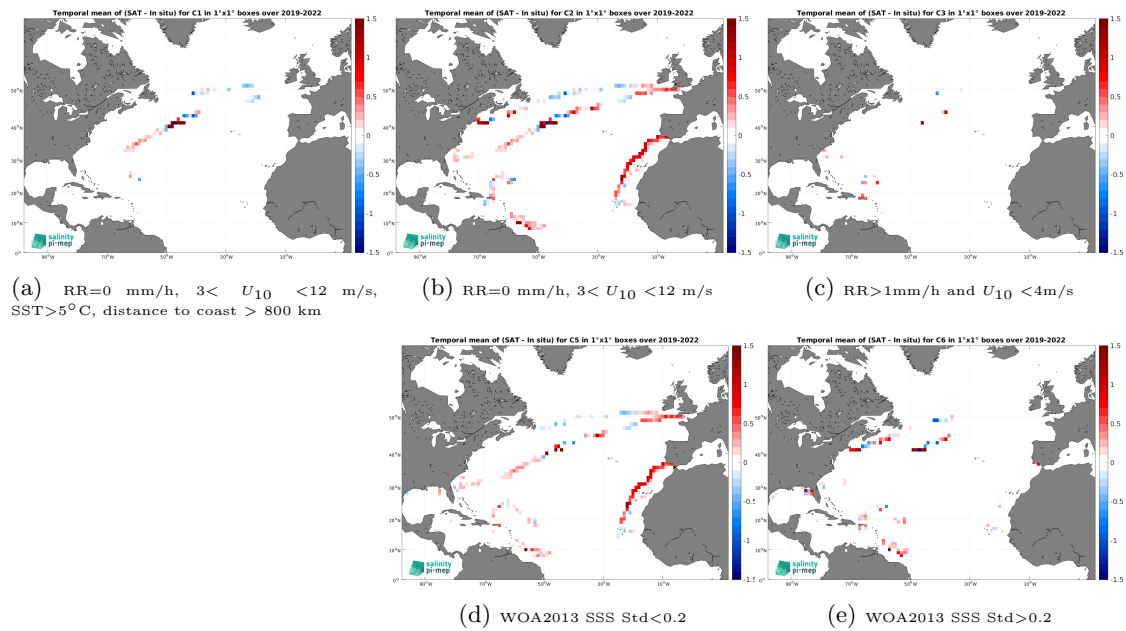
Figure 14: Temporal mean gridded over spatial boxes of size 1^\circ \times 1^\circ of \Delta\text{SSS} (SMAP SSS L3 v5.3 - Monthly (RSS) - Sairdrone) for 5 different subdatasets corresponding to:RR=0 mm/h, 3 < U_{10} < 12 m/s, SST > 5^\circ\text{C} , distance to coast > 800 km (a), RR=0 mm/h, 3 < U_{10} < 12 m/s (b), RR > 1 mm/h and U_{10} < 4 m/s (c), WOA2013 SSS Std < 0.2 (d), WOA2013 SSS Std > 0.2 (e).
