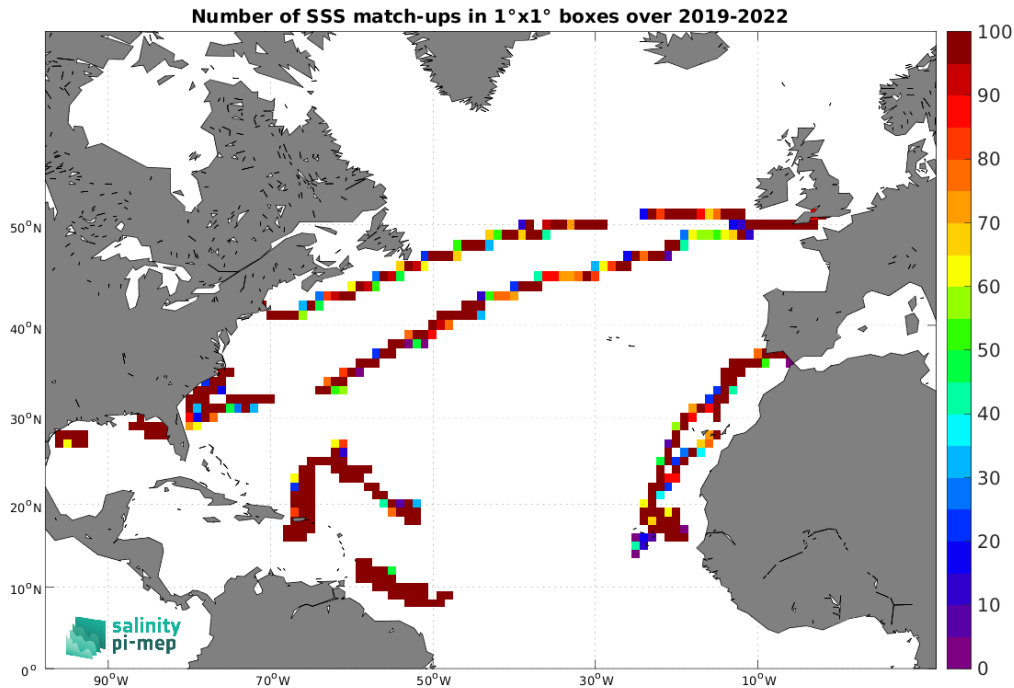
Figure 5: Number of SSS match-ups between Saildrone SSS and the SMAP SSS L3 v5.3 - Monthly (RSS) SSS product for the North Atlantic Ocean Pi-MEP region over 1^\circ \times 1^\circ boxes and for the full satellite product period.
