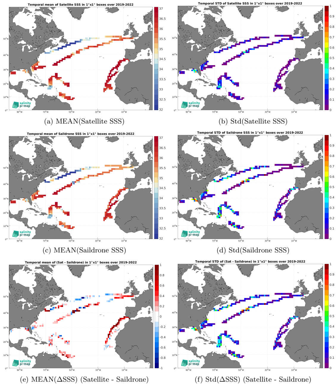
Figure 7: Temporal mean (left) and Std (right) of SSS from SMAP SSS L3 v5.3 - Monthly (RSS) (top), Saildrone (middle), and of \Delta SSS (Satellite - Saildrone). Only match-up pairs are used to generate these maps.
