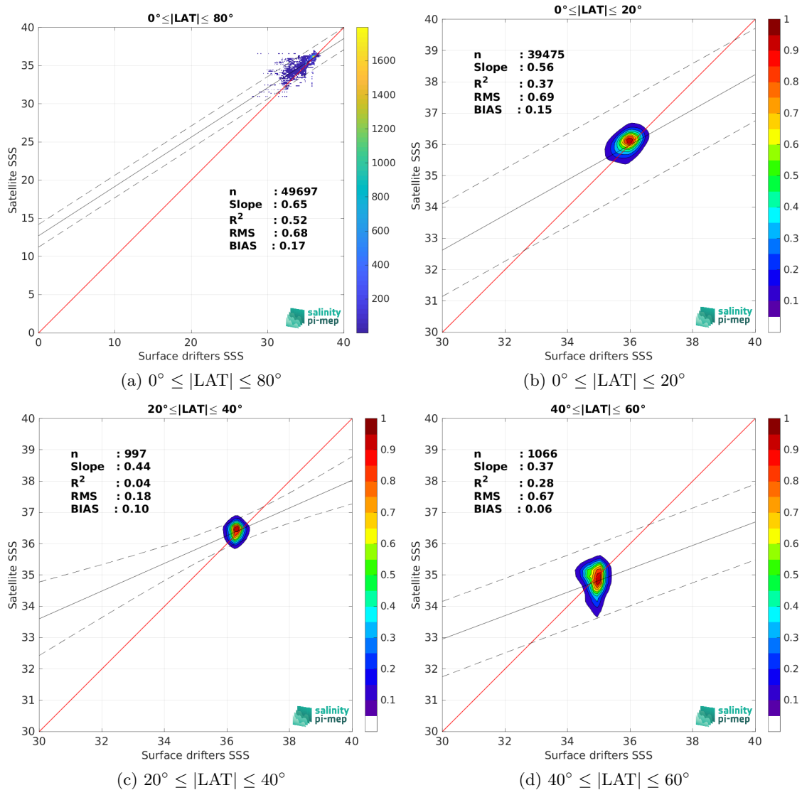
Figure 9: Contour maps of the concentration of SMAP SSS L3 v5.3 - Monthly (RSS) SSS (y-axis) versus Surface drifters SSS (x-axis) at match-up pairs for different latitude bands. For each plot, the red line shows x=y . The black thin and dashed lines indicate a linear fit through the data cloud and the \pm 95\% confidence levels, respectively. The number match-up pairs n , the slope and R^2 coefficient of the linear fit, the root mean square (RMS) and the mean bias between satellite and in situ data are indicated for each latitude band in each plots.
