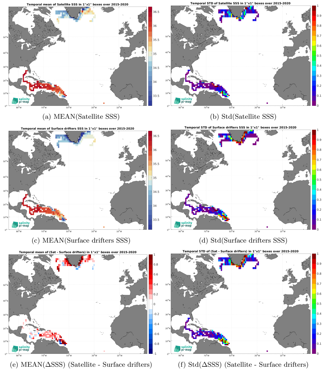
Figure 6: Temporal mean (left) and Std (right) of SSS from SMAP SSS L3 v5.3 - Monthly (RSS) (top), Surface drifters (middle), and of \Delta SSS (Satellite - Surface drifters). Only match-up pairs are used to generate these maps.
