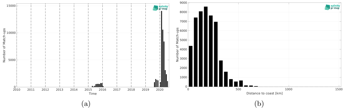
Figure 2: Number of match-ups between Surface drifters and SMAP SSS L3 v5.3 - Monthly (RSS) SSS as a function of time (a) and as function of the distance to coast (b) over the North Atlantic Ocean Pi-MEP region and for the full satellite product period.
