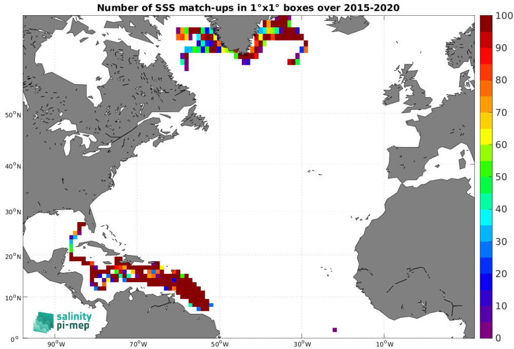
Figure 4: Number of SSS match-ups between Surface drifters SSS and the SMAP SSS L3 v5.3 - Monthly (RSS) SSS product for the North Atlantic Ocean Pi-MEP region over 1^\circ \times 1^\circ boxes and for the full satellite product period.
