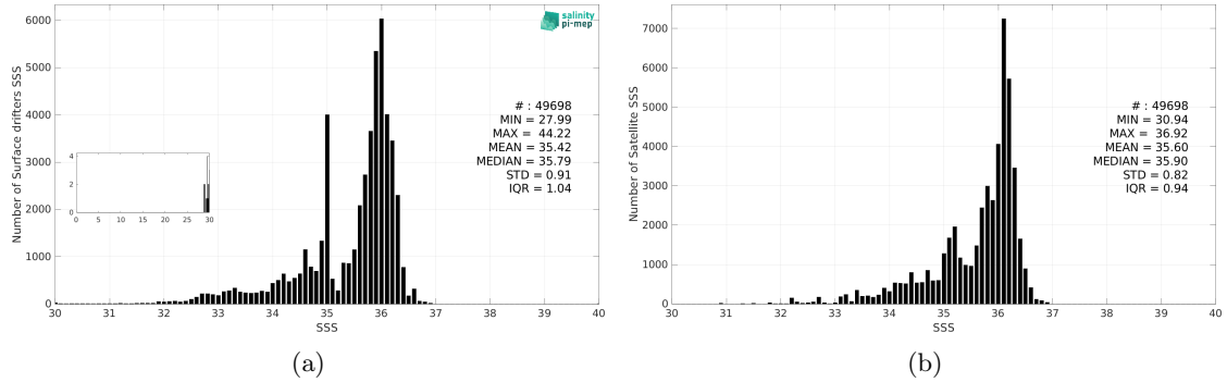
Figure 3: Histograms of SSS from Surface drifters (a) and SMAP SSS L3 v5.3 - Monthly (RSS) (b) considering all match-up pairs per bins of 0.1 over the North Atlantic Ocean Pi-MEP region and for the full satellite product period.
