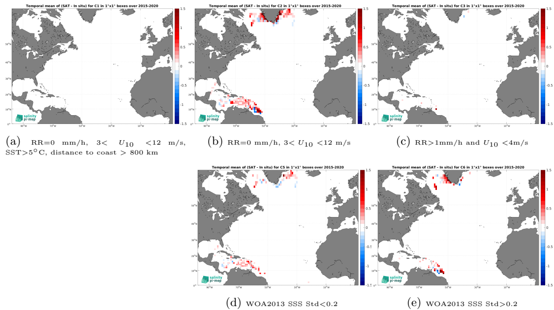
Figure 13: Temporal mean gridded over spatial boxes of size 1^\circ \times 1^\circ of \Delta\text{SSS} (SMAP SSS L3 v5.3 - Monthly (RSS) - Surface drifters) for 5 different subdatasets corresponding to:RR=0 mm/h, 3 < U_{10} < 12 m/s, SST >5^\circ\text{C} , distance to coast > 800 km (a), RR=0 mm/h, 3 < U_{10} < 12 m/s (b), RR >1 mm/h and U_{10} < 4 m/s (c), WOA2013 SSS Std <0.2 (d), WOA2013 SSS Std >0.2 (e).
