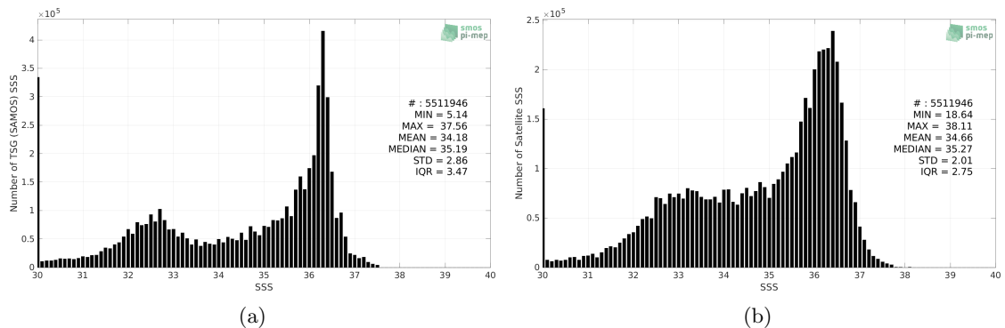
Figure 2: Histograms of SSS from TSG (SAMOS) (a) and SMAP SSS L3 v5 - 8-Day running (RSS) (b) considering all match-up pairs per bins of 0.1 over the North Atlantic Ocean Pi-MEP region and for the full satellite product period.
