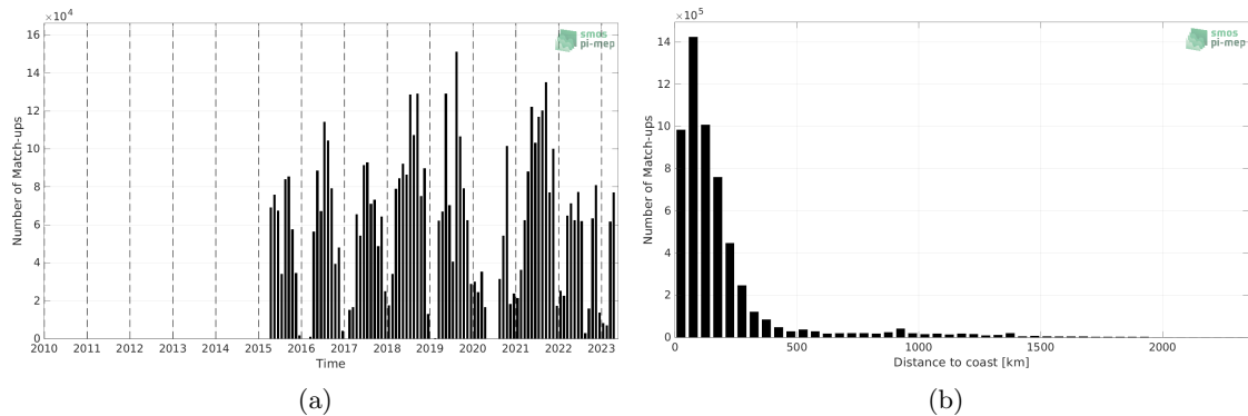
Figure 1: Number of match-ups between TSG (SAMOS) and SMAP SSS L3 v5 - 8-Day running (RSS) SSS as a function of time (a) and as function of the distance to coast (b) over the North Atlantic Ocean Pi-MEP region and for the full satellite product period.
