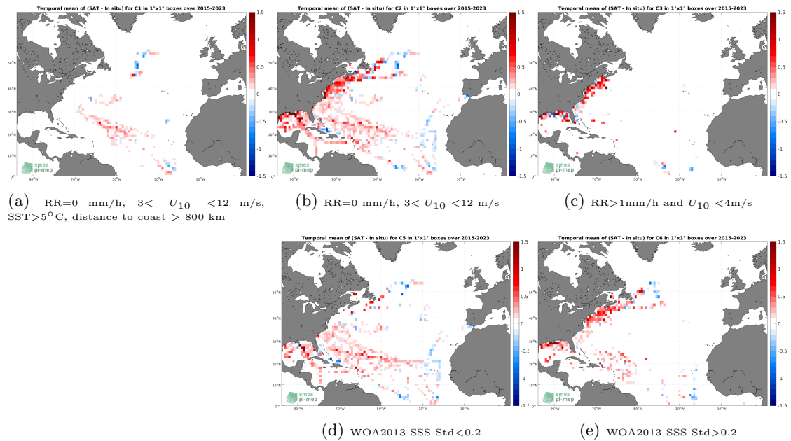
Figure 12: Temporal mean gridded over spatial boxes of size 1^\circ \times 1^\circ of \Delta SSS (SMAP SSS L3 v5 - 8-Day running (RSS) - TSG (SAMOS)) for 5 different subdatasets corresponding to:RR=0 mm/h, 3 < U_{10} < 12 m/s, SST >5^\circ C, distance to coast > 800 km (a), RR=0 mm/h, 3 < U_{10} < 12 m/s (b), RR >1 mm/h and U_{10} < 4 m/s (c), WOA2013 SSS Std <0.2 (d), WOA2013 SSS Std >0.2 (e).
