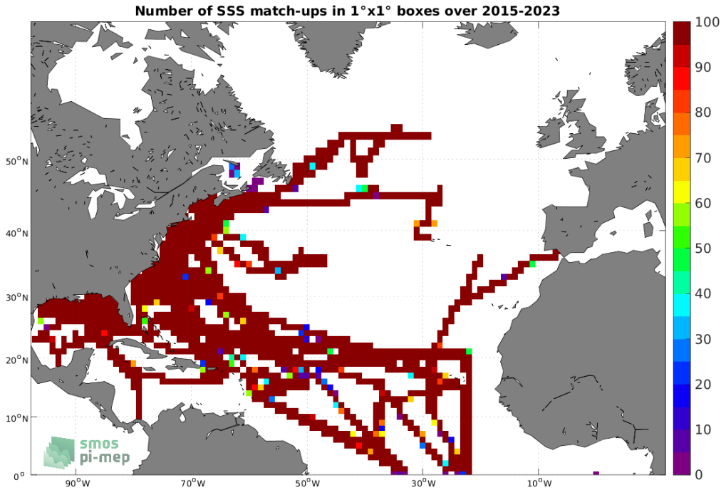
Figure 4: Number of SSS match-ups between TSG (SAMOS) SSS and the SMAP SSS L3 v5 - 8-Day running (RSS) SSS product for the North Atlantic Ocean Pi-MEP region over 1^\circ \times 1^\circ boxes and for the full satellite product period.
