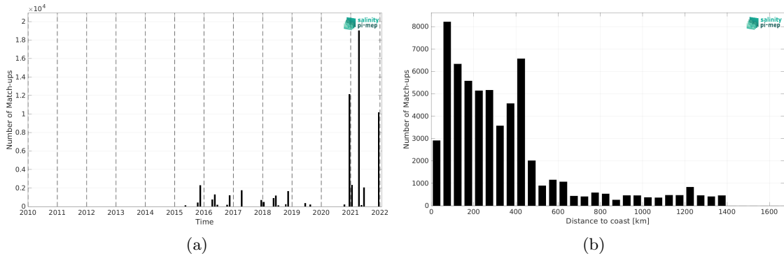
Figure 1: Number of match-ups between TSG (Polarstern) and SMAP SSS L3 v5 - 8-Day running (RSS) SSS as a function of time (a) and as function of the distance to coast (b) over the North Atlantic Ocean Pi-MEP region and for the full satellite product period.
