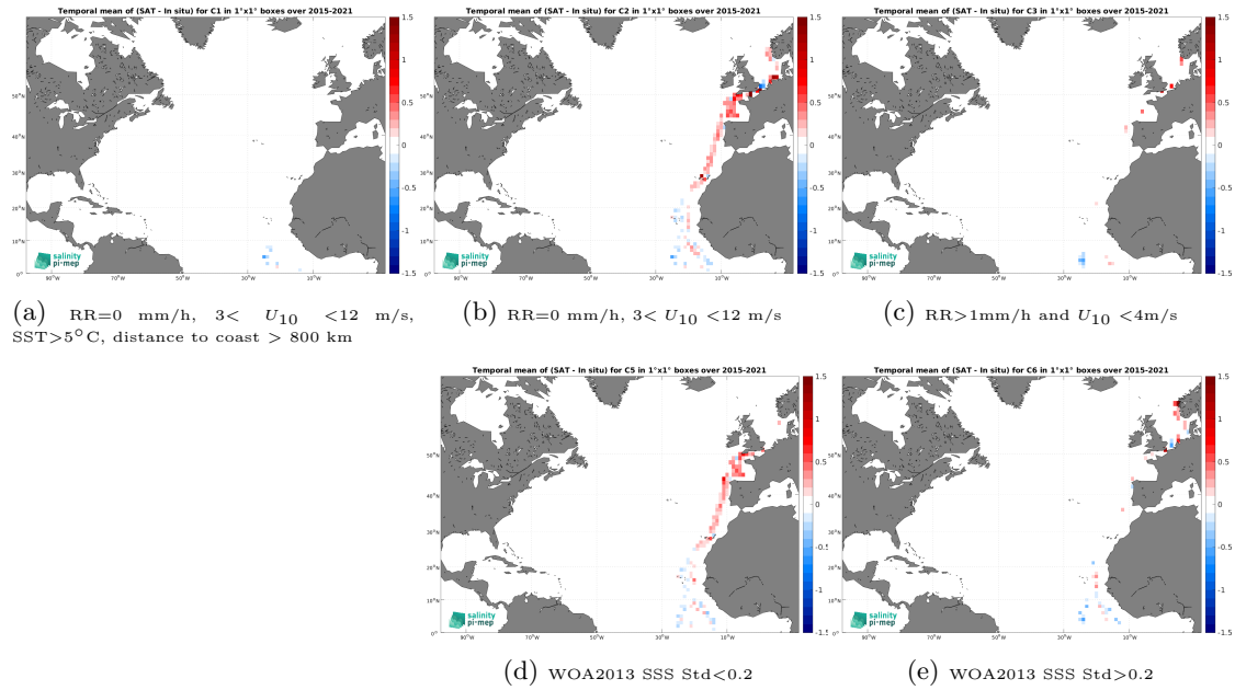
Figure 12: Temporal mean gridded over spatial boxes of size 1^\circ \times 1^\circ of \Delta\text{SSS} (SMAP SSS L3 v5 - 8-Day running (RSS) - TSG (Polarstern)) for 5 different subdatasets corresponding to:RR=0 mm/h, 3 < U_{10} < 12 m/s, SST >5^\circ\text{C} , distance to coast > 800 km (a), RR=0 mm/h, 3 < U_{10} < 12 m/s (b), RR >1 mm/h and U_{10} < 4 m/s (c), WOA2013 SSS Std <0.2 (d), WOA2013 SSS Std >0.2 (e).
