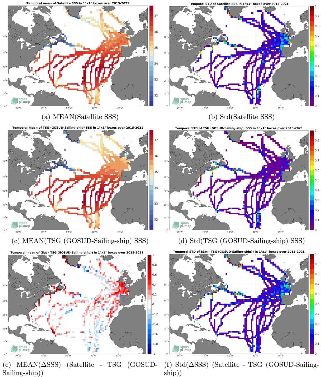
Figure 6: Temporal mean (left) and Std (right) of SSS from SMAP SSS L3 v5 - 8-Day running (RSS) (top), TSG (GOSUD-Sailing-ship) (middle), and of \Delta SSS (Satellite - TSG (GOSUD-Sailing-ship)). Only match-up pairs are used to generate these maps.
