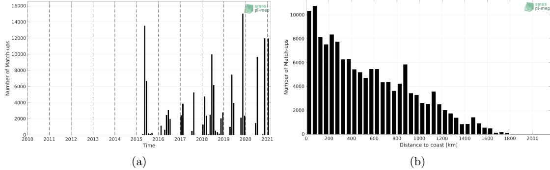
Figure 1: Number of match-ups between TSG (GOSUD-Sailing-ship) and SMAP SSS L3 v5 - 8-Day running (RSS) SSS as a function of time (a) and as function of the distance to coast (b) over the North Atlantic Ocean Pi-MEP region and for the full satellite product period.
