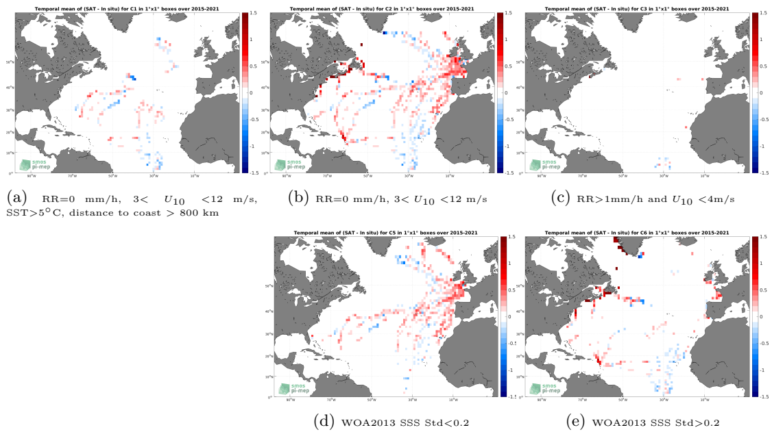
Figure 12: Temporal mean gridded over spatial boxes of size 1^\circ \times 1^\circ of \Delta\text{SSS} (SMAP SSS L3 v5 - 8-Day running (RSS) - TSG (GOSUD-Sailing-ship)) for 5 different subdatasets corresponding to:RR=0 mm/h, 3 < U_{10} < 12 m/s, SST > 5°C, distance to coast > 800 km (a), RR=0 mm/h, 3 < U_{10} < 12 m/s (b), RR > 1mm/h and U_{10} < 4 m/s (c), WOA2013 SSS Std < 0.2 (d), WOA2013 SSS Std > 0.2 (e).
