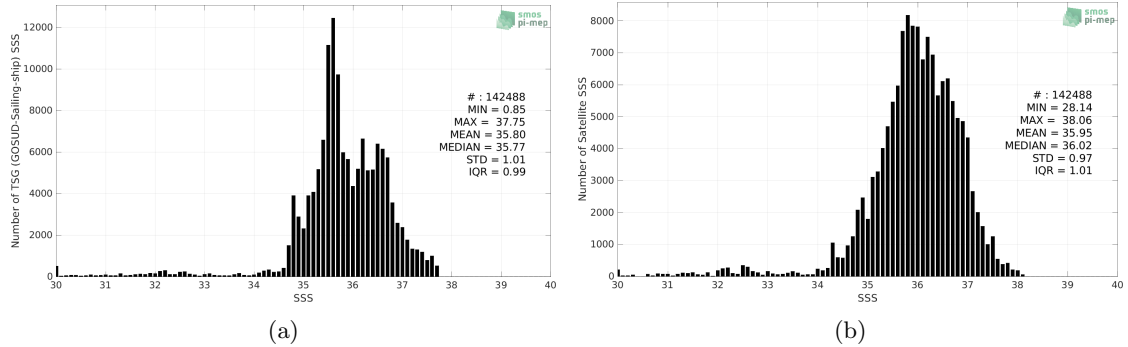
Figure 2: Histograms of SSS from TSG (GOSUD-Sailing-ship) (a) and SMAP SSS L3 v5 - 8-Day running (RSS) (b) considering all match-up pairs per bins of 0.1 over the North Atlantic Ocean Pi-MEP region and for the full satellite product period.
