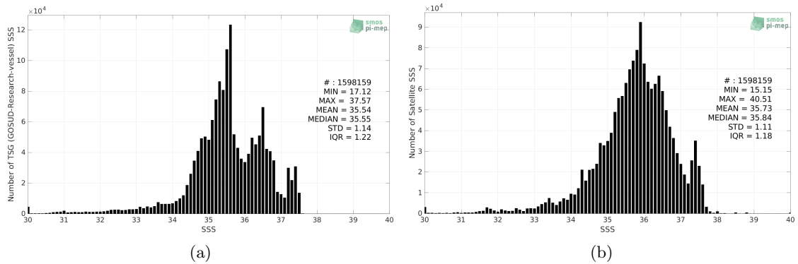
Figure 2: Histograms of SSS from TSG (GOSUD-Research-vessel) (a) and SMAP SSS L3 v5 - 8-Day running (RSS) (b) considering all match-up pairs per bins of 0.1 over the North Atlantic Ocean Pi-MEP region and for the full satellite product period.
