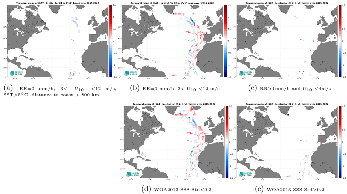
Figure 12: Temporal mean gridded over spatial boxes of size 1^\circ \times 1^\circ of \Delta\text{SSS} (SMAP SSS L3 v5 - 8-Day running (RSS) - TSG (CSIC-UTM)) for 5 different subdatasets corresponding to:RR=0 mm/h, 3 < U_{10} < 12 m/s, SST >5^\circ\text{C} , distance to coast > 800 km (a), RR=0 mm/h, 3 < U_{10} < 12 m/s (b), RR >1 mm/h and U_{10} < 4 m/s (c), WOA2013 SSS Std <0.2 (d), WOA2013 SSS Std >0.2 (e).
