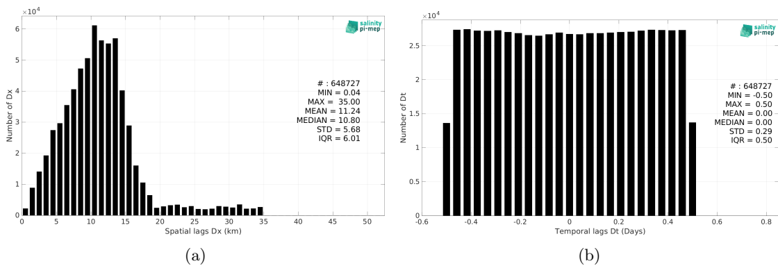
Figure 5: Histograms of the spatial (a) and temporal (b) lags between the location/time of the TSG (CSIC-UTM) measurement and the date of the corresponding SMAP SSS L3 v5 - 8-Day running (RSS) SSS pixel.
