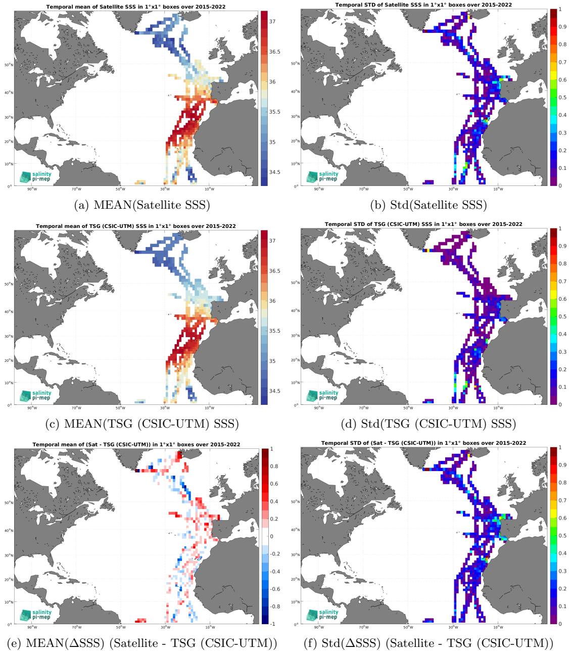
Figure 6: Temporal mean (left) and Std (right) of SSS from SMAP SSS L3 v5 - 8-Day running (RSS) (top), TSG (CSIC-UTM) (middle), and of \Delta SSS (Satellite - TSG (CSIC-UTM)). Only match-up pairs are used to generate these maps.
