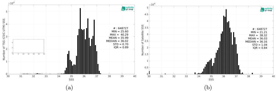
Figure 2: Histograms of SSS from TSG (CSIC-UTM) (a) and SMAP SSS L3 v5 - 8-Day running (RSS) (b) considering all match-up pairs per bins of 0.1 over the North Atlantic Ocean Pi-MEP region and for the full satellite product period.
