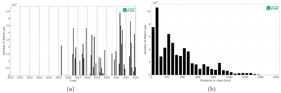
Figure 1: Number of match-ups between TSG (CSIC-UTM) and SMAP SSS L3 v5 - 8-Day running (RSS) SSS as a function of time (a) and as function of the distance to coast (b) over the North Atlantic Ocean Pi-MEP region and for the full satellite product period.
