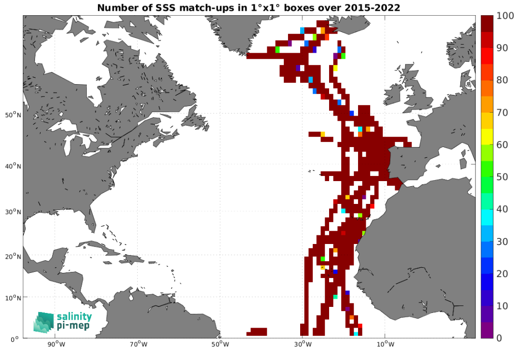
Figure 4: Number of SSS match-ups between TSG (CSIC-UTM) SSS and the SMAP SSS L3 v5 - 8-Day running (RSS) SSS product for the North Atlantic Ocean Pi-MEP region over 1^\circ \times 1^\circ boxes and for the full satellite product period.
