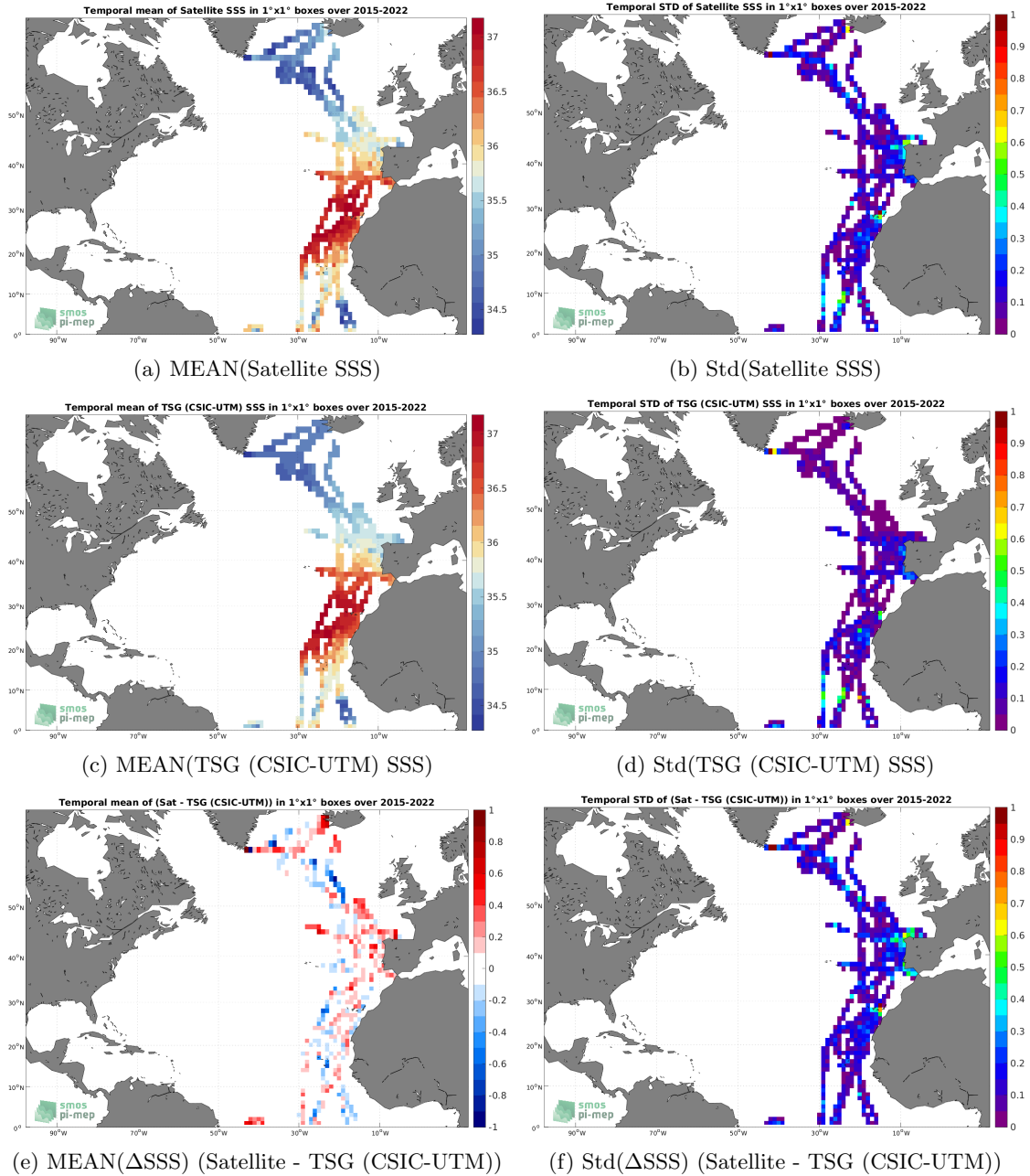
(a) MEAN(Satellite SSS) (b) Std(Satellite SSS) (c) MEAN(TSG (CSIC-UTM) SSS) (d) Std(TSG (CSIC-UTM) SSS) (e) MEAN( \Delta SSS) (Satellite - TSG (CSIC-UTM)) (f) Std( \Delta SSS) (Satellite - TSG (CSIC-UTM)) Figure 6: Temporal mean (left) and Std (right) of SSS from SMAP SSS L3 v5 - 8-Day running (RSS) (top), TSG (CSIC-UTM) (middle), and of \Delta SSS (Satellite - TSG (CSIC-UTM)). Only match-up pairs are used to generate these maps.
