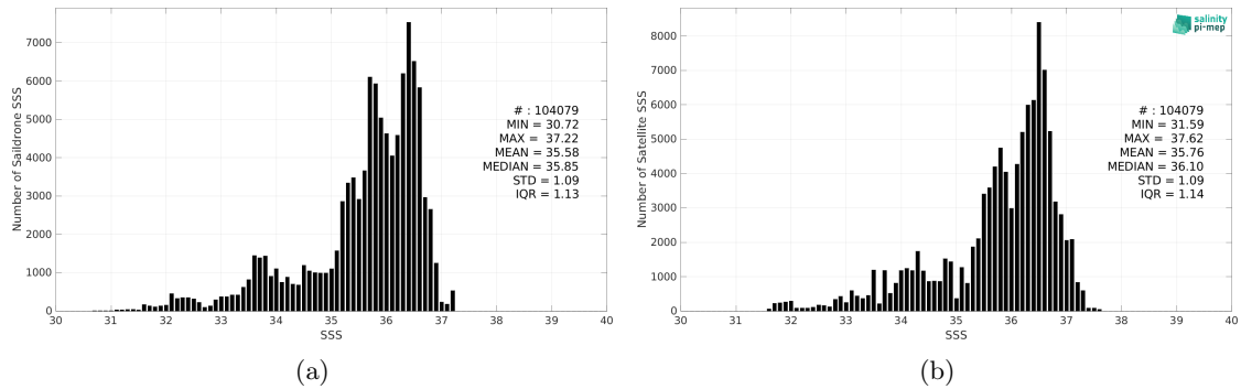
Figure 2: Histograms of SSS from Saildrone (a) and SMAP SSS L3 v5 - 8-Day running (RSS) (b) considering all match-up pairs per bins of 0.1 over the North Atlantic Ocean Pi-MEP region and for the full satellite product period.
