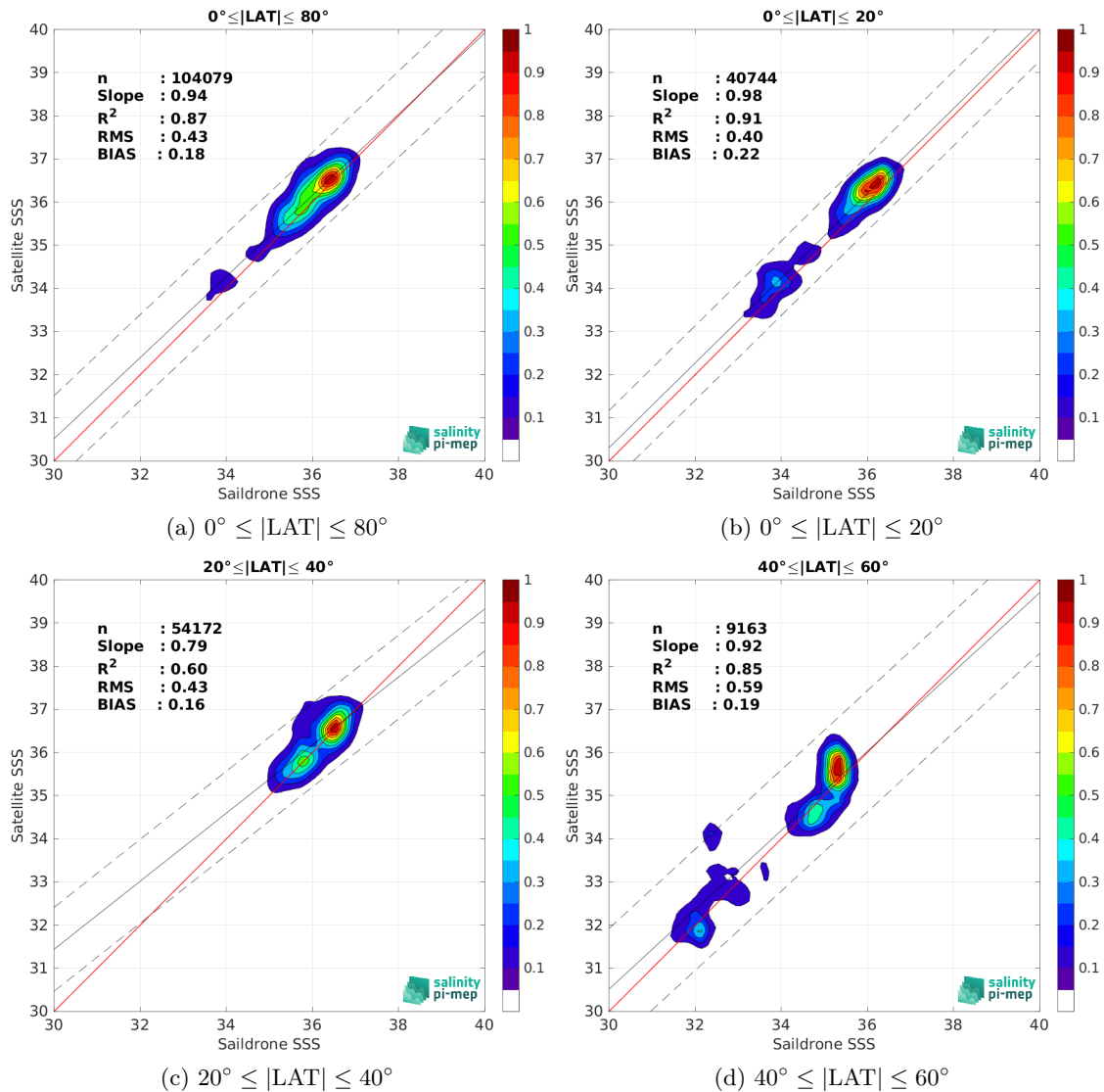
Figure 9: Contour maps of the concentration of SMAP SSS L3 v5 - 8-Day running (RSS) SSS (y-axis) versus Saildrone SSS (x-axis) at match-up pairs for different latitude bands. For each plot, the red line shows x=y . The black thin and dashed lines indicate a linear fit through the data cloud and the \pm 95\% confidence levels, respectively. The number match-up pairs n , the slope and R^2 coefficient of the linear fit, the root mean square (RMS) and the mean bias between satellite and in situ data are indicated for each latitude band in each plots.
