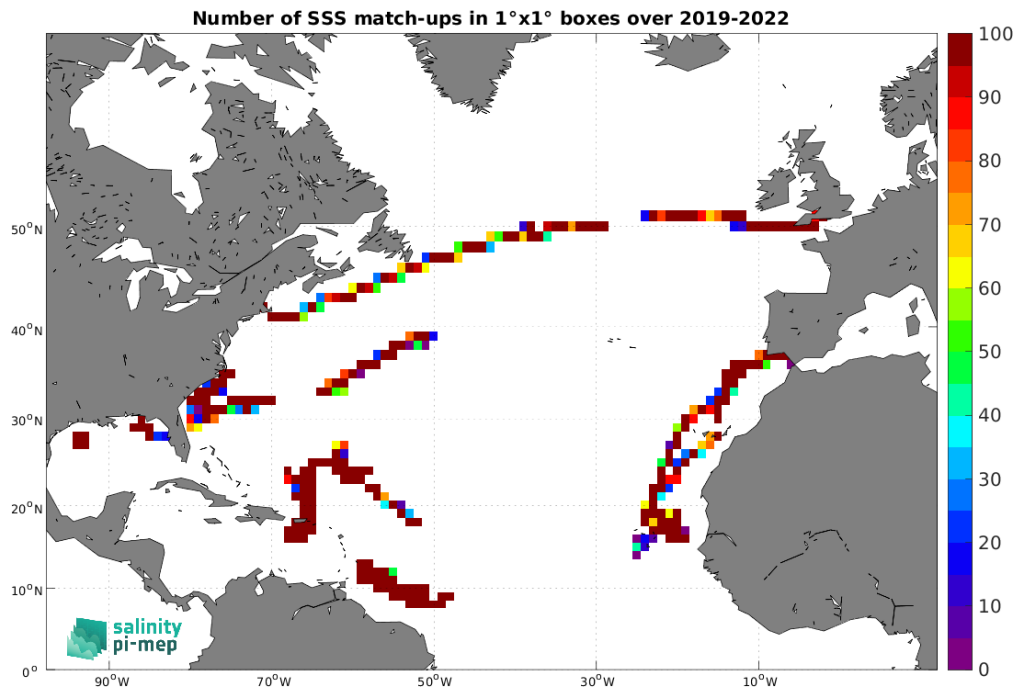
Figure 4: Number of SSS match-ups between Saildrone SSS and the SMAP SSS L3 v5 - 8-Day running (RSS) SSS product for the North Atlantic Ocean Pi-MEP region over 1^\circ \times 1^\circ boxes and for the full satellite product period.
