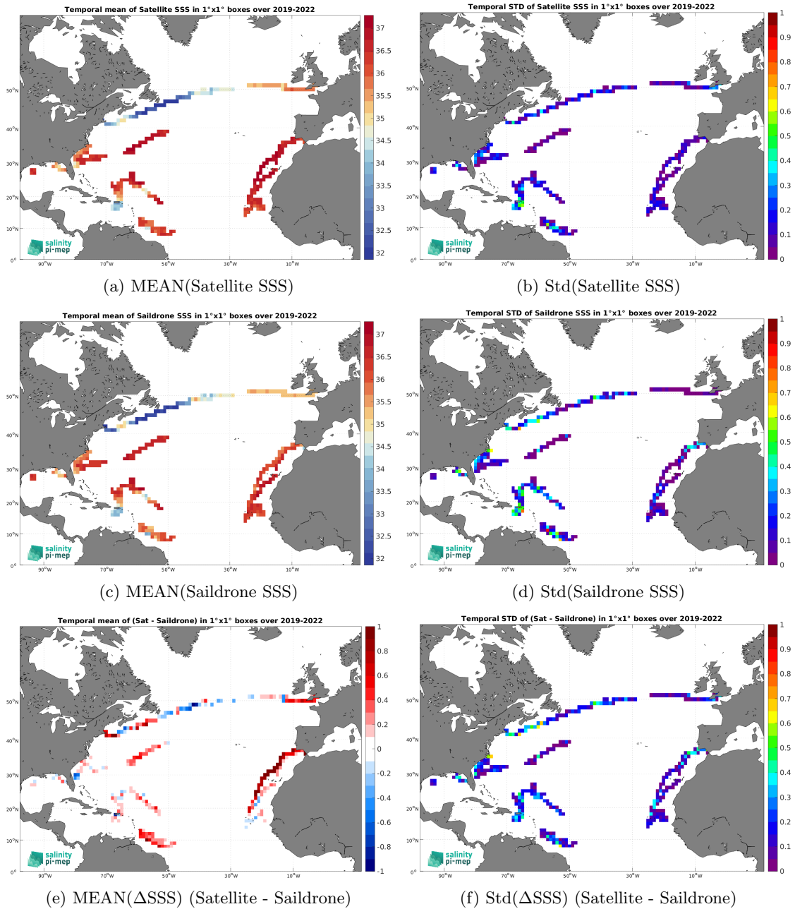
Figure 6: Temporal mean (left) and Std (right) of SSS from SMAP SSS L3 v5 - 8-Day running (RSS) (top), Saildrone (middle), and of \Delta SSS (Satellite - Saildrone). Only match-up pairs are used to generate these maps.
