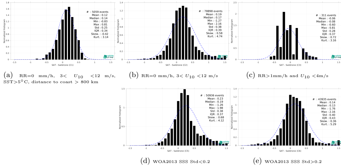
Figure 13: Normalized histogram of \Delta SSS (SMAP SSS L3 v5 - 8-Day running (RSS) - Sairdronne) for 5 different subdatasets corresponding to: RR=0 mm/h, 3 < U_{10} < 12 m/s, SST > 5°C, distance to coast > 800 km (a), RR=0 mm/h, 3 < U_{10} < 12 m/s (b), RR > 1mm/h and U_{10} < 4 m/s (c), WOA2013 SSS Std < 0.2 (d), WOA2013 SSS Std > 0.2 (e).
