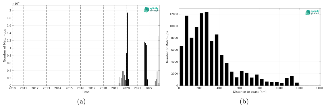
Figure 1: Number of match-ups between Saildrone and SMAP SSS L3 v5 - 8-Day running (RSS) SSS as a function of time (a) and as function of the distance to coast (b) over the North Atlantic Ocean Pi-MEP region and for the full satellite product period.
