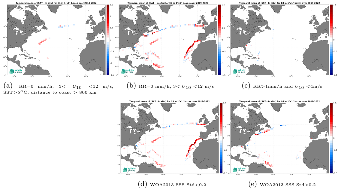
Figure 12: Temporal mean gridded over spatial boxes of size 1^\circ \times 1^\circ of \Delta\text{SSS} (SMAP SSS L3 v5 - 8-Day running (RSS) - Saikrone) for 5 different subdatasets corresponding to:RR=0 mm/h, 3 < U_{10} < 12 m/s, SST >5^\circ\text{C} , distance to coast > 800 km (a), RR=0 mm/h, 3 < U_{10} < 12 m/s (b), RR >1 mm/h and U_{10} < 4 m/s (c), WOA2013 SSS Std <0.2 (d), WOA2013 SSS Std >0.2 (e).
