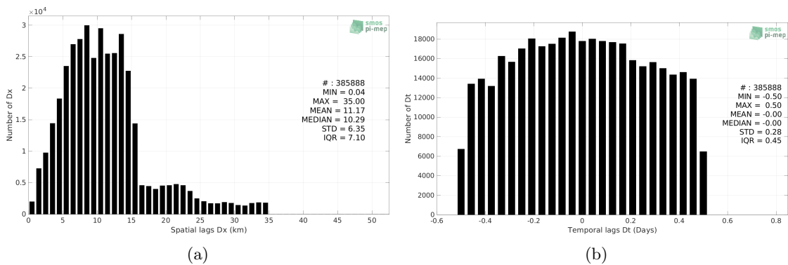
Figure 5: Histograms of the spatial (a) and temporal (b) lags between the location/time of the ICES measurement and the date of the corresponding SMAP SSS L3 v5 - 8-Day running (RSS) SSS pixel.
