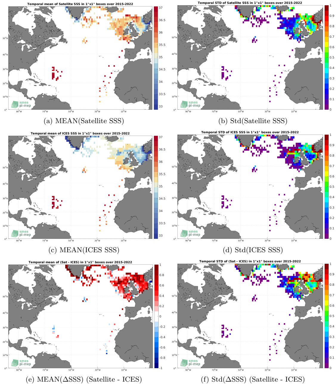
Figure 6: Temporal mean (left) and Std (right) of SSS from SMAP SSS L3 v5 - 8-Day running (RSS) (top), ICES (middle), and of \Delta SSS (Satellite - ICES). Only match-up pairs are used to generate these maps.
