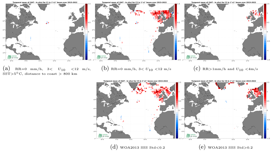
Figure 12: Temporal mean gridded over spatial boxes of size 1^\circ \times 1^\circ of \Delta\text{SSS} (SMAP SSS L3 v5 - 8-Day running (RSS) - ICES) for 5 different subdatasets corresponding to:RR=0 mm/h, 3 < U_{10} < 12 m/s, SST >5^\circ\text{C} , distance to coast > 800 km (a), RR=0 mm/h, 3 < U_{10} < 12 m/s (b), RR >1 mm/h and U_{10} < 4 m/s (c), WOA2013 SSS Std <0.2 (d), WOA2013 SSS Std >0.2 (e).
