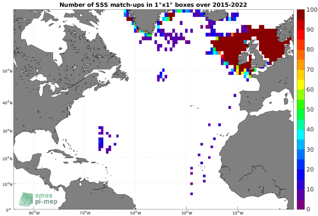
Figure 4: Number of SSS match-ups between ICES SSS and the SMAP SSS L3 v5 - 8-Day running (RSS) SSS product for the North Atlantic Ocean Pi-MEP region over 1^\circ \times 1^\circ boxes and for the full satellite product period.
