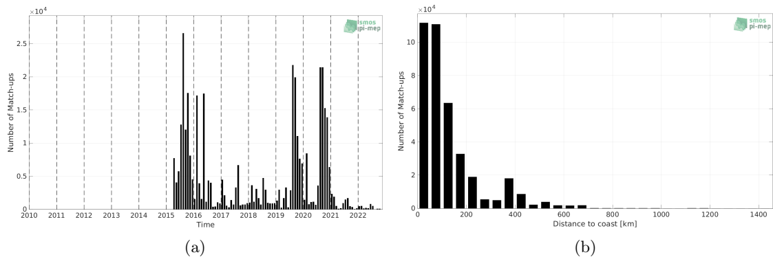
Figure 1: Number of match-ups between ICES and SMAP SSS L3 v5 - 8-Day running (RSS) SSS as a function of time (a) and as function of the distance to coast (b) over the North Atlantic Ocean Pi-MEP region and for the full satellite product period.
