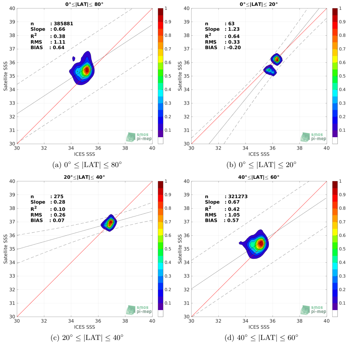
Figure 9: Contour maps of the concentration of SMAP SSS L3 v5 - 8-Day running (RSS) SSS (y-axis) versus ICES SSS (x-axis) at match-up pairs for different latitude bands. For each plot, the red line shows x=y . The black thin and dashed lines indicate a linear fit through the data cloud and the \pm 95\% confidence levels, respectively. The number match-up pairs n , the slope and R^2 coefficient of the linear fit, the root mean square (RMS) and the mean bias between satellite and in situ data are indicated for each latitude band in each plots.
