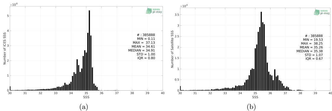
Figure 2: Histograms of SSS from ICES (a) and SMAP SSS L3 v5 - 8-Day running (RSS) (b) considering all match-up pairs per bins of 0.1 over the North Atlantic Ocean Pi-MEP region and for the full satellite product period.
