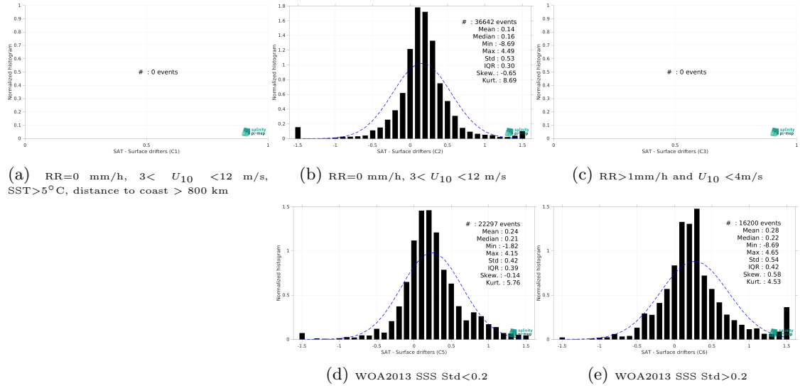
Figure 12: Normalized histogram of \Delta SSS (SMAP SSS L3 v5 - 8-Day running (RSS) - Surface drifters) for 5 different subdatasets corresponding to: RR=0 mm/h, 3 < U_{10} < 12 m/s, SST > 5°C, distance to coast > 800 km (a), RR=0 mm/h, 3 < U_{10} < 12 m/s (b), RR > 1mm/h and U_{10} < 4 m/s (c), WOA2013 SSS Std < 0.2 (d), WOA2013 SSS Std > 0.2 (e).
