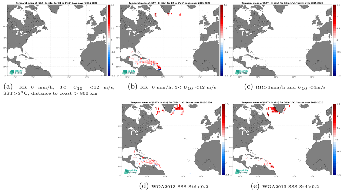
Figure 11: Temporal mean gridded over spatial boxes of size 1^\circ \times 1^\circ of \Delta SSS (SMAP SSS L3 v5 - 8-Day running (RSS) - Surface drifters) for 5 different subdatasets corresponding to:RR=0 mm/h, 3 < U_{10} < 12 m/s, SST >5^\circ\text{C} , distance to coast > 800 km (a), RR=0 mm/h, 3 < U_{10} < 12 m/s (b), RR >1 mm/h and U_{10} < 4 m/s (c), WOA2013 SSS Std <0.2 (d), WOA2013 SSS Std >0.2 (e).
