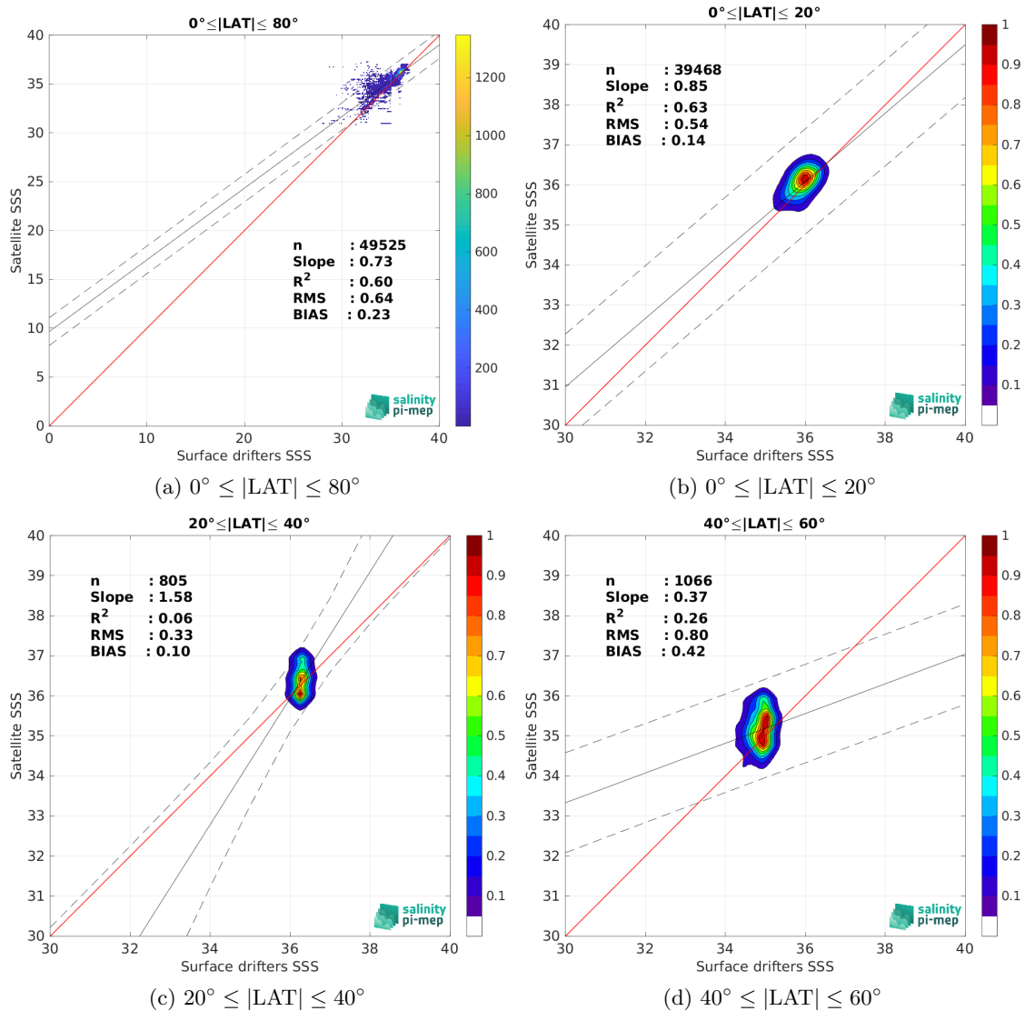
Figure 8: Contour maps of the concentration of SMAP SSS L3 v5 - 8-Day running (RSS) SSS (y-axis) versus Surface drifters SSS (x-axis) at match-up pairs for different latitude bands. For each plot, the red line shows x=y . The black thin and dashed lines indicate a linear fit through the data cloud and the \pm 95\% confidence levels, respectively. The number match-up pairs n , the slope and R^2 coefficient of the linear fit, the root mean square (RMS) and the mean bias between satellite and in situ data are indicated for each latitude band in each plots.
