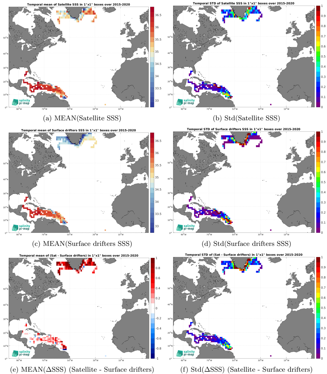
Figure 5: Temporal mean (left) and Std (right) of SSS from SMAP SSS L3 v5 - 8-Day running (RSS) (top), Surface drifters (middle), and of \Delta SSS (Satellite - Surface drifters). Only match-up pairs are used to generate these maps.
