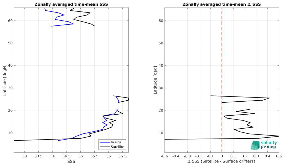
Figure 7: Left panel: Zonal mean SSS from SMAP SSS L3 v5 - 8-Day running (RSS) satellite product (black) and from Surface drifters (blue). Right panel: Zonal mean of \Delta SSS (Satellite - Surface drifters) for all the collected Pi-MEP match-up pairs estimated over the full satellite product period.
