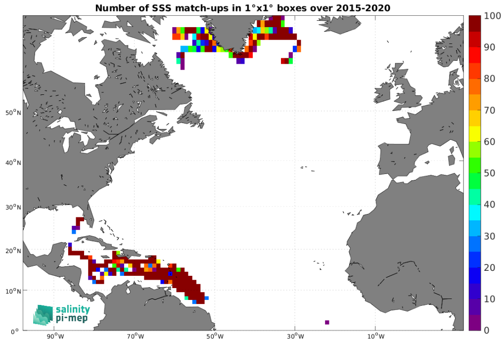
Figure 3: Number of SSS match-ups between Surface drifters SSS and the SMAP SSS L3 v5 - 8-Day running (RSS) SSS product for the North Atlantic Ocean Pi-MEP region over 1^\circ \times 1^\circ boxes and for the full satellite product period.
