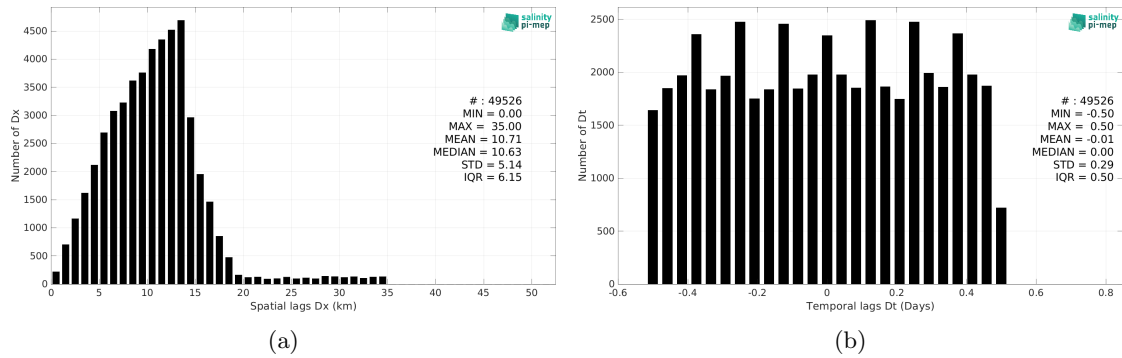
Figure 4: Histograms of the spatial (a) and temporal (b) lags between the location/time of the Surface drifters measurement and the date of the corresponding SMAP SSS L3 v5 - 8-Day running (RSS) SSS pixel.
