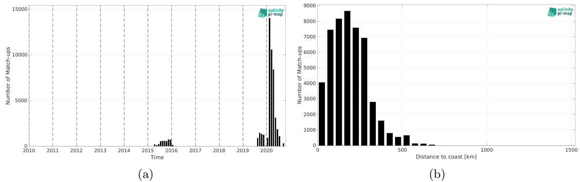
Figure 1: Number of match-ups between Surface drifters and SMAP SSS L3 v5 - 8-Day running (RSS) SSS as a function of time (a) and as function of the distance to coast (b) over the North Atlantic Ocean Pi-MEP region and for the full satellite product period.
