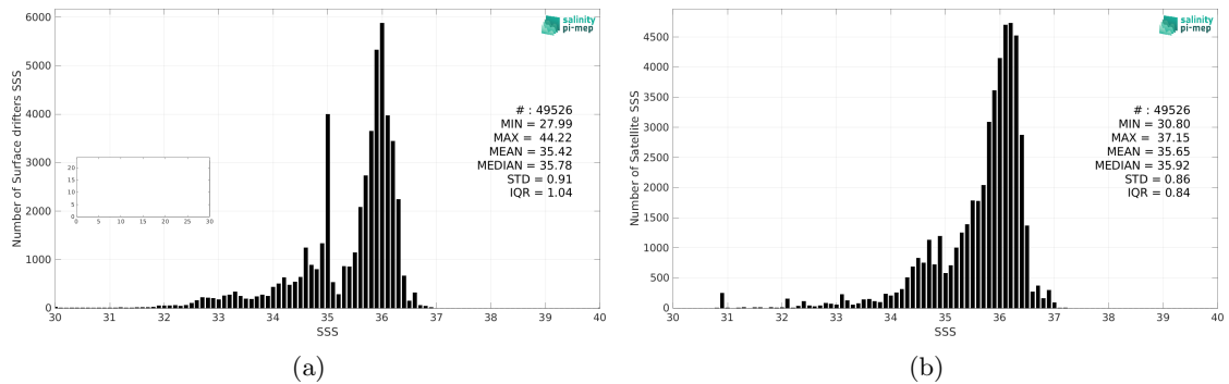
Figure 2: Histograms of SSS from Surface drifters (a) and SMAP SSS L3 v5 - 8-Day running (RSS) (b) considering all match-up pairs per bins of 0.1 over the North Atlantic Ocean Pi-MEP region and for the full satellite product period.
