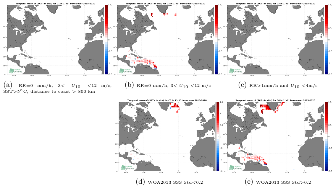
Figure 11: Temporal mean gridded over spatial boxes of size 1^\circ \times 1^\circ of \Delta\text{SSS} (SMAP SSS L3 v5 - 8-Day running (RSS) - Surface drifters) for 5 different subdatasets corresponding to:RR=0 mm/h, 3 < U_{10} < 12 m/s, SST >5^\circ\text{C} , distance to coast > 800 km (a), RR=0 mm/h, 3 < U_{10} < 12 m/s (b), RR >1 mm/h and U_{10} < 4 m/s (c), WOA2013 SSS Std <0.2 (d), WOA2013 SSS Std >0.2 (e).
