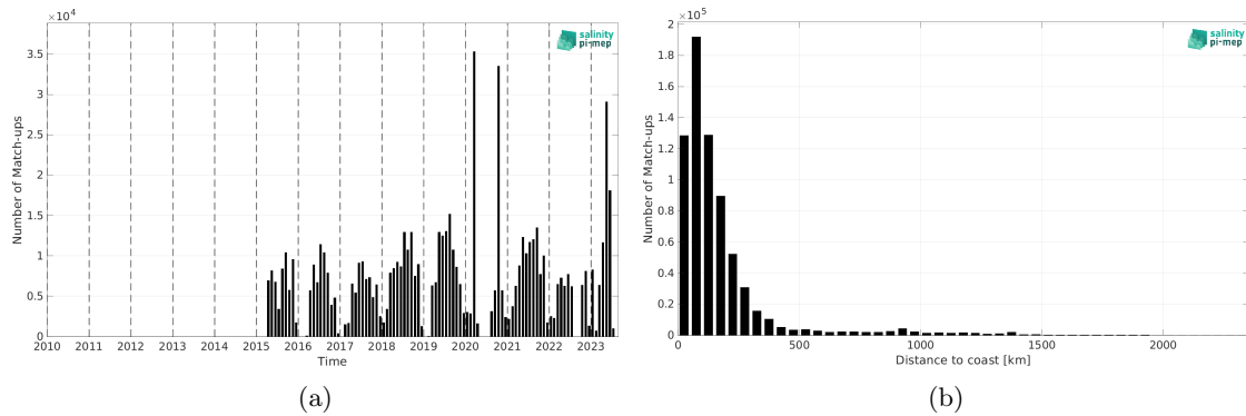
Figure 1: Number of match-ups between TSG (SAMOS) and SMAP SSS L3 v5 - Monthly (RSS) SSS as a function of time (a) and as function of the distance to coast (b) over the North Atlantic Ocean Pi-MEP region and for the full satellite product period.
