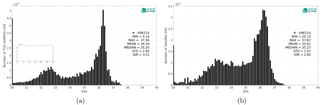
Figure 2: Histograms of SSS from TSG (SAMOS) (a) and SMAP SSS L3 v5 - Monthly (RSS) (b) considering all match-up pairs per bins of 0.1 over the North Atlantic Ocean Pi-MEP region and for the full satellite product period.
