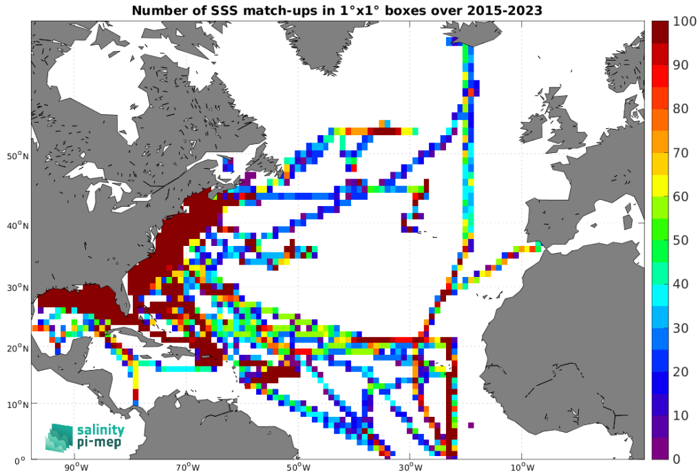
Figure 4: Number of SSS match-ups between TSG (SAMOS) SSS and the SMAP SSS L3 v5 - Monthly (RSS) SSS product for the North Atlantic Ocean Pi-MEP region over 1^\circ \times 1^\circ boxes and for the full satellite product period.
