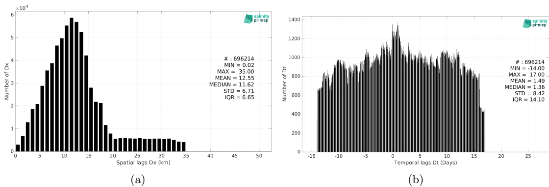
Figure 5: Histograms of the spatial (a) and temporal (b) lags between the location/time of the TSG (SAMOS) measurement and the date of the corresponding SMAP SSS L3 v5 - Monthly (RSS) SSS pixel.
