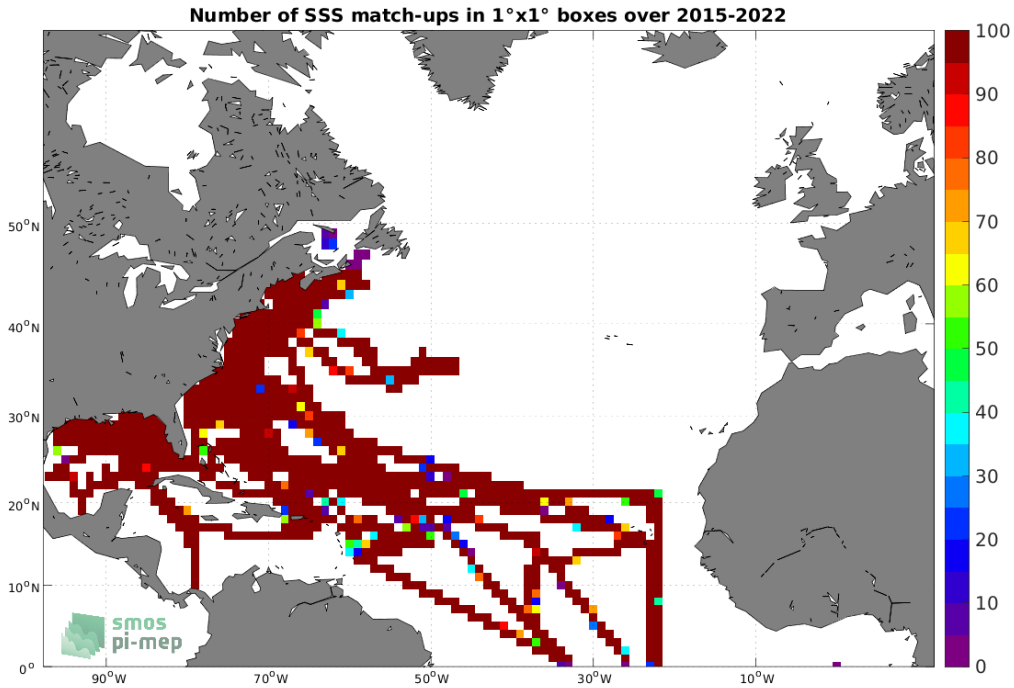
Figure 4: Number of SSS match-ups between TSG (SAMOS) SSS and the SMAP SSS L3 v5 - Monthly (RSS) SSS product for the North Atlantic Ocean Pi-MEP region over 1°×1° boxes and for the full satellite product period.
