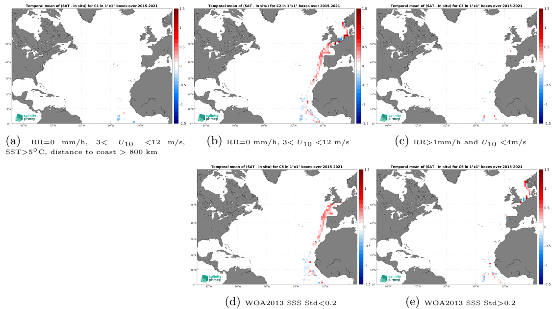
Figure 12: Temporal mean gridded over spatial boxes of size 1^\circ \times 1^\circ of \Delta\text{SSS} (SMAP SSS L3 v5 - Monthly (RSS) - TSG (Polarstern)) for 5 different subdatasets corresponding to:RR=0 mm/h, 3 < U_{10} < 12 m/s, SST >5^\circ\text{C} , distance to coast > 800 km (a), RR=0 mm/h, 3 < U_{10} < 12 m/s (b), RR >1 mm/h and U_{10} < 4 m/s (c), WOA2013 SSS Std <0.2 (d), WOA2013 SSS Std >0.2 (e).
