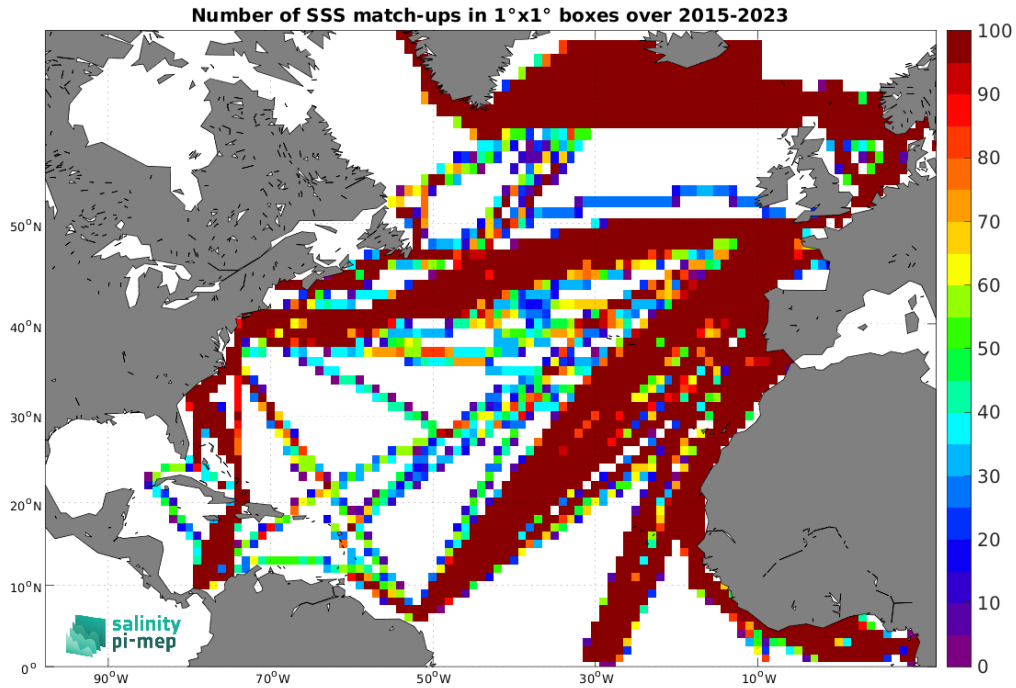
Figure 4: Number of SSS match-ups between TSG (LEGOS-DM) SSS and the SMAP SSS L3 v5 - Monthly (RSS) SSS product for the North Atlantic Ocean Pi-MEP region over 1°x1° boxes and for the full satellite product period.
