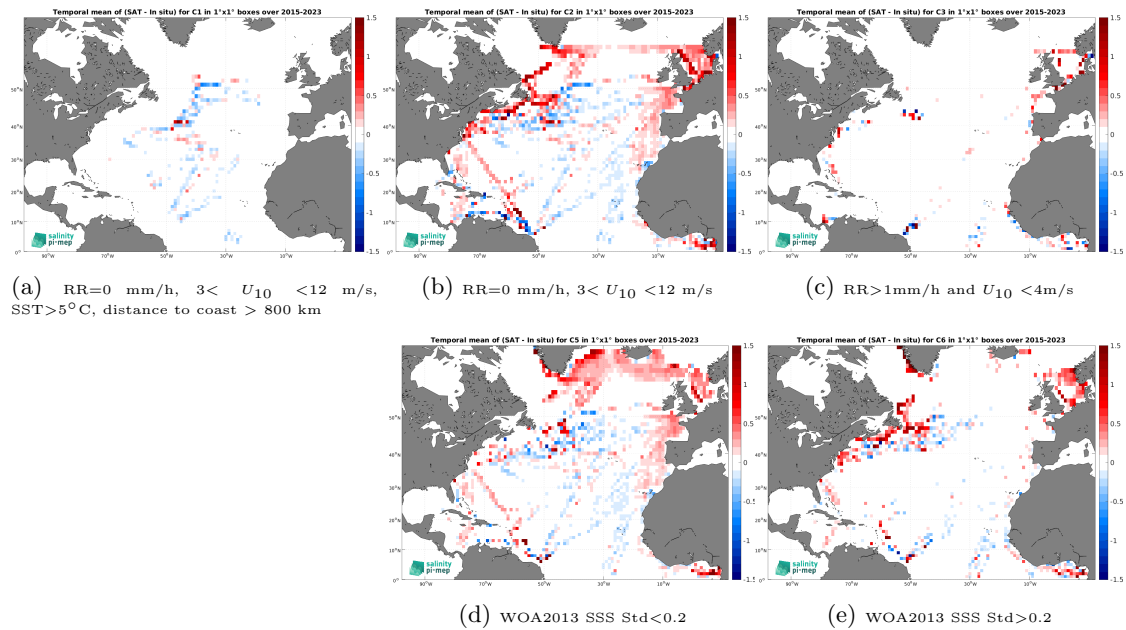
Figure 12: Temporal mean gridded over spatial boxes of size 1^\circ \times 1^\circ of \Delta\text{SSS} (SMAP SSS L3 v5 - Monthly (RSS) - TSG (LEGOS-DM)) for 5 different subdatasets corresponding to:RR=0 mm/h, 3 < U_{10} < 12 m/s, SST > 5^\circ\text{C} , distance to coast > 800 km (a), RR=0 mm/h, 3 < U_{10} < 12 m/s (b), RR > 1 mm/h and U_{10} < 4 m/s (c), WOA2013 SSS Std < 0.2 (d), WOA2013 SSS Std > 0.2 (e).
