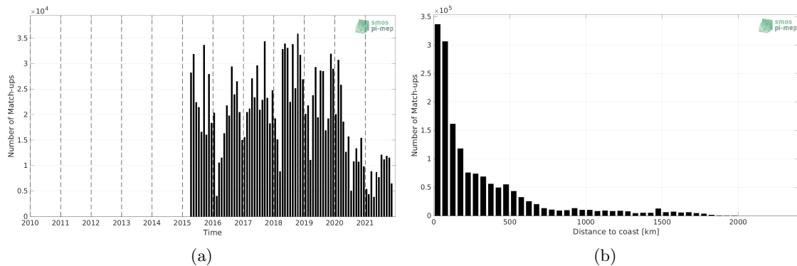
Figure 1: Number of match-ups between TSG (LEGOS-DM) and SMAP SSS L3 v5 - Monthly (RSS) SSS as a function of time (a) and as function of the distance to coast (b) over the North Atlantic Ocean Pi-MEP region and for the full satellite product period.
