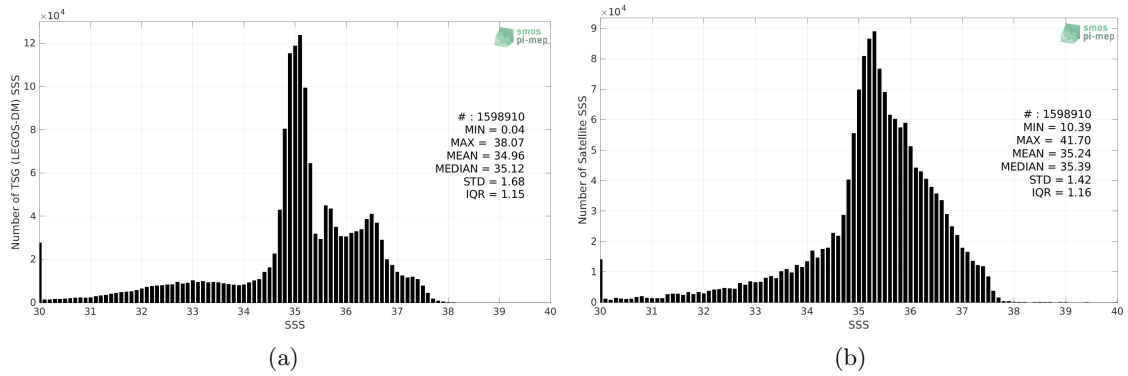
Figure 2: Histograms of SSS from TSG (LEGOS-DM) (a) and SMAP SSS L3 v5 - Monthly (RSS) (b) considering all match-up pairs per bins of 0.1 over the North Atlantic Ocean Pi-MEP region and for the full satellite product period.
