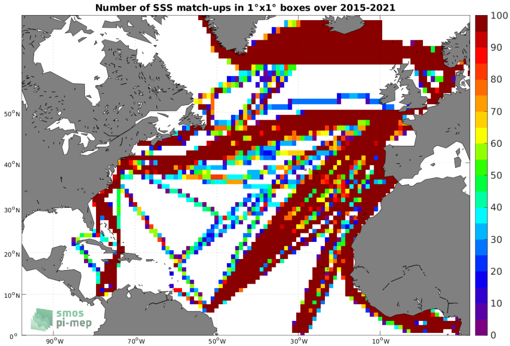
Figure 4: Number of SSS match-ups between TSG (LEGOS-DM) SSS and the SMAP SSS L3 v5 - Monthly (RSS) SSS product for the North Atlantic Ocean Pi-MEP region over 1^\circ \times 1^\circ boxes and for the full satellite product period.
