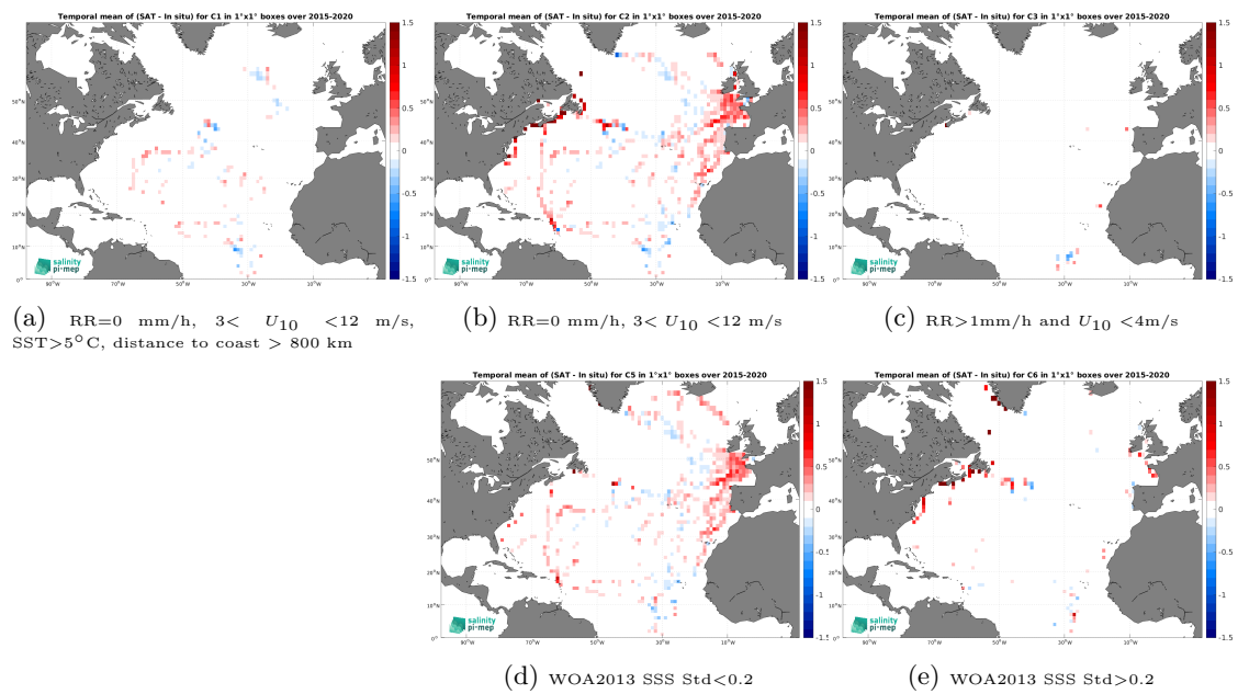
Figure 12: Temporal mean gridded over spatial boxes of size 1^\circ \times 1^\circ of \Delta\text{SSS} (SMAP SSS L3 v5 - Monthly (RSS) - TSG (GOSUD-Sailing-ship)) for 5 different subdatasets corresponding to:RR=0 mm/h, 3 < U_{10} < 12 m/s, SST >5^\circ\text{C} , distance to coast > 800 km (a), RR=0 mm/h, 3 < U_{10} < 12 m/s (b), RR >1 mm/h and U_{10} < 4 m/s (c), WOA2013 SSS Std <0.2 (d), WOA2013 SSS Std >0.2 (e).
