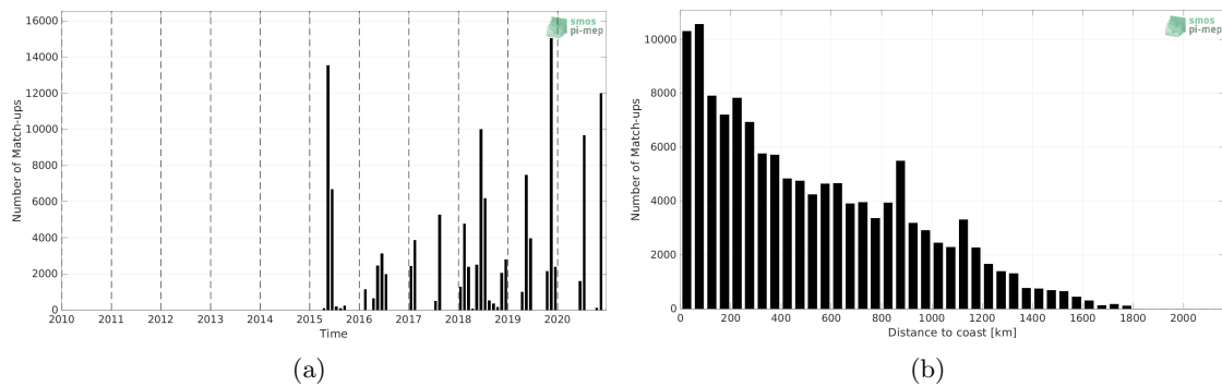
Figure 1: Number of match-ups between TSG (GOSUD-Sailing-ship) and SMAP SSS L3 v5 - Monthly (RSS) SSS as a function of time (a) and as function of the distance to coast (b) over the North Atlantic Ocean Pi-MEP region and for the full satellite product period.
