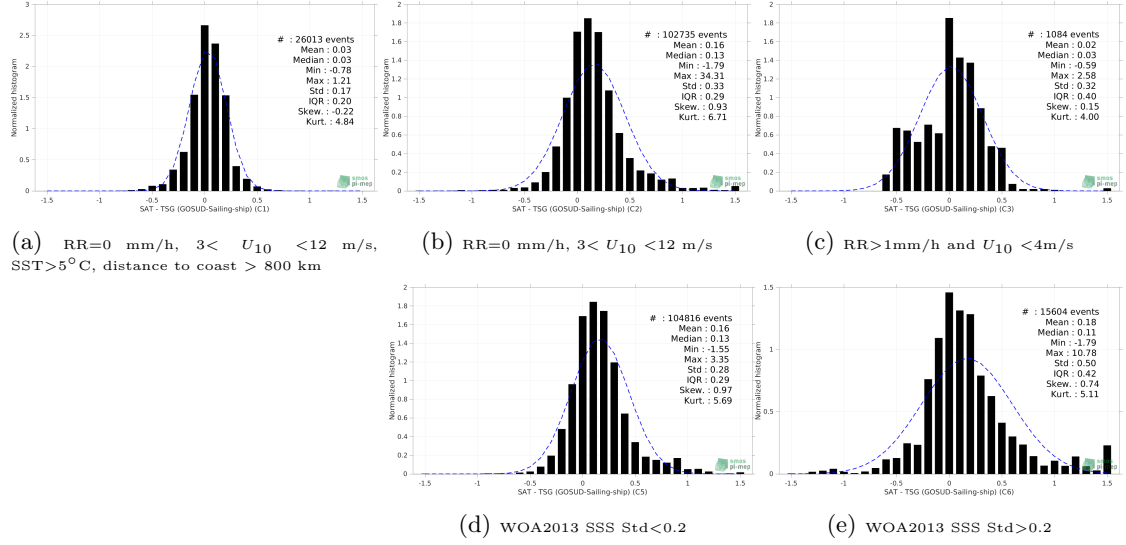
Figure 13: Normalized histogram of \Delta SSS (SMAP SSS L3 v5 - Monthly (RSS) - TSG (GOSUD-Sailing-ship)) for 5 different subdatasets corresponding to: RR=0 mm/h, 3 < U_{10} < 12 m/s, SST > 5°C, distance to coast > 800 km (a), RR=0 mm/h, 3 < U_{10} < 12 m/s (b), RR > 1mm/h and U_{10} < 4 m/s (c), WOA2013 SSS Std < 0.2 (d), WOA2013 SSS Std > 0.2 (e).
