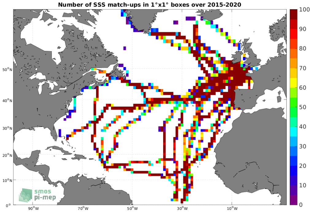
Figure 4: Number of SSS match-ups between TSG (GOSUD-Sailing-ship) SSS and the SMAP SSS L3 v5 - Monthly (RSS) SSS product for the North Atlantic Ocean Pi-MEP region over 1^\circ \times 1^\circ boxes and for the full satellite product period.
