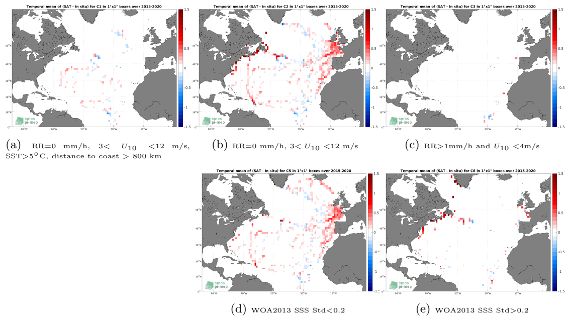
Figure 12: Temporal mean gridded over spatial boxes of size 1^\circ \times 1^\circ of \Delta SSS (SMAP SSS L3 v5 - Monthly (RSS) - TSG (GOSUD-Sailing-ship)) for 5 different subdatasets corresponding to:RR=0 mm/h, 3 < U_{10} < 12 m/s, SST>5°C, distance to coast > 800 km (a), RR=0 mm/h, 3 < U_{10} < 12 m/s (b), RR>1mm/h and U_{10} < 4 m/s (c), WOA2013 SSS Std<0.2 (d), WOA2013 SSS Std>0.2 (e).
