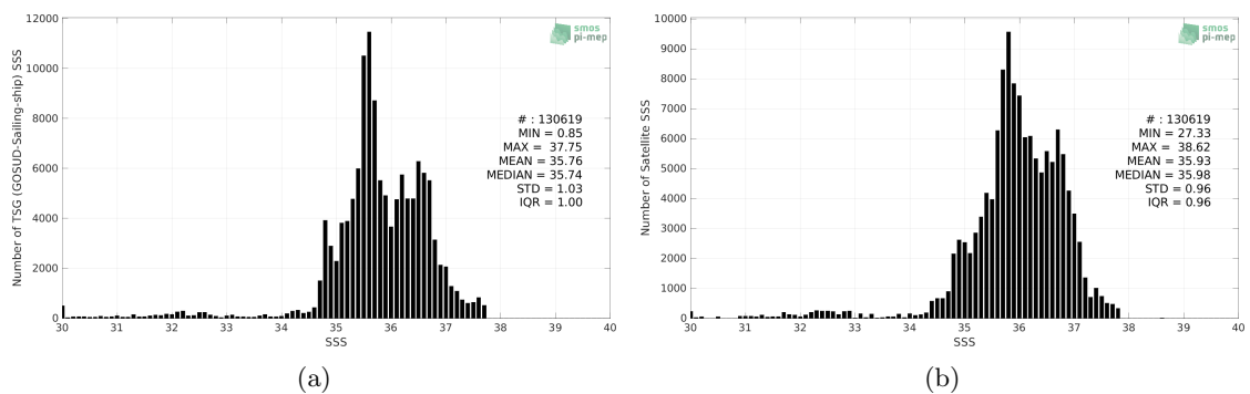
Figure 2: Histograms of SSS from TSG (GOSUD-Sailing-ship) (a) and SMAP SSS L3 v5 - Monthly (RSS) (b) considering all match-up pairs per bins of 0.1 over the North Atlantic Ocean Pi-MEP region and for the full satellite product period.
