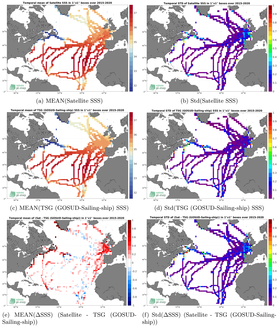
Figure 6: Temporal mean (left) and Std (right) of SSS from SMAP SSS L3 v5 - Monthly (RSS) (top), TSG (GOSUD-Sailing-ship) (middle), and of \Delta SSS (Satellite - TSG (GOSUD-Sailing-ship)). Only match-up pairs are used to generate these maps.
