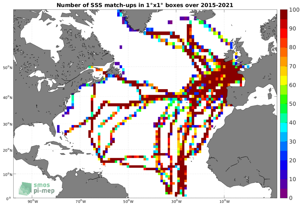
Figure 4: Number of SSS match-ups between TSG (GOSUD-Sailing-ship) SSS and the SMAP SSS L3 v5 - Monthly (RSS) SSS product for the North Atlantic Ocean Pi-MEP region over 1°x1° boxes and for the full satellite product period.
