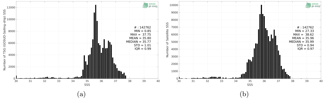
Figure 2: Histograms of SSS from TSG (GOSUD-Sailing-ship) (a) and SMAP SSS L3 v5 - Monthly (RSS) (b) considering all match-up pairs per bins of 0.1 over the North Atlantic Ocean Pi-MEP region and for the full satellite product period.
